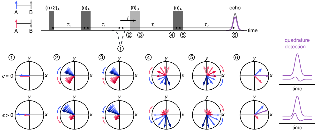
Figure 2. Vector model of the spin movement along the 4-pulse DEER sequence. Cases of low and high polarization values are shown where the numbers indicate the vector picture at a given point in time during the pulse sequence. The vectors indicate the two sub-populations of A-spins where those next to up-B-spins are colored blue and those next to down-B-spins are pink. The length of the arrows indicates the population. The overall magnetization is a sum of the two sub-populations, shown in purple. The respective echoes for low and high spin polarization values are shown on the right.
