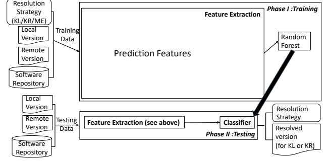
Figure 2: RPREDICTOR has two phases: training and testing
