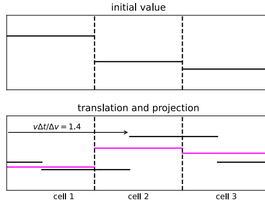
Fig. 1. Illustration of the semi-Lagrangian discontinuous Galerkin scheme (note that for the first scheme described here we have a constant, i.e., a polynomial of degree 0, in each cell).
