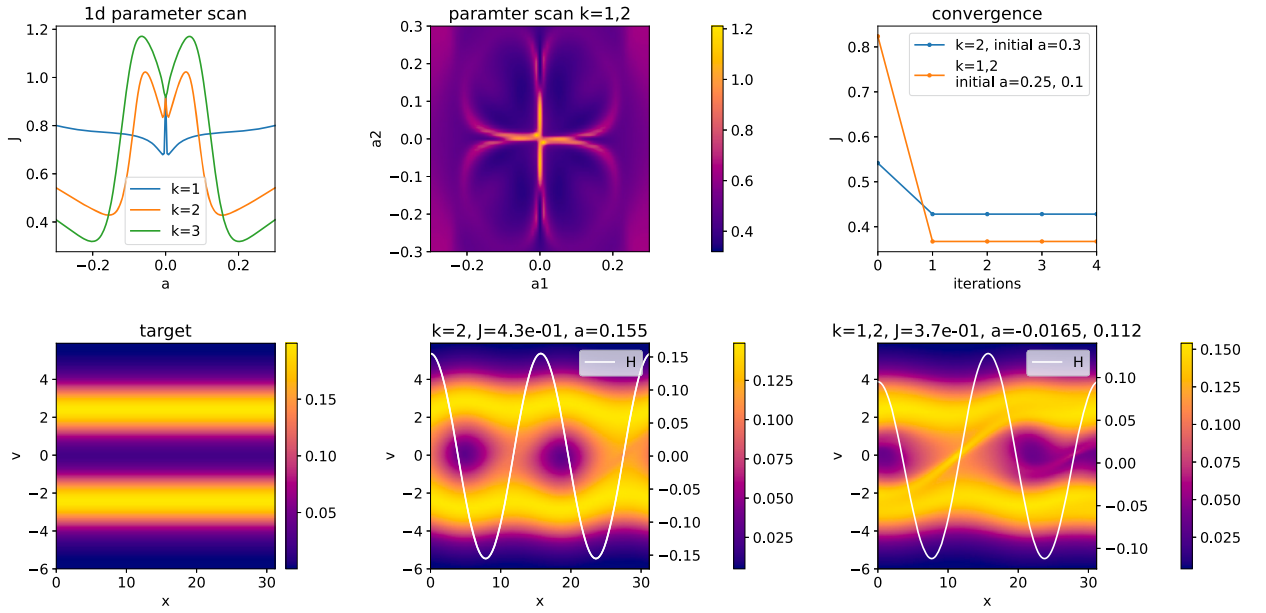
Fig. 9. A one-dimensional parameter scan for K = \{1\} , K = \{2\} , and K = \{3\} is shown on the top left and a two-dimensional parameter scan for K = \{1,2\} is shown on the top middle. The convergence of Algorithm 3 for two different initial guesses/two configurations is shown on the top right. The corresponding distribution function at time t = 40 is shown along with the target at the bottom.
