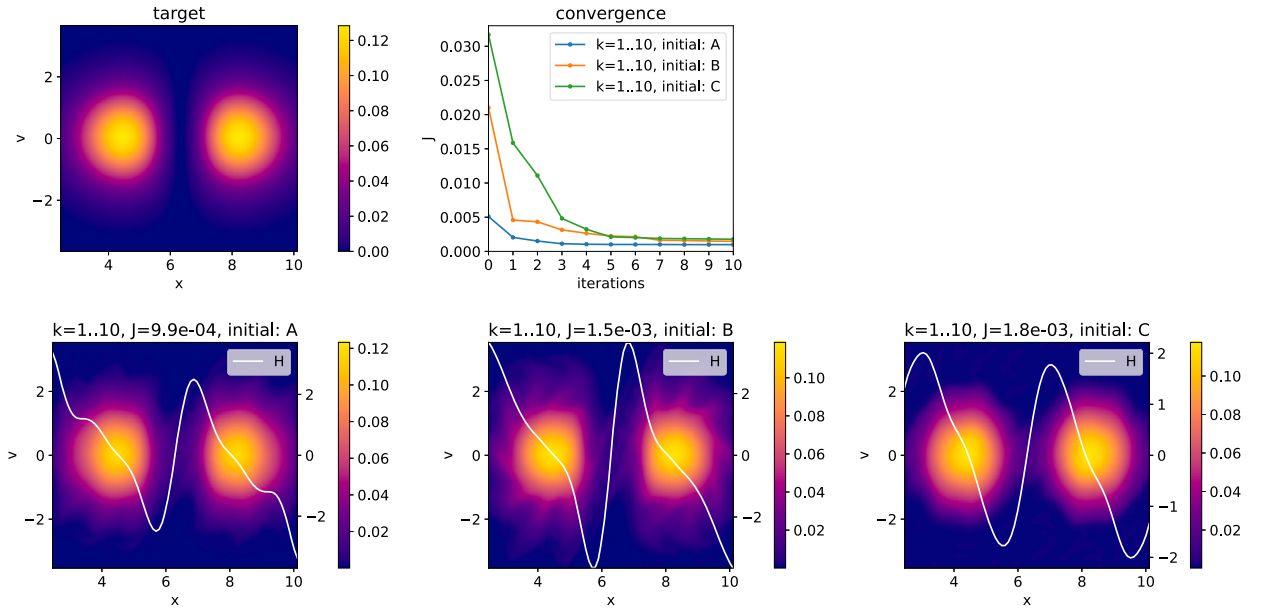
Fig. 5. We show the convergence of the optimization algorithm for three different runs with different initial guesses. The initial guesses for the three runs are listed in Table 1. Note that we have restricted both the x and v axes in the plots of the distribution function in order to make the comparison easier.
