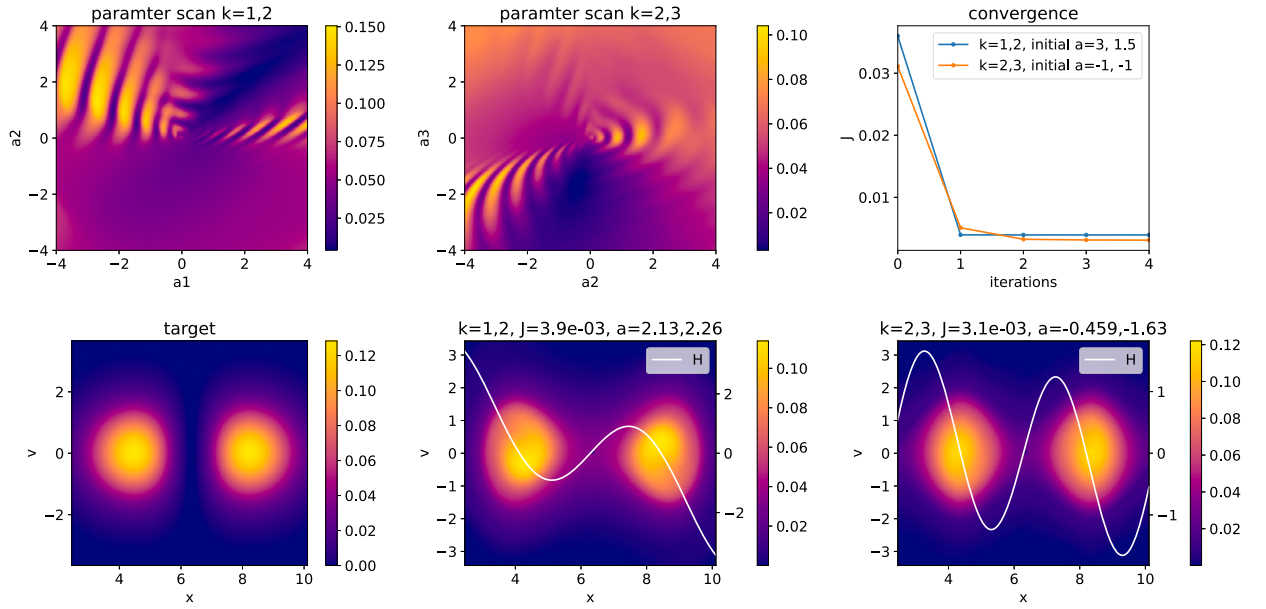
Fig. 4. A parameter scan for K = \{1, 2\} and K = \{2, 3\} is shown on the top. The convergence of the optimization algorithm for two different initial values is shown on the top right and the corresponding distribution function at time t = 20 is shown at the bottom. Note that we have restricted both the x and v axis in the plots of the distribution function in order to make the comparison easier.
