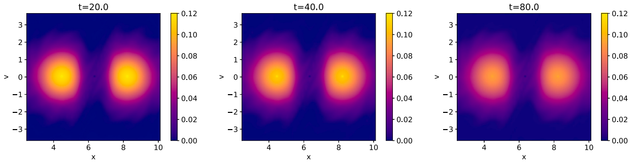
Fig. 7. The parameter found in the genetic algorithm with gradient-polishing that achieves J = 7.2 \cdot 10^{-4} at t = 20 is applied as the external field to the VP system, which is then ran to t = 40 and t = 80 . The plasma particles start to leak and show blurring compared to the target distribution, but the beam shape is relatively preserved well. Note that we have restricted both the x and v axes in the plots of the distribution function in order to make the comparison easier.
