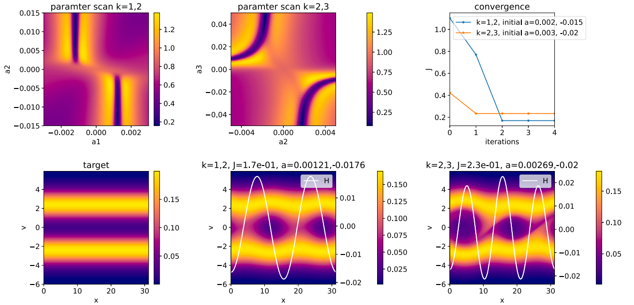
Fig. 10. A parameter scan for K = \{1,2\} and K = \{2,3\} is shown on the top. The convergence of Algorithm 3 for two different initial guesses is shown on the top right, and the corresponding distribution function at time t = 40 is shown at the bottom.
