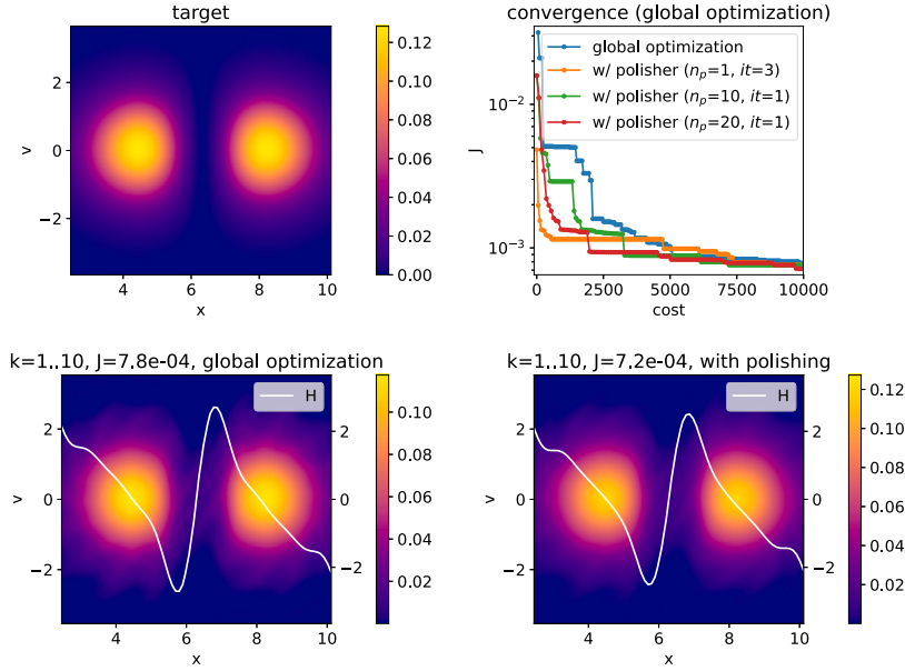
Fig. 6. The plot presents the convergence performance of the genetic optimization algorithm with gradient based polishing for different values of n_p (the number of candidate solutions in each generation that are polished) and it (the number of gradient-descent sub-iterations during the polishing). We use 50 candidate solutions in the genetic algorithm. For the computational cost we made a crude assumption that each forward and backward problem solve has a unit cost, and thus the computational cost per iteration is 50 + 2 \cdot n_p \cdot it . Including gradient-based optimization as part of a global optimization algorithm significantly reduces the computational cost. On the bottom of the plot, the distribution function for the best solutions, found with and without the gradient-based polishing algorithm, are shown. The optimization results are similar while gradient-polishing achieves the convergence with much less cost. Note that we have restricted both the x and y axes in the plots of the distribution function in order to make the comparison easier.
