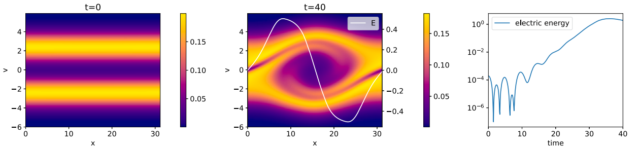
Fig. 8. Time evolution of the two-stream instability when the external field is set to be H = 0 : A small perturbation at t = 0 leads to an exponential increase of the electric energy until nonlinear effects cap it off with a saturation. The amplitude of E is marked on the right side of the plot in the middle panel.
