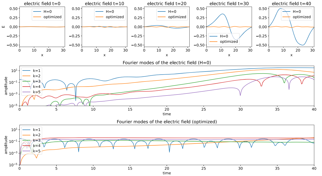
Fig. 12. Snapshots of the electric field E using H = 0 and the optimal H from results displayed in Fig. 11 are shown on the top. The plot in the second row shows the first five Fourier modes of E with H = 0 : They clearly demonstrate the exponential growth that suggests instability. The plot on the bottom shows the evolution of the electric field E when the optimal external field (found by the optimization algorithm) is applied. The external field invokes all Fourier modes to be excited but none present exponential growth. These modes nonlinearly interact, providing overall stability.
