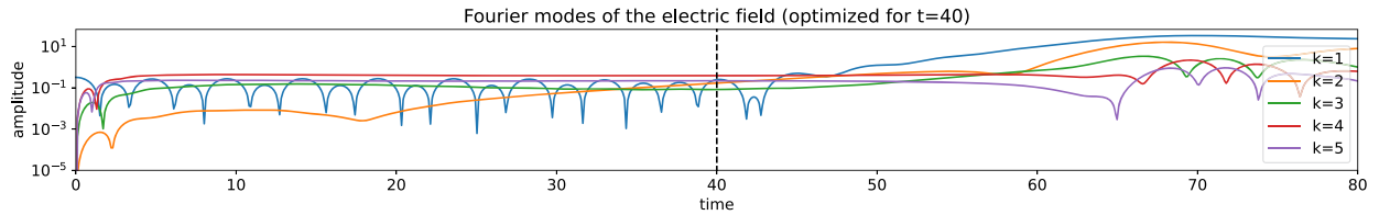
Fig. 13. The first five Fourier modes of the self-generated electric field E are shown as a function of time when the VP system is imposed by the found optimized external field H , found through running optimization up to t = 40 (as indicated by the black dashed vertical line). Over this time interval, the mixing of the modes suppresses the instability. As one continues running the VP system, in the long time horizon, the instability of the k = 1 mode manifests itself, leading to an exponential growth of the electric energy. The nonlinearity eventually kicks in, capping off the growth at saturation.
