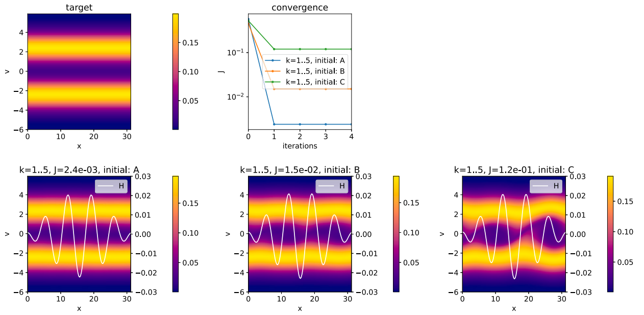
Fig. 11. Algorithm 3 is ran for K = \{1, \dots, 5\} with three different initial guesses. The convergence in iteration is shown on the top right and the obtained distribution functions at t = 40 are shown on the bottom. For initial configuration A, B and C are given in Table 2. The best obtained solution has J \approx 2.4 \cdot 10^{-3} generated by [a_1, \dots, a_5] = [0.00000591, -0.00003512, 0.00134810, -0.01075167, 0.01016702] .
