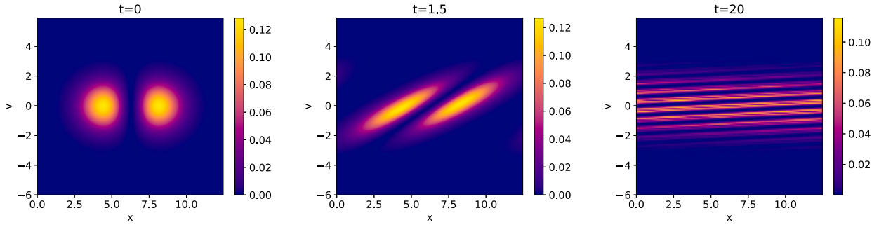
Fig. 2. The distribution function f(t, x, v) is shown at time t = 0 , t = 1.5 , and t = 20 with the external electric field set to be H = 0 (i.e., no control imposed). As expected, the beams spread out quickly forming filaments. For this simulation, 128 grid points in both the space and velocity direction and a time step size of \Delta t = 0.5 has been used. (For interpretation of the colors in the figure(s), the reader is referred to the web version of this article.)
