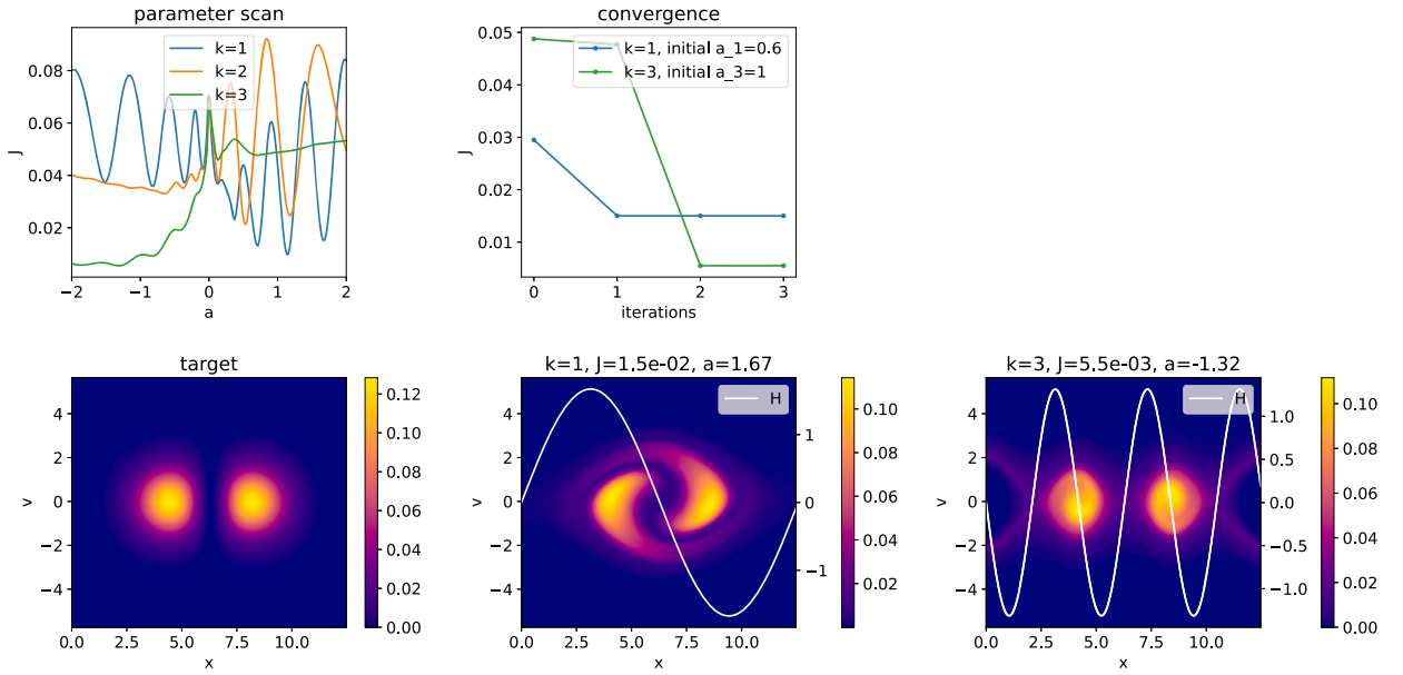
Fig. 3. The top left plot shows the parameter scan for k = 1 , k = 2 , and k = 3 . The convergence of the optimization algorithm for two runs using k = 1 and k = 3 respectively is shown on the top middle and the corresponding distribution function at time t = 20 is shown at the bottom.
