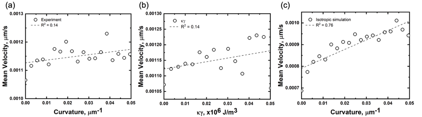
Fig. 3. Mean grain boundary velocity versus curvature for (a) experimental data. (b) Mean grain boundary velocity versus the product of energy and curvature ( \kappa\gamma ). (c) Mean grain boundary velocity versus curvature for isotropic simulation. The dashed lines are linear fits that serve as guides to the eye. In each case, the standard deviations are large (not shown) but have roughly the same value at each point and average to 9.3 \times 10^{-4} \mu\text{m/s} , 9.2 \times 10^{-4} \mu\text{m/s} , and 7.2 \times 10^{-4} \mu\text{m/s} in (a), (b), and (c), respectively.
