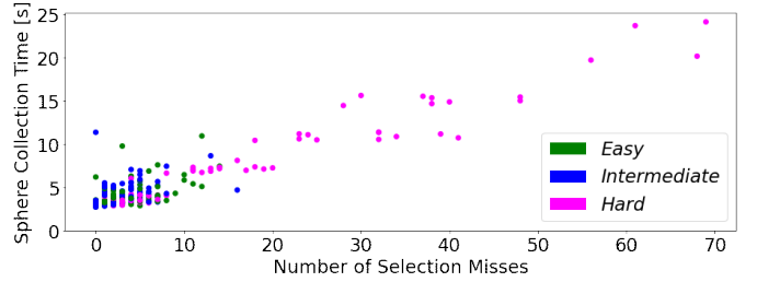
Fig. 11: The time needed to collect a sphere as a function of the number of selection misses, and of the sphere type.
