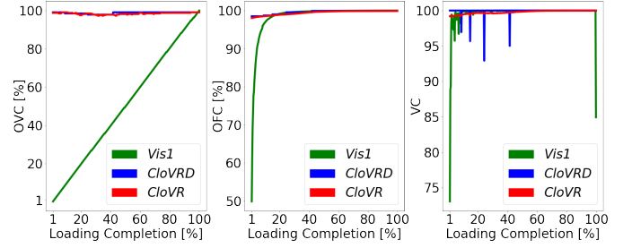
Fig. 4: Analytical comparison of loading approaches for the City VE in terms of object visualization completion (left), object footprint completion (middle), and visual continuity (right).
