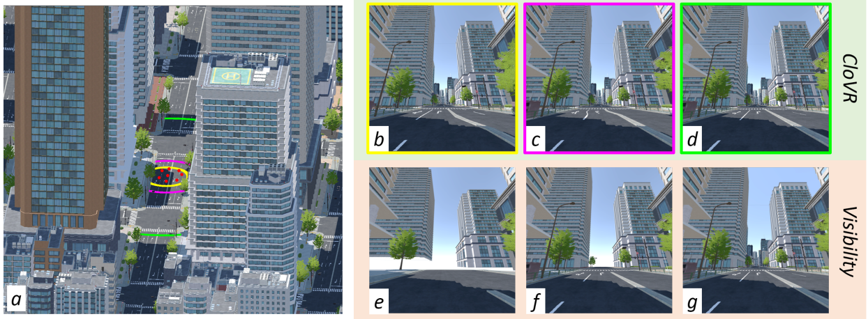
Fig. 1: (a) Overhead visualization of eight users (red dots) in a City virtual environment (VE) with 25 million triangles. The users are co-located in the same real world room and are wearing VR headsets that can render up to one million triangles. A server running on a laptop is reducing the VE either through our CloVR approach of near-far partitioning with continuous progressive refinement (b-d), or through conventional visibility computation (e-g). With CloVR the user quickly sees a complete view of the VE (b), which is then refined progressively by increasing the near region with strict visual continuity (from b to c to d). With the conventional approach the user is provided with an incomplete view (e) that is filled in as objects are received (f and g).
