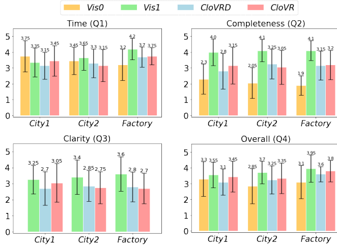
Fig. 9: Box-plots of answers to preference questionnaire for the four approaches and three VE locations, over all participants. Higher value always means better.
