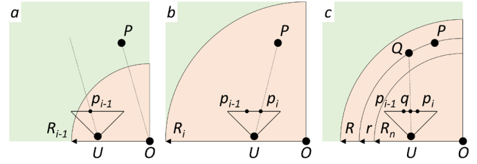
Fig. 3: Near region extension with visual continuity. Initially (panel a), the near region has radius R_{i-1} ; a VE object P is in the far region and projects to p_{i-1} . If the near region is extended abruptly to R_i (panel b), the projection of P jumps from p_{i-1} to p_i . For a near region with radius R \in [R_{i-1}, R_i] (panel c), our gradual extension projects P to the intermediate position q , as explained in Alg. 1.
