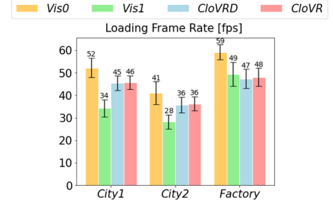
Fig. 8: Box-plots of average frame rate during loading, for the four approaches and the three VE locations, over all participants.
