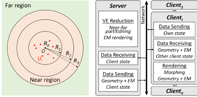
Fig. 2: CloVR approach (left) and system overview (right).
