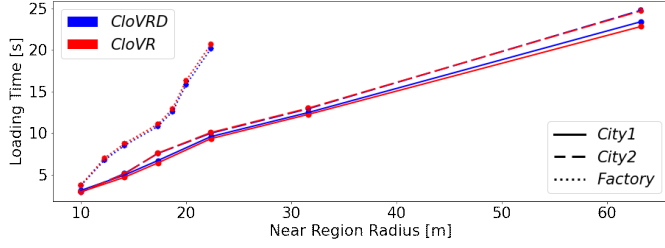
Fig. 7: Progressive loading times as a function of the growing near region radius, for the two near-far partitioning methods and the three VE locations, averaged over all Experiment 1 participants.
