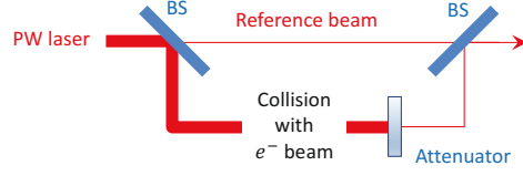
FIG. 3. Interferometer setup for detection of the laser phase change. BS: beam splitter. [Reproduced with permission from K. Qu, Phys. Plasmas 29, 042117 (2022).]
