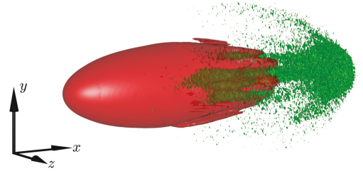
FIG. 1. A laser (red) propagating in the x direction collides with an electron beam to create a pair plasma (green). After collision, the pairs separate into two groups. One group quickly expands and continues to propagate in the beam direction. The other group is reflected and forms filaments near the center of the laser. [Reproduced with permission from K. Qu, Phys. Rev. E (2024).]
