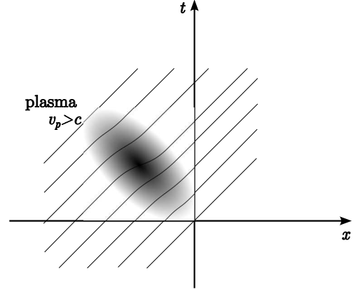
FIG. 2. Spacetime diagram of plasma creation and laser frequency upshift. [Reproduced with permission from K. Qu, Plasma Phys. Control. Fusion 65 034007 (2023).]
