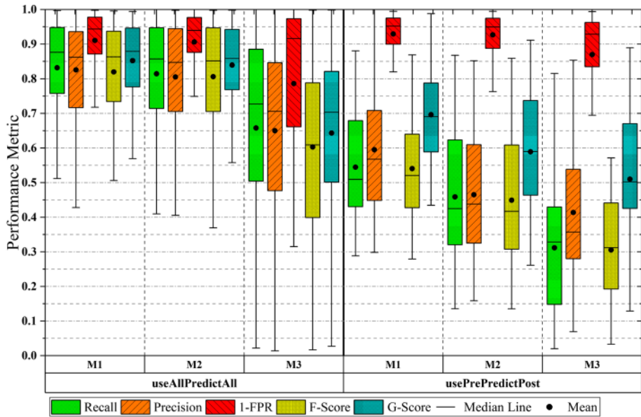
Fig. 6 Performance metrics for the two learning approaches and three prediction styles
