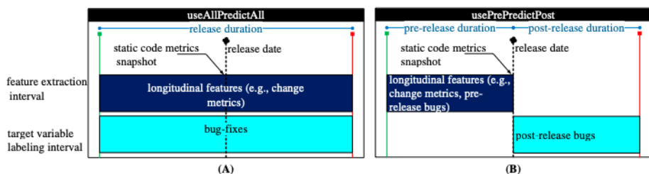
Fig. 2 Temporal aspects of the feature extraction intervals and target variable labeling intervals for the two learning approaches
