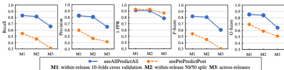
Fig. 7 Means of all performance metrics for the two learning approaches and three prediction styles
