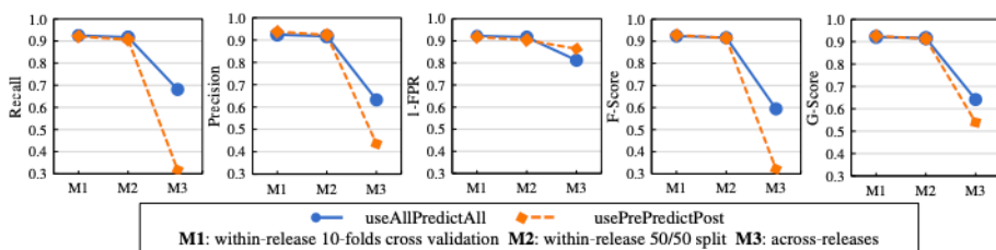
Fig. 9 Means of performance metrics for the two learning approaches and three prediction styles when SMOTE was applied
