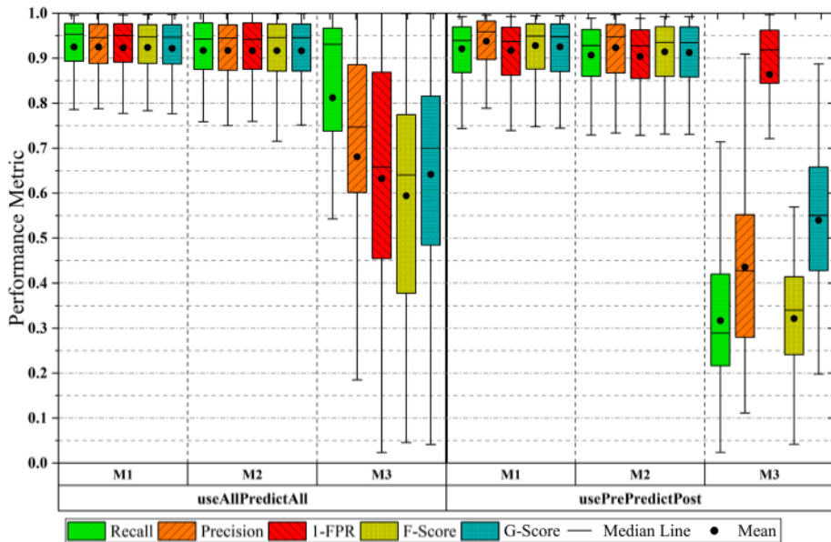
Fig. 8 Performance metrics for the two learning approaches and three prediction styles when SMOTE was applied
