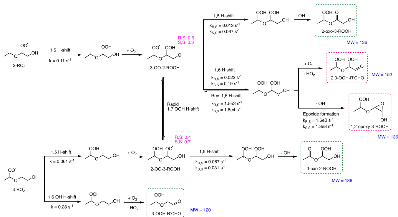
Scheme 2. Autoxidation Mechanism of the Peroxy Radicals in the 2-EE System based on Calculated H-Shift Rate Coefficients at 298.15 K a
