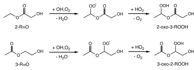
Scheme 5. Oxidation of Ethyl Glycolate (2-R=O) and 2-Hydroxyethyl Acetate (3-R=O) by OH under High \text{HO}_2 Condition
