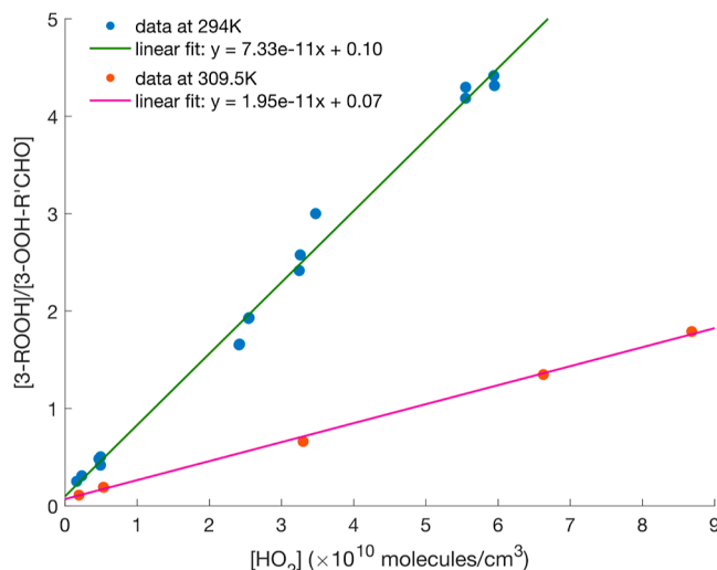
Figure 3. [3\text{-ROOH}]/[3\text{-OOH-R}'\text{CHO}] vs [\text{HO}_2] at ambient temperature (294 K) and high temperature (309.5 K) and respective unweighted linear regression fits. The uncertainties in the data are mainly systematic and are detailed in Section S6 ( \sim 25\% for concentration ratios and \sim 17\% for [\text{HO}_2] ). The respective R^2 values of the linear fits are 0.992 for ambient temperature data (green solid line) and 0.998 for high-temperature data (pink solid line).
