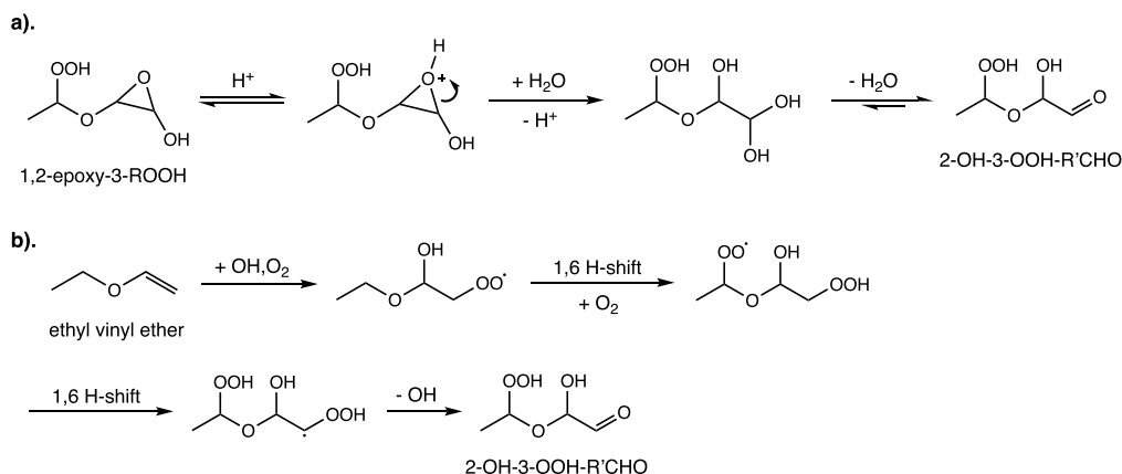
Scheme 6. Speculative Formation Pathways of 2-OH-3-OOH-R'CHO from (a) 2-EE and (b) EVE a
