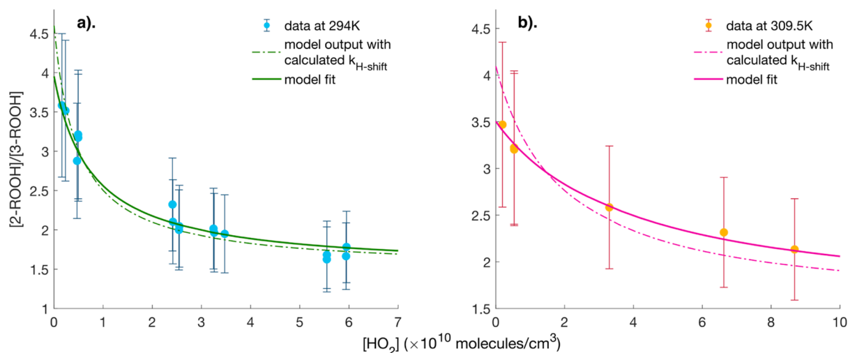
Figure 4. [2\text{-ROOH}]/[3\text{-ROOH}] vs [\text{HO}_2] at (a) ambient temperature (294 K) and (b) high temperature (309.5 K). The solid lines represent the optimized model fit to the data. The dashed lines represent the model output based on calculated H-shift rate coefficients. The uncertainties in the data are dominated by common systematic errors as detailed in Section S6 ( \sim 25\% for concentration ratios and \sim 17\% for [\text{HO}_2] ).
