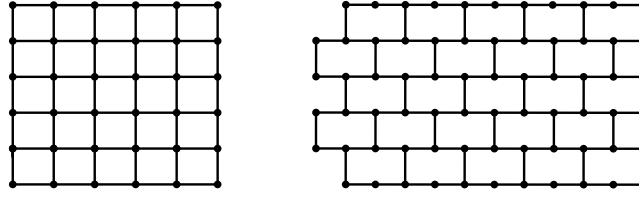
FIGURE 1. The 6-by-6 square grid (left) and the 6-by-6 wall W_{6 \times 6} (right).
