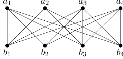
Figure 2: K(4, 4, 0) -subgraph.
