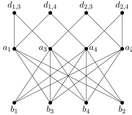
Figure 19: For the proof of 7.1, step (2).
