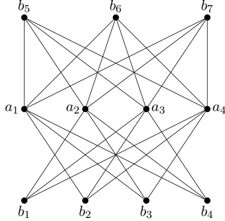
Figure 6: K(4, 7, 4) -subgraph.
