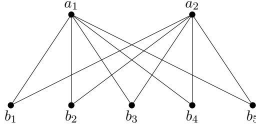
Figure 14: K(2, 5, 0) -subgraph.
