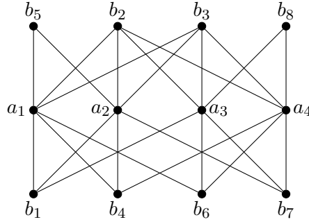
Figure 17: For the last part of the proof of 6.2. ( a_5 is not drawn.)
