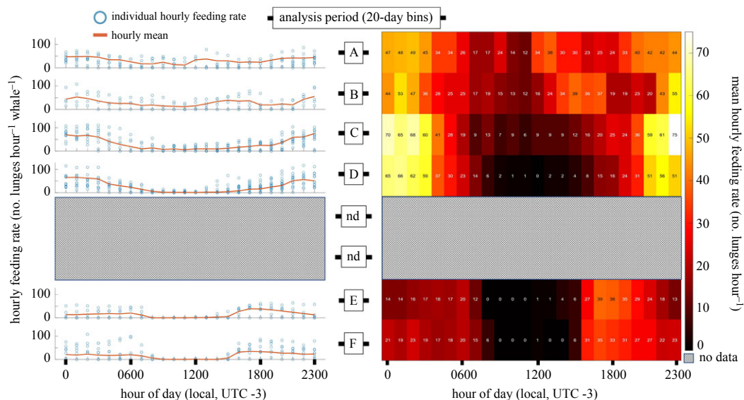
Figure 2. Seasonal feeding rates by hour of the day. The left panel shows plots for each analysis period (vertically stacked) with hourly feeding rates (y-axis) by hour of the day (x-axis) for every hour of sampled tag data. Individual hourly feeding rates are represented as a blue circle. The 40-day period between analysis period D and E is labelled as ‘nd’ for ‘no data’.
