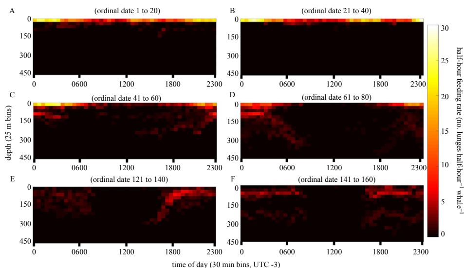
Figure 5. Heatmap of feeding rates by depth and time of day for each analysis period. Heatmaps of half-hour feeding rates over the diel period. Each plot presents data across 20-day analysis periods (A–F). Figures for ordinal dates 81–120 are absent due to insufficient data.
