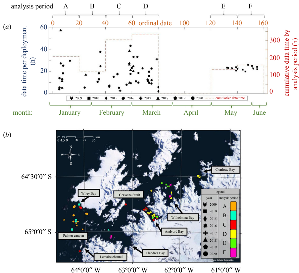
Figure 1. Study period and site. (a) Each point represents a tag deployment (left y-axis). Red dashed lines are cumulative values (right y-axis). Analysis periods A–F, encompass 20-day calendar periods: (A) 1–20 January, (B) 21 January–9 February, (C) 10 February–1 March, (D) 2–21 March, (Excluded; 22 March–30 April), (E) 1–20 May, (F) 21 May–9 June. (b) Study site and tag deployments (plotted points) by year and analysis period.
