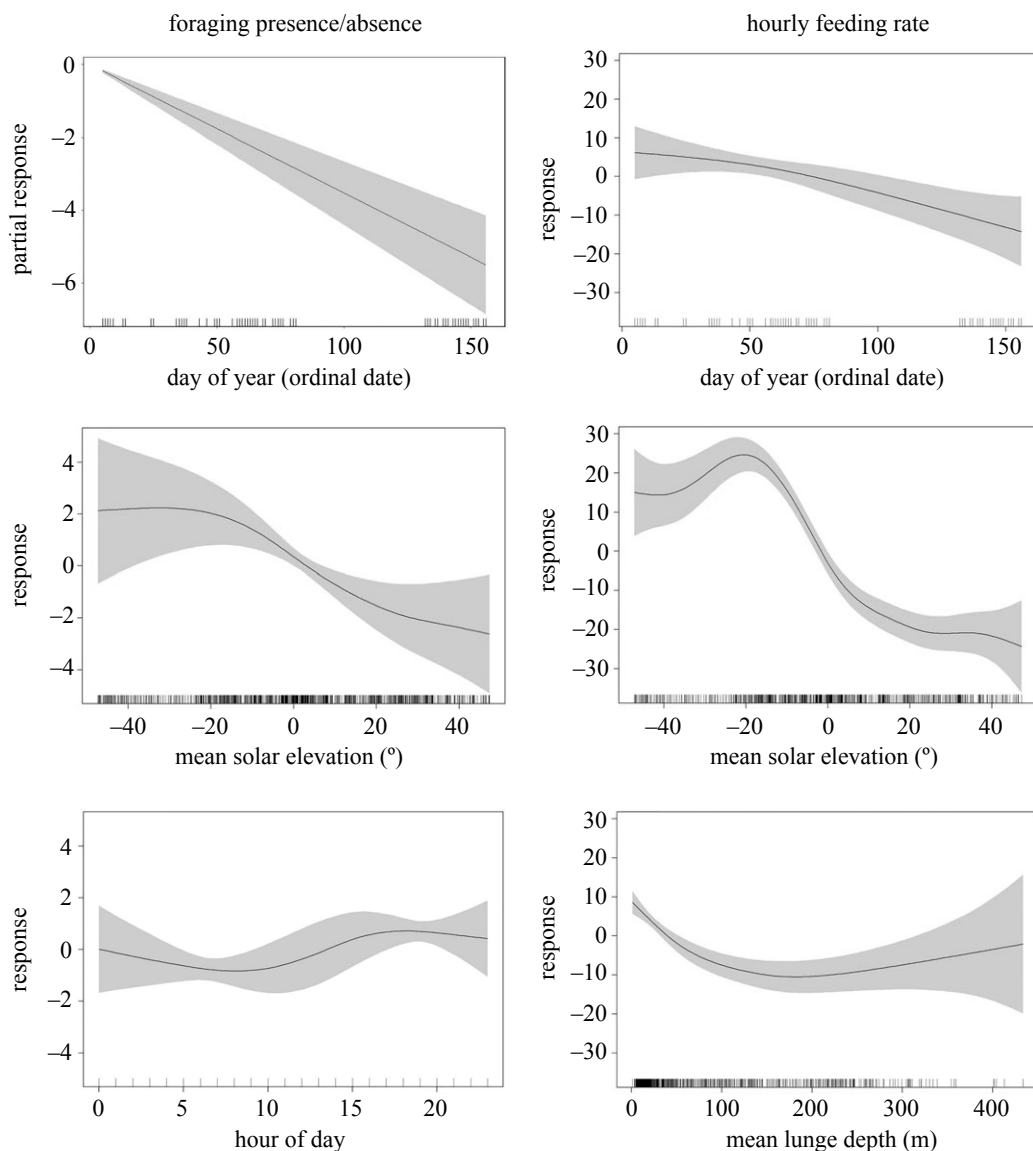
Figure 4. GAMM Response Plots for Humpback Whale Foraging: The left column shows response curves for the three covariates included in the foraging presence/absence GAMM. The right column shows response curves for the three covariates included in the hourly feeding rate GAMM. Shaded areas represent 95% confidence intervals. Rug plots on the x-axis of each plot show individual observations.
