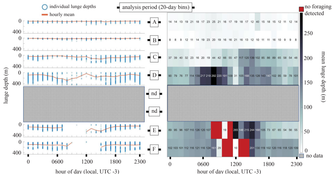
Figure 3. Seasonal feeding depths by hour of the day. The left panel shows plots for each analysis period (vertically stacked) with lunge depth ( y -axis) by hour of the day ( x -axis). Individual lunge depths are represented as a blue circle. The 40-day period between analysis period D and E is labelled as 'nd' for 'no data'.
