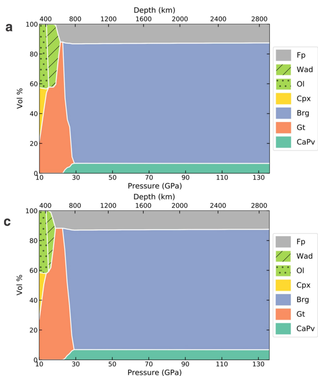
Extended Data Fig. 3 | Phase diagrams of the bulk silicate Earth (a), Theia_1 (b), Theia_2 (c) and Theia_3 (d) with geotherm from ref. 58. The FeO contents of Theia are 13 wt% (Theia_1), 15 wt% (Theia_2), and 17 wt% (Theia_3), respectively.
