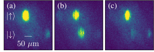
FIG. 2. Spin-momentum oscillation in a double-well SOC BEC. (a)–(c) Absorption images for \hbar\Omega_L = 0.4E_R after an evolution time of t = 0.15, 1.05 , and 1.65 \text{ ms} .
