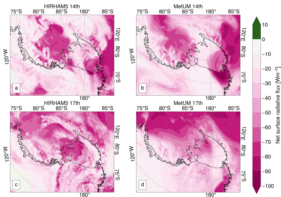
Figure 7. Maps of West Antarctica showing 3-hourly averaged net surface LW fluxes ( \text{W m}^{-2} ) at 12:00 UTC on 14 January 2016 (top row; a, b ) and 12:00 UTC on 17 January 2016 (bottom row; c, d ) from HIRHAM5 (left column; a, c ) and MetUM (right column; b, d ). Downward fluxes are positive. Note that 12:00 UTC is equivalent to 00:00 LT over the Ross Ice Shelf.
