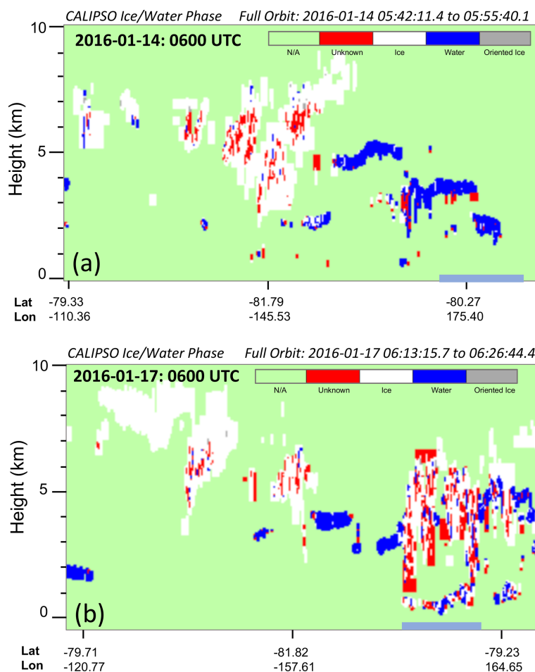
Figure 10. Observed vertical profile of cloud phase from the CALIPSO satellite over the RIS at around 06:00 UTC on (a) 14 January and (b) 17 January. The light blue bars at the bottom of each panel include the parts of the satellite ground track that overlap with the RIS region highlighted in Fig. 1. Note that 06:00 UTC is equivalent to 18:00 LT over the Ross Ice Shelf.
