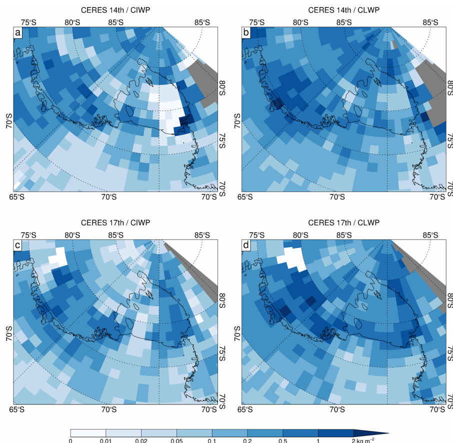
Figure 12. Maps of West Antarctica showing the cloud ice water path (CIWP; left column; a , c ; kg m -2 ) and cloud liquid water path (CLWP; right column; b , d ; kg m -2 ) at 12:00 UTC on 14 January 2016 (top row; a , b ) and 12:00 UTC on 17 January 2016 (bottom row; c , d ) from CERES observations based on 3-hourly averages. Note that 12:00 UTC is equivalent to 00:00 LT over the Ross Ice Shelf.
