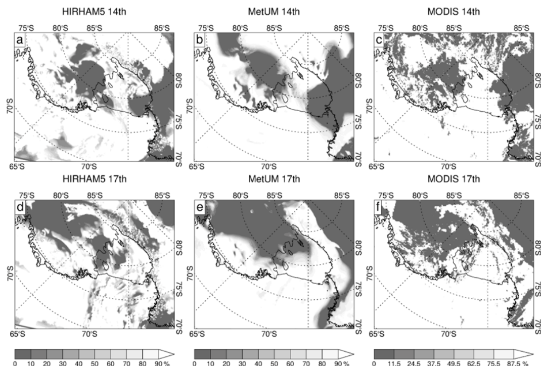
Figure 9. Maps of West Antarctica showing cloud cover (%) at 12:00 UTC on 14 January 2016 (top row; a–c ) and 12:00 UTC on 17 January 2016 (bottom row; d–f ) from HIRHAM5 (left column; a, d ), MetUM (middle column; b, e ), and MODIS (right column; c, f ). The model results are based on 6-hourly averages of low-level cloud fraction. For MODIS, a pseudo-image at 12:00 UTC was calculated by averaging two MODIS images that corresponded to satellite ground tracks over the western sector of the RIS at around 06:00 and 18:00 UTC.
