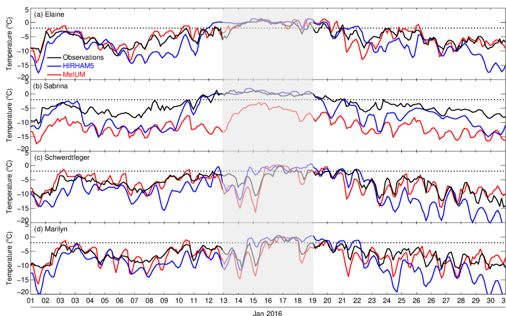
Figure 4. Time series of near-surface air temperature (°C) from the 1 to 31 January 2016 from AWS measurements (black line), HIRHAM5 output (blue line), and MetUM output (red line) at (a) Elaine, (b) Sabrina, (c) Schwerdtfeger, and (d) Marilyn. The period of special interest from 13 to 18 January is highlighted by the semi-transparent shaded region. The date shown is in UTC, with local time for the Ross Ice Shelf 12 h ahead of UTC. The horizontal dotted line shows temperatures at -2^{\circ}\text{C} , which Nicolas et al. (2017) suggests is the threshold for melting for this particular event.
