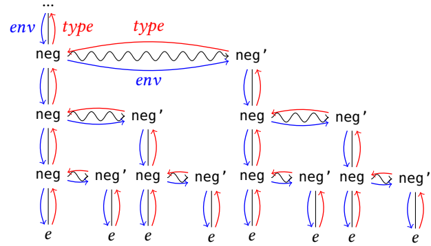
Figure 3. The resolution of operator overloading on a unary negation expression \sim (\sim (\sim e)) resulting in an exponential number of trees being created and traversed when computing type.neg' is the specialized implementation of neg for the type of e . Some labels are omitted for clarity.
