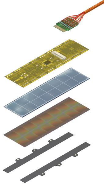
Figure 2: An exploded view of a pixel module with power and signal cables, HDI including TBM, silicon sensors, ROCs, and base strip.
