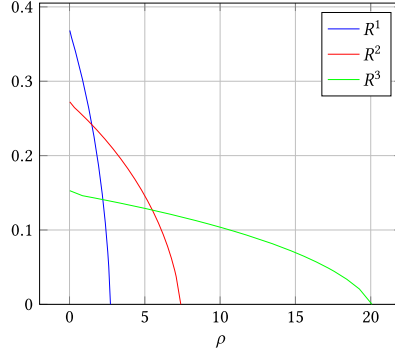
Fig. 4. Revenue of myopic policy versus other policies.
