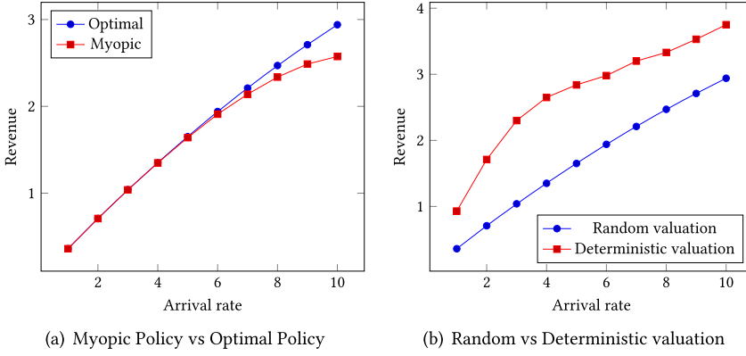
Fig. 7. Revenue variation with arrival rate.
