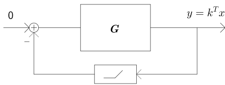
(a) Selector control illustrations in the feedback control form
