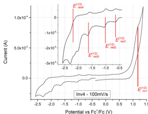
Figure 2 - Representative CV of Inv4 (1 mM) recorded in DMSO/toluene (1:1 v/v)
