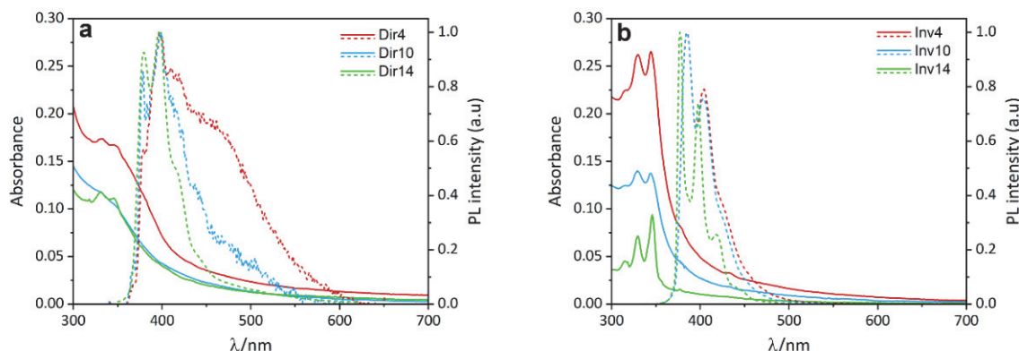
Figure 3 - Absorption and emission spectra of D- \chi -A dyads in DMSO at room temperature. Absorption (solid lines) and emission spectra (dashed lines) of (a) direct and (b) inverse dyads. Emission spectra were measured with \lambda_{\text{exc}} = 330 nm and normalized at their maximum.
