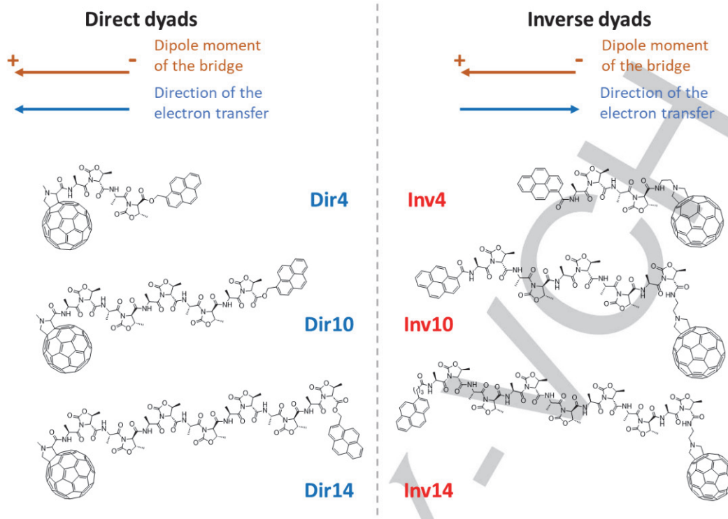
Figure 1 - Engineering of the D- \chi -A dyads. Sketched molecular structures of the six D- \chi -A dyads synthesised in this work. The Py unit acts as an electron donor (D) and the C 60 unit as an electron acceptor (A). Different chiral bridges have been probed to investigate the role of the bridge length and its electric dipole moment. Legend: Dir = direct dyad, i.e. the electric dipole moment of the bridge is parallel to the direction of ET; Inv = inverse dyad, i.e. the electric dipole moment of the bridge is antiparallel to the direction of ET; n = number of amino acids of the peptide bridge.
