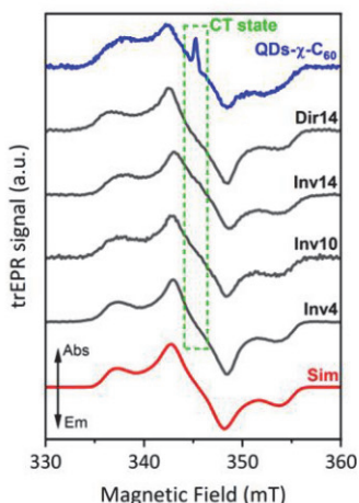
Figure 4 – trEPR spectra of D- \chi -A dyads. Normalised experimental trEPR spectra
