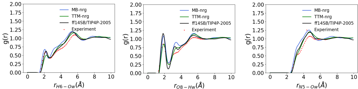
Figure 6: Radial distribution functions between different pairs of atoms located on the NMA and H 2 O molecules calculated with the MB-nrg (blue) and TTM-nrg (green) PEFs, and the ff14SB/TIP4P-2005 force field (yellow). Also shown are the EPSR-based radial distribution functions derived from NDIS measurements. 171 See main text for details.
