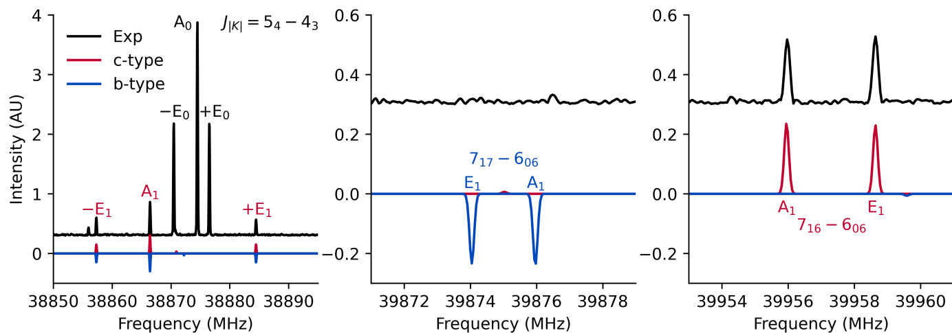
Fig. 7 (left) J_k = 5_{\pm 4} - 4_{\pm 3} transition of MTBE in the ground and torsionally excited states. The + and - labels on E correspond to the sign of K , and subscripts indicate the v_t quantum number. (center) Experimental spectrum at the location of the b -type 7_{17} - 6_{06} transition in the torsionally excited state. (right) Experimental spectrum at the location of the c -type 7_{16} - 6_{06} transition in the torsionally excited state. In all three panels, the red trace corresponds to a simulation with the dipole moment aligned to the c axis, while the downward blue trace shows a simulation with the dipole moment aligned to the b axis. The experimental spectrum has been offset by 0.3 units for clarity.
