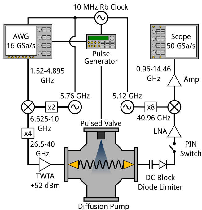
Fig. 1 Simplified block diagram of the K_a band spectrometer. A more detailed schematic is available in the ESI.
