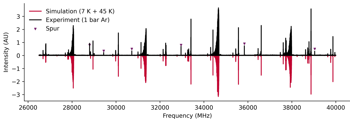
Fig. 6 K_a band spectrum of MTBE with a backing pressure of 1 bar Ar (black). The simulated spectrum is based on the S -reduction fit in Table 6, and consists of 7 K and 45 K components in a roughly 1:3 ratio. Spurious signals arising from the spectrometer digital signals are marked with purple triangles.
