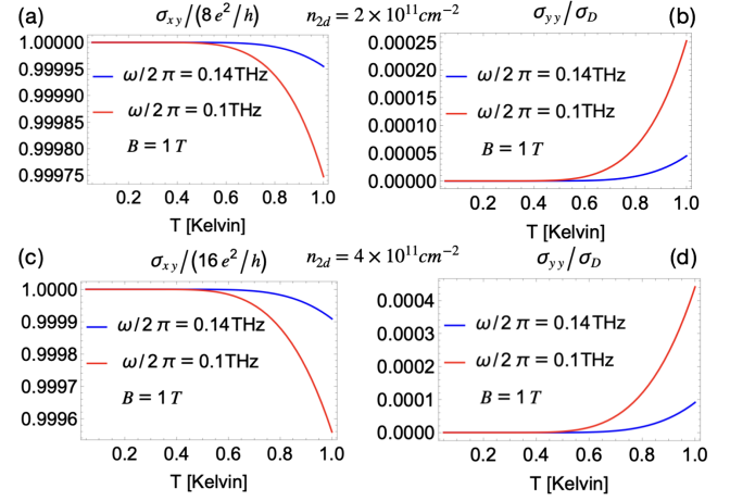
FIG. 3. Low temperature transport at magnetic field strength B = 1 T. In (a) and (b) n_{2D} = 2 \times 10^{11} \text{ cm}^{-2} while in (c) and (d) n_{2D} = 4 \times 10^{11} \text{ cm}^{-2} . The light-matter coupling strongly affects the quantum Hall transport. For the smaller cavity frequency \omega = 2\pi \times 0.1 THz and the larger electron density the deviation from the topologically protected values maximizes. This relates to the behavior of \Omega_- which controls the thermal activation in the system. The broadening parameter is chosen very small \delta = 2\pi \times 10^{-4} THz to avoid influencing transport, but guarantee numerical convergence.
