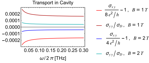
FIG. 2. Quantum Hall transport in a cavity at T = 0 with a finite broadening \delta = 2\pi \times 5 \times 10^{-3} THz for two different values of magnetic field strength B = 1 T and B = 2 T which correspond to the filling factors \nu = 8 and \nu = 4 , respectively. The 2D electron density is n_{2D} = 2 \times 10^{11} \text{ cm}^{-2} as in Ref. [23]. The Hall and the longitudinal conductivities deviate from the topologically expected values. For the smaller value of the magnetic field (higher filling factor) the deviations of the IQH transport due to the cavity are enhanced.
