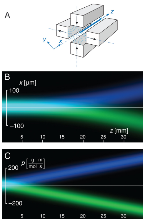
Figure 15. (A) Magnetic field gradient generated by a quadrupole arrangement of permanent magnets. The beam path indicated (solid blue line) passes through a region where the magnetic field is parallel to the y-axis, but varies in magnitude along the x-axis (uniaxial field gradient whose field lines are all parallel but vary in density in the direction perpendicular to the magnetic field). This magnetic field satisfies Maxwell's equation, cf. Figure 11. (B) Projections of the Wigner matrix elements onto the spatial axis as a function of position along the beam path through the Stern–Gerlach apparatus. (C) Projections of the Wigner matrix elements onto the transverse momentum dimension along the beam path through the apparatus. Note that in this Figure, the space-fixed axes x, y, and z are defined such that y is the quantization axis and z is the beam propagation direction. Reproduced from Ref. [64] with permission from the authors.
