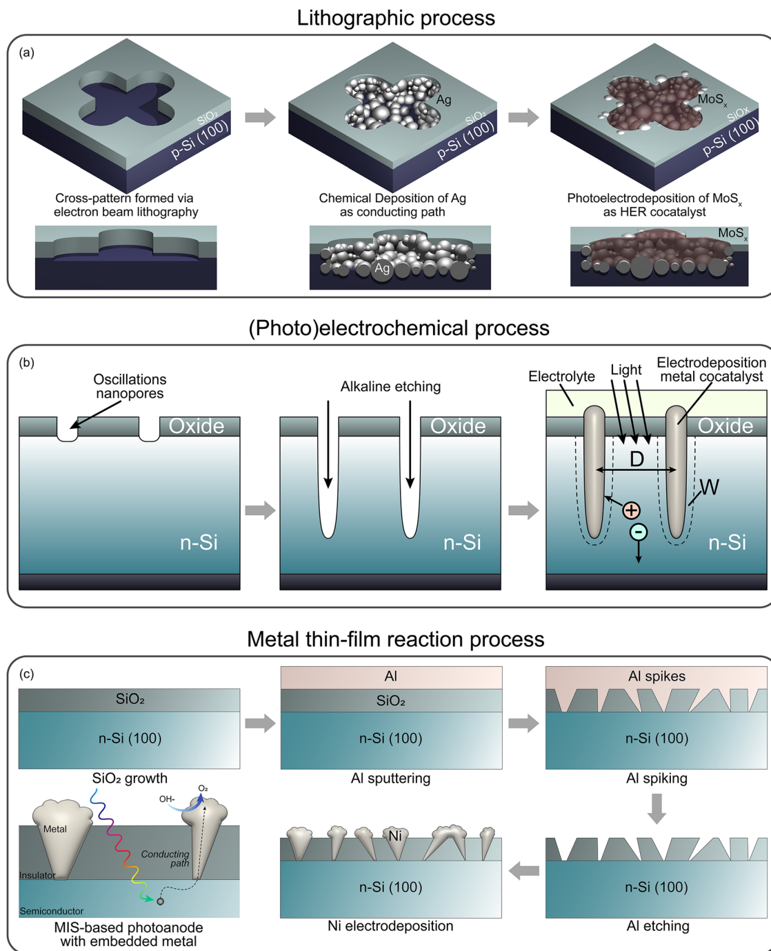
Fig. 24 Different methods of fabricating conductive pathways embedded in the insulator layers. (a) Schematic illustration of preparation procedures for the p-Si/SiO x /Ag/MoS x photocathode. The embedded cross-pattern in a 50 nm thick SiO 2 film was formed by electron beam stepper lithography. Reproduced from ref. 300 with permission from the American Chemical Society, copyright 2021. (b) Schematic illustration of preparation procedures for the nanoemitter photoelectrode. The oxide nanopores were formed by (photo)electrochemical current oscillations. Reproduced from ref. 304 with permission from the Elsevier, copyright 2008. (c) Schematic illustration of preparation procedures for the n-Si/SiO 2 /Ni photoanode. The embedded metallic conduction pathways were formed by thin-film reaction between Al and SiO 2 at the annealing temperatures of 450–600 °C. Reproduced from ref. 23 under the terms of the CC-BY 4.0 license, copyright 2021, the authors, published by Springer Nature.
