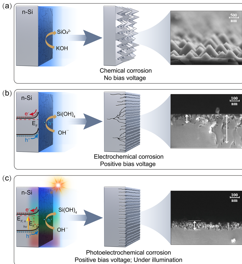
Fig. 3 Schematic illustration of the corrosion process of an n-Si photoanode for PEC water splitting in KOH electrolyte. (a) Chemical corrosion of silicon reacting with KOH leads to the formation of micro-pyramidal surface morphology. (b) Electrochemical corrosion of anodic current to oxidize electrodes leads to the formation of nanostructured silicon. (c) Photoelectrochemical corrosion of photogenerated holes to oxidize electrodes leads to the formation of nanostructured silicon within the light penetration depth. SEM images are reproduced from ref. 138 with permission from the Royal Society of Chemistry, copyright 2022.
