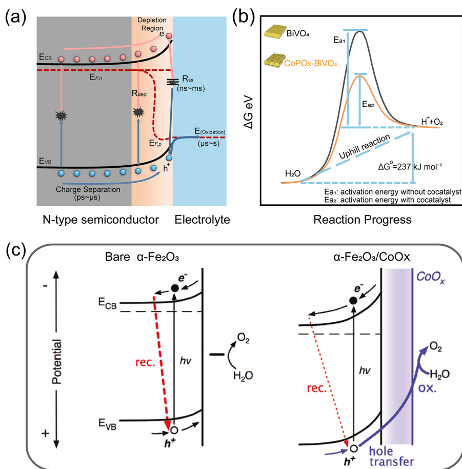
Fig. 8 Explanation of sluggish redox kinetics on semiconductors. (a) Carrier transport and main recombination paths of photogenerated carriers with the corresponding timescales for an n-type semiconductor photoelectrochemical cell without external processes of photogenerated carriers include bulk phase carrier recombination ( R_{bulk} ), depletion region recombination ( R_{depl} ), and surface state carrier recombination ( R_{ss} ). (b) Schematic diagram of the change path of Gibbs free energy in the water oxidation reaction with and without a cocatalyst. Reproduced from ref. 204 with permission from the American Chemical Society, copyright 2012. (c) Schematic diagrams illustrating that adding cobalt phosphate onto the photoanode effectively suppresses carrier recombination. Reproduced from ref. 206 with permission from the American Chemical Society, copyright 2011.
