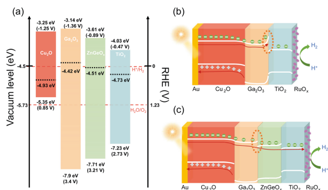
Fig. 6 Multilayer insulator synergistic strategy for MIS photoelectrodes. (a) Energy diagrams of \text{Cu}_2\text{O} , \text{Ga}_2\text{O}_3 , \text{ZnGeO}_x , and \text{TiO}_2 . (b) Schematic diagram of the photogenerated carrier transport behavior in the \text{Cu}_2\text{O}/\text{Ga}_2\text{O}_3/\text{TiO}_2/\text{RuO}_x photocathode under illumination. (c) Schematic diagram of the photogenerated carrier transport behavior in the \text{Cu}_2\text{O}/\text{Ga}_2\text{O}_3/\text{ZnGeO}_x/\text{TiO}_2/\text{RuO}_x photocathode under illumination. Reproduced from ref. 171 under the terms of the CC-BY 4.0 license, copyright 2023, the authors, published by Springer Nature.
