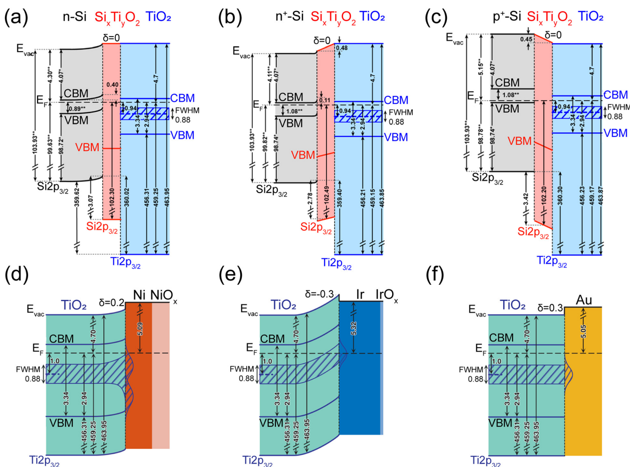
Fig. 21 (a)–(c) Energy band diagrams of the heterojunction interfaces between three different semiconductor substrates and the leaky \text{TiO}_2 , from left to right: (a) n-Si/ \text{TiO}_2 , (b) \text{n}^+\text{-Si} / \text{TiO}_2 , and (c) \text{p}^+\text{-Si} / \text{TiO}_2 . Reproduced from ref. 291 with permission from the American Chemical Society, copyright 2016. (d)–(f) Energy band diagrams of the heterojunction interfaces between the leaky \text{TiO}_2 and three metal layers with different work functions, from left to right: (d) \text{TiO}_2/\text{Ni}/\text{NiO}_x , (e) \text{TiO}_2/\text{Ir}/\text{IrO}_x , and (f) \text{TiO}_2/\text{Au} . Reproduced from ref. 293 with permission from the American Chemical Society, copyright 2021.
