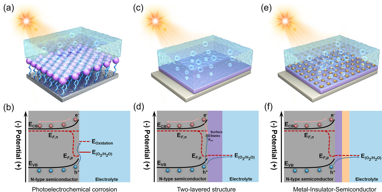
Fig. 4 Schematic illustration of various protection strategies and energy band structures. (a) Surface functionalization with electroactive reagents. (b) Energy band structure of photoelectrochemical corrosion in an n-type semiconductor. (c) Two-layered structure protection strategy. (d) Energy band structure of a two-layered photoelectrode for PEC oxygen evolution. (e) Three-layered structure protection strategy of the metal-insulator-semiconductor configuration. (f) Energy band structure of a metal-insulator-semiconductor photoelectrode for PEC oxygen evolution.
