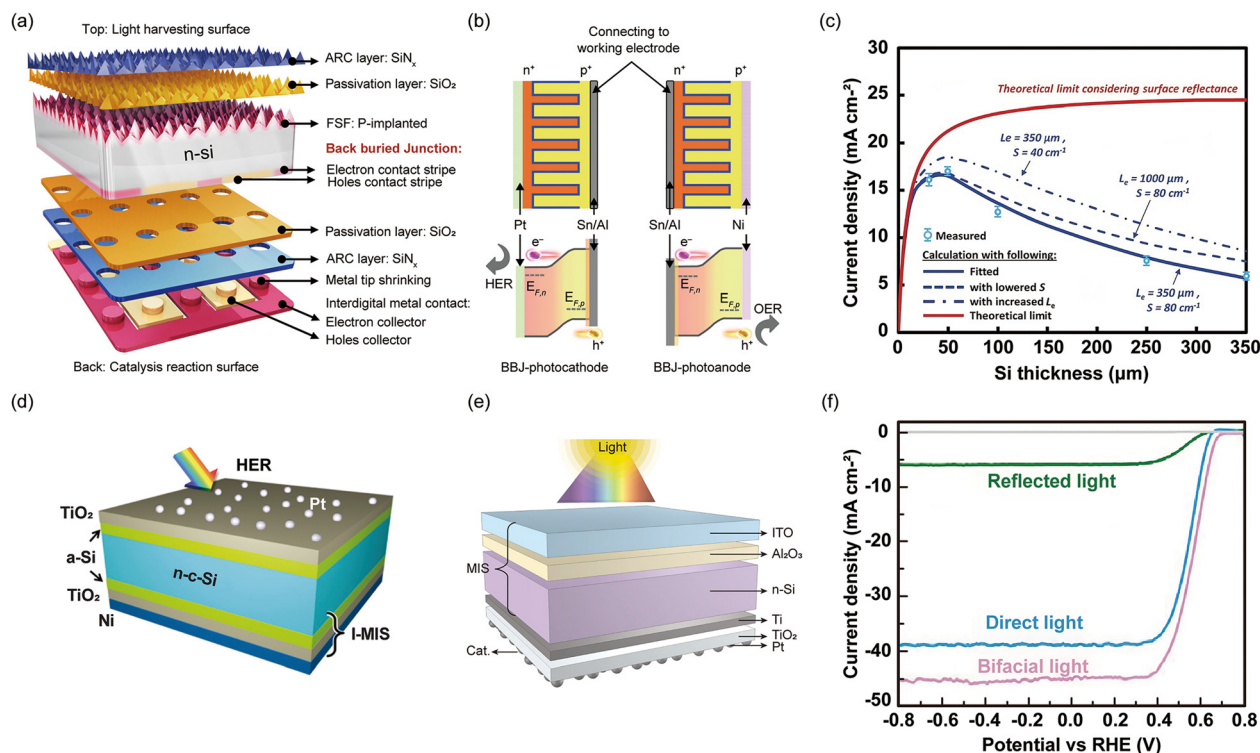
Fig. 26 Derivative configurations of single MIS photoelectrodes. (a) Schematic of the components and (b) schematic illustration of band diagrams of the back-illuminated MIS photoelectrodes with interdigitated BBJ structure. Reproduced from ref. 320 under the terms of the CC-BY 4.0 license, copyright 2023, the authors, published by Springer Nature. (c) Dependence of theoretical photocurrent density limits on silicon thickness: comparing curves at a fixed and increased carrier diffusion length ( L_e ) and surface recombination velocity ( S ). Reproduced from ref. 269 with permission from the Royal Society of Chemistry, copyright 2015. (d) Schematic illustration of the configuration of the Si I-MIS photocathode. Reproduced from ref. 172 with permission from the Royal Society of Chemistry, copyright 2020. (e) Schematic illustration of the configuration of the illumination-reaction decoupled n-Si MIS photocathode (ITO/Al 2 O 3 /n-Si/Ti/TiO 2 /Pt). Reproduced from ref. 52 under the terms of the CC-BY 4.0 license, copyright 2020, the authors, published by Oxford University Press on behalf of China Science Publishing & Media Ltd. (f) Comparison of J-V curves of a double-side Si photocathode under bifacial, direct, and reflected light illumination. Reproduced from ref. 173 with permission from John Wiley and Sons, copyright 2020.
