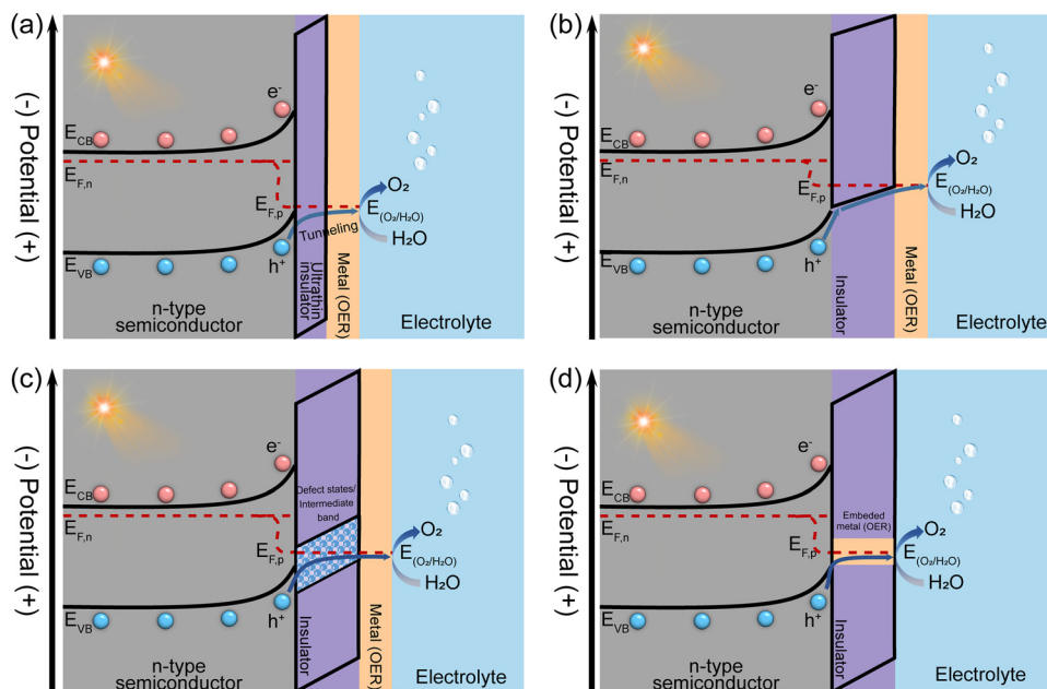
Fig. 17 Schematic illustration of band diagrams showing carrier transfer mechanisms of MIS-based photoelectrodes with n-type semiconductors. (a) Photogenerated holes tunnel through an ultrathin insulator layer usually with a thickness less than 3 nm. (b) Photogenerated holes transport across the insulator layer via its valence band. (c) Photogenerated holes transport across the insulator layer via defect states or intermediate bands. (d) Photogenerated holes transport across the insulator layer via embedded metal conduction paths.
