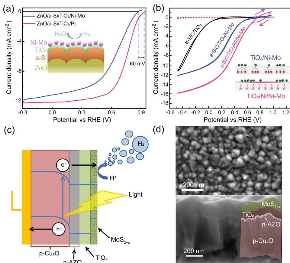
Fig. 11 Earth-abundant transition-metal-based cocatalysts in the MIS photocathode for the HER. (a) LSV plots of amorphous Si MIS-based photocathodes with a Ni–Mo or Pt catalyst. Reproduced from ref. 220 with permission from the American Chemical Society, copyright 2013. (b) CV curves of a-SiC/TiO 2 , a-SiC/TiO 2 /Ni–Mo and a-SiC/TiO 2 /Ni/Ni–Mo in a 1 M KOH electrolyte. The inset image shows the role of the Ni layer in facilitating the transfer of photogenerated carriers to the Ni–Mo cocatalysts. Reproduced from ref. 224 with permission from the Royal Society of Chemistry, copyright 2016. (c) Schematic structure of the p-Cu 2 O/n-AZO/TiO 2 /MoS 2+x MIS photocathode. The combination of n-AZO and p-Cu 2 O formed a photovoltaic p–n junction, leading to an enhanced photogenerated voltage. The TiO 2 layer safeguarded the buried p-Cu 2 O/n-AZO junction from exposure to the aqueous environment; (d) Surface and cross-sectional SEM images of a p-Cu 2 O/n-AZO/TiO 2 /MoS 2+x MIS photocathode. Reproduced from ref. 227 with permission from Springer Nature, copyright 2014.
