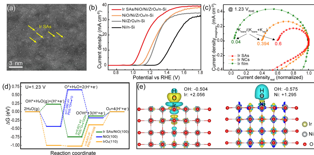
Fig. 16 Single-atom cocatalysts for MIS-based photoelectrodes. (a) HAADF-STEM image of an Ir SAs/NiO thin-film catalyst. (b) LSV curves of the following photoanodes: Ni/n-Si, Ni/ZrO 2 /n-Si, NiO/Ni/ZrO 2 /n-Si, and Ir SAs/NiO/Ni/ZrO 2 /n-Si. (c) Nyquist plots of Ir SAs, Ir NCs, and Ir film at an applied potential of 1.23 V vs. RHE. (d) Free energy diagrams of the OER on Ir SAs/NiO (100), NiO (100), and IrO 2 (110) at an applied potential of 1.23 V vs. RHE. (e) Charge density redistribution diagrams of Ir SAs/NiO and NiO during the OER. Reproduced from ref. 263 under the terms of the CC-BY 4.0 license, copyright 2023, the authors, published by Springer Nature.
