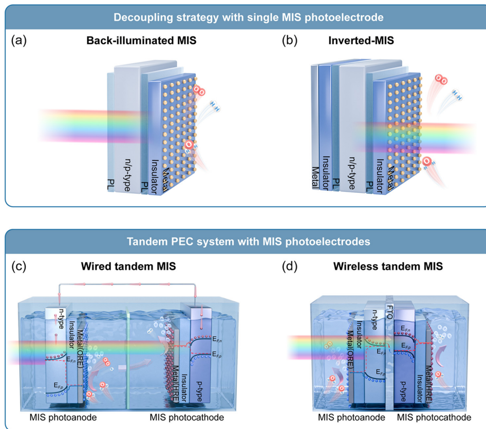
Fig. 25 Schematic illustration of derivative MIS configurations for PEC water splitting. Single MIS photoelectrodes: (a) back-illuminated MIS photoelectrode configuration and (b) inverted-MIS photoelectrode configuration (PL represents an ultra-thin passivation layer). Tandem MIS photoelectrodes: (c) wired tandem MIS photoelectrodes and (d) wireless monolithic tandem PEC system with MIS photoelectrodes.
