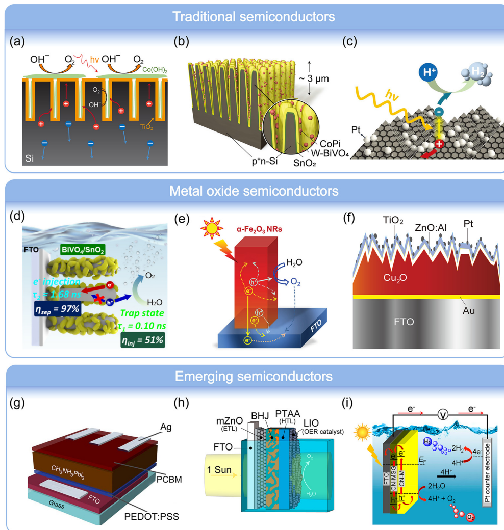
Fig. 2 Schematic illustration of the configuration of different semiconductor material photoelectrodes. (a) The charge generation and oxygen evolution processes in the MIS photoanode b-Si/TiO 2 /Co(OH) 2 . Reproduced from ref. 50 with permission from Springer Nature, copyright 2017. (b) The integrated tandem photoanode b-Si/SnO 2 /BiVO 4 /CoPi. Reproduced from ref. 74 with permission from John Wiley and Sons, copyright 2017. (c) The 3D pyramid-shaped graphene/p-type silicon Schottky junction photocathode. Reproduced from ref. 48 with permission from John Wiley and Sons, copyright 2019. (d) Schematics of charge carrier transfer of a BiVO 4 /SnO 2 heterostructure photoanode. Reproduced from ref. 96 with permission from Elsevier, copyright 2021. (e) Schematic illustration of three main photogenerated carrier recombination pathways in hematite photoanodes. Reproduced from ref. 108 with permission from John Wiley and Sons, copyright 2015. (f) Schematic diagram of a MIS-based Cu 2 O/Al-ZnO/TiO 2 /Pt photocathode structure. Reproduced from ref. 113 with permission from Springer Nature, copyright 2011. (g) The configuration of the inverted halide perovskite used for the photocathode. Reproduced from ref. 123 under the terms of the CC-BY 4.0 license, copyright 2016, the authors, published by Springer Nature. (h) The donor-acceptor bulk heterojunction polymer semiconductor photoanode for solar water oxidation. Reproduced from ref. 129 with permission from Springer Nature, copyright 2021. (i) The dual-layer carbon nitride heterostructure photoanode for PEC water oxidation. Reproduced from ref. 133 with permission from the American Chemical Society, copyright 2020.
