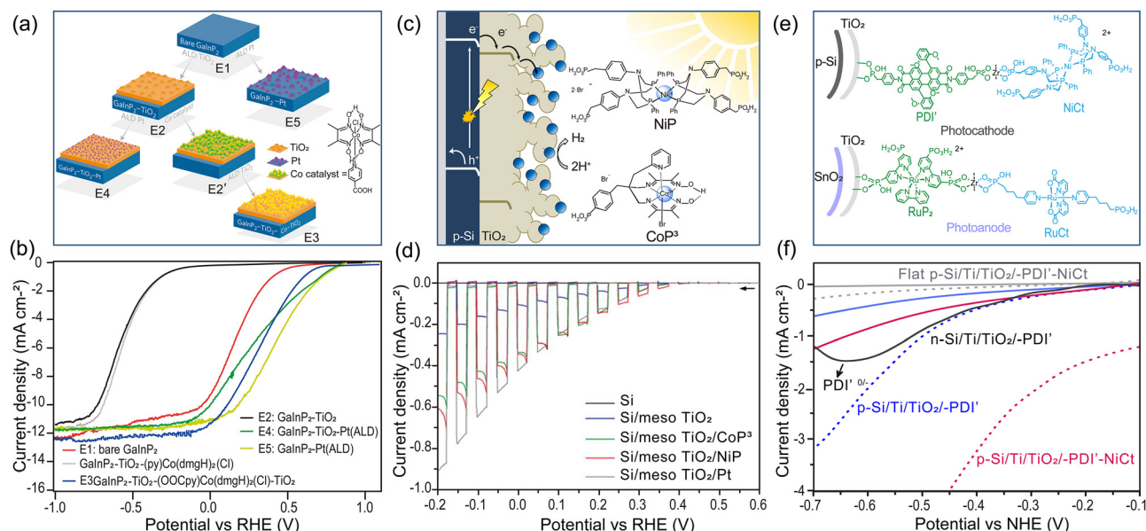
Fig. 14 Molecular cocatalysts for MIS-based photoelectrodes. (a) Schematic diagram of the preparation process of the p-GaInP 2 photoelectrode modified with Co-based molecular cocatalysts; (b) LSV curves of a MIS-based photoelectrode with the target cobalt molecular catalyst (E3) and other comparative photoelectrodes. Reproduced from ref. 251 with permission from Springer Nature, copyright 2015. (c) Schematic diagram of a Si/mesoTiO 2 /NiP or CoP 3 photocathode; (d) LSV curves of Si, Si/mesoTiO 2 , and Si/mesoTiO 2 /CoP 3 or NiP or Pt. Reproduced from ref. 252 under the terms of the CC-BY 3.0 license, copyright 2017, the authors, published by the Royal Society of Chemistry. (e) Structure of the p-Si/TiO 2 /PDI'-NiCt photocathode and a dye-sensitized SnO 2 /TiO 2 /RuP 2 -RuCt photoanode; (f) LSV curves of p-Si/TiO 2 /PDI' (blue), n-Si/TiO 2 /PDI' (black), p-Si/TiO 2 /PDI'-NiCt (red) and flat p-Si/TiO 2 /PDI'-NiCt (gray) under dark (solid line) or illumination (dashed line) conditions. Reproduced from ref. 253 with permission from the American Chemical Society, copyright 2019.
