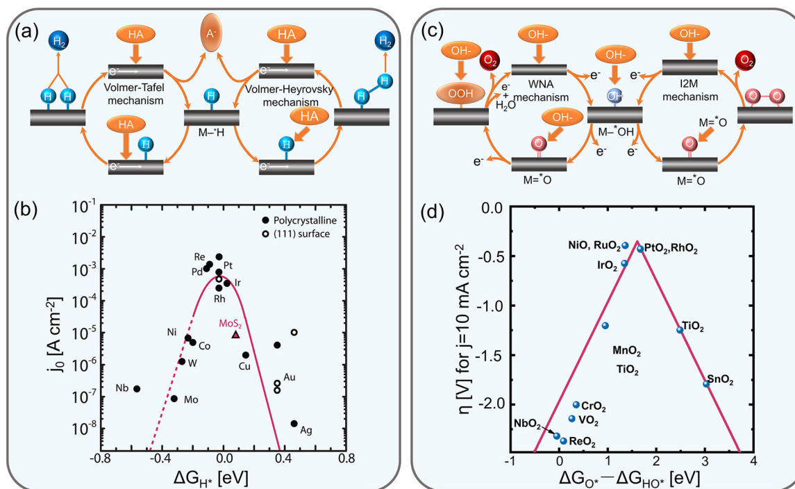
Fig. 9 Schematic diagram of the mechanism pathways of HER and OER reactions on metal-based catalysts and volcano plots of the common metal-based catalysts for HER and OER reactions. (a) Volmer–Tafel mechanism based on chemical desorption and Volmer–Heyrovsky mechanism based on electrochemical desorption. The \text{A}^- species depends on the pH of the electrolyte. In an acidic solution, it corresponds to \text{H}_2\text{O} , whereas in an alkaline solution, it represents \text{OH}^- . (b) HER volcano plot depicting a function of the calculated free energy for hydrogen adsorption ( \Delta G_{\text{H}^*} ) and experimentally measured current density ( j_0 ) for metals and \text{MoS}_2 . Reproduced from ref. 207 with permission from American Association for the Advancement of Science, copyright 2017. (c) WNA mechanism for single-site water oxidation and I2M mechanism for two-site coupling interaction in an alkaline electrolyte. (d) OER volcano plot depicting a function of the calculated free energy of ( \Delta G_{\text{O}^*} - \Delta G_{\text{HO}^*} ) and negative value of experimentally measured overpotential ( \eta ) for metal oxide catalysts. Reproduced from ref. 231 with permission from John Wiley and Sons, copyright 2011.
