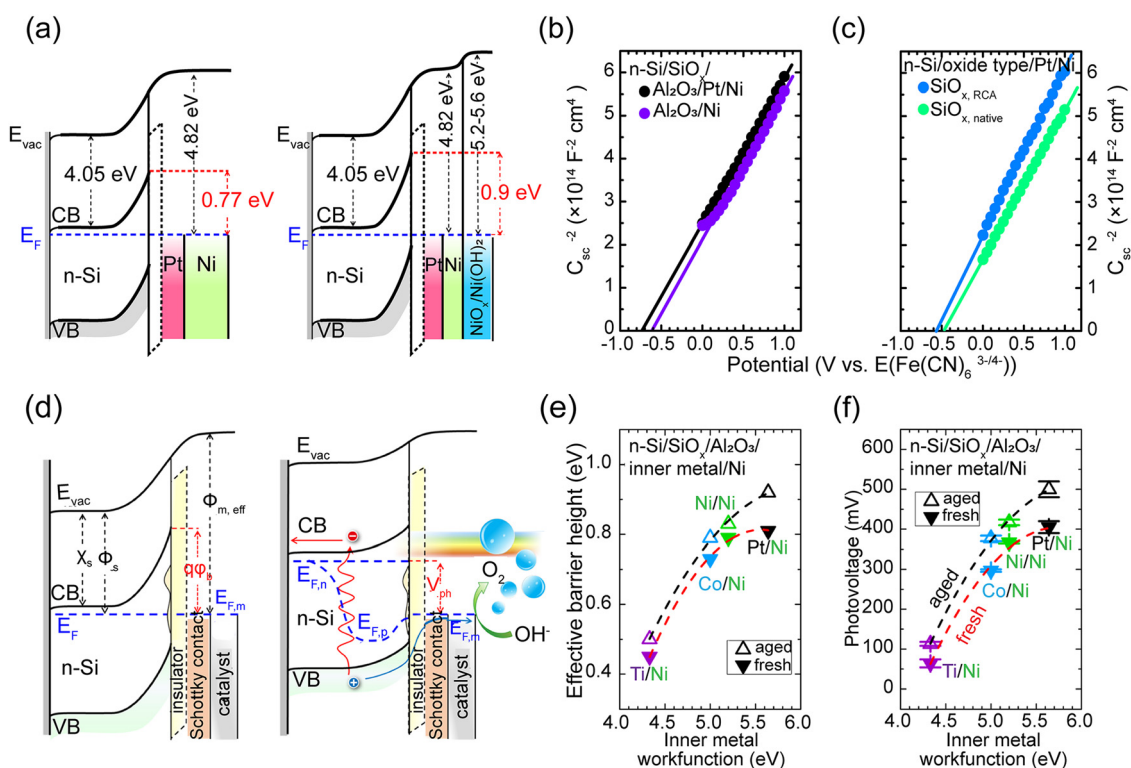
Fig. 19 (a) Energy band diagram of the fresh n-Si/ \text{SiO}_{x,\text{RCA}}/\text{Al}_2\text{O}_3/\text{Pt}/\text{Ni} photoelectrode (left) and that after an 18-hour aging process in KOH (right); (b) Mott–Schottky plots of n-Si/ \text{SiO}_{x,\text{RCA}}/\text{Al}_2\text{O}_3/\text{Pt} (2 nm)/Ni (4 nm) and n-Si/ \text{SiO}_{x,\text{RCA}}/\text{Al}_2\text{O}_3/\text{Ni} (6 nm); (c) Mott–Schottky plots of n-Si/ \text{SiO}_{x,\text{RCA}}/\text{Pt}/\text{Ni} and n-Si/ \text{SiO}_{x,\text{native}}/\text{Pt}/\text{Ni} . Reproduced from ref. 152 under the terms of the CC-BY 4.0 license, copyright 2017, the authors, published by Springer Nature. (d) Energy band diagram of MIS-based photoanodes in the dark and under illumination; (e) effective barrier height as a function of the inner metal work function of n-Si/ \text{SiO}_x/\text{Al}_2\text{O}_3 /inner metal/Ni photoanodes; (f) photovoltage as a function of the inner metal work function of n-Si/ \text{SiO}_x/\text{Al}_2\text{O}_3 /inner metal/Ni photoanodes. Reproduced from ref. 266 under the terms of the CC-BY 4.0 license, copyright 2018, the authors, published by the American Chemical Society.
