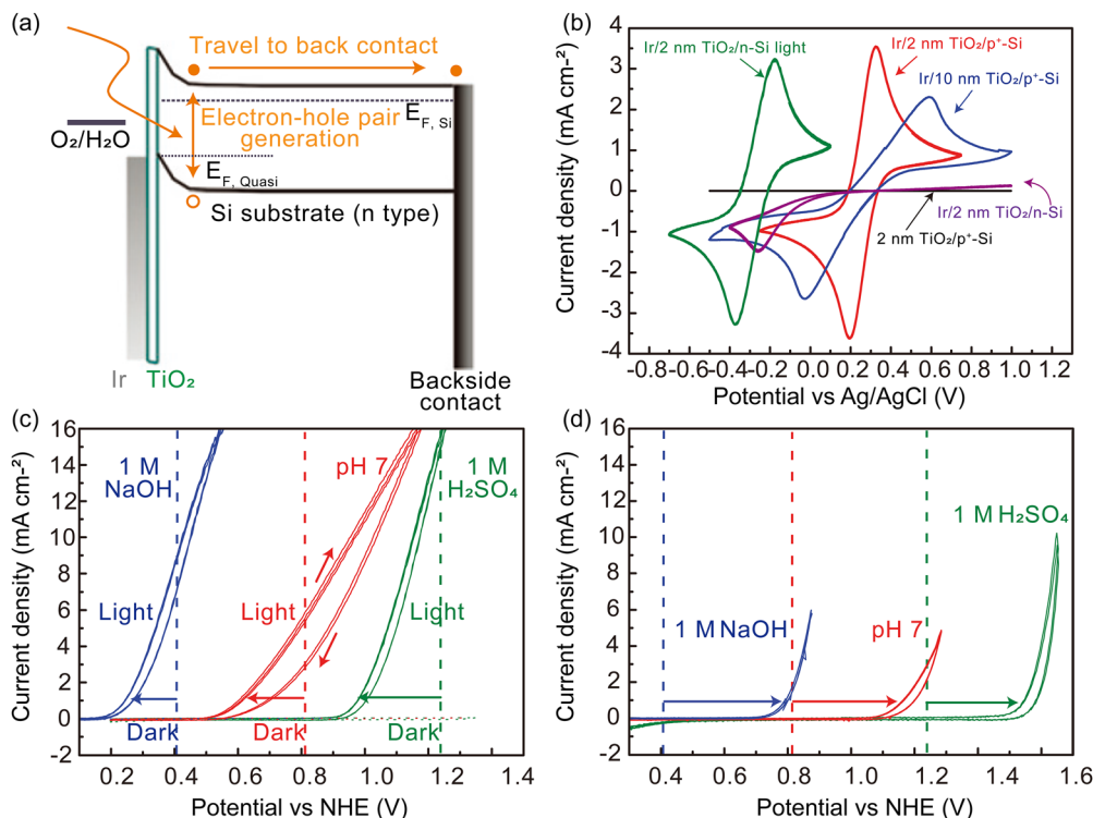
Fig. 12 Noble metal cocatalysts in the MIS-based photoanode for the OER. (a) Energy band diagram of the Ir/TiO 2 /SiO 2 /n-Si photoanode. (b) CV curves in ferri/ferrocyanide solutions of 2 nm TiO 2 /p + -Si (black line, in the dark), Ir/2 nm TiO 2 /p + -Si (red line, in the dark), Ir/10 nm TiO 2 /p + -Si (blue line, in the dark), Ir/2 nm TiO 2 /n-Si (violet line, in the dark), and Ir/2 nm TiO 2 /n-Si (green line, under 1 sun illumination). (c) LSV plots of Ir/TiO 2 /n-Si measured with (lines) and without (dots) simulated solar irradiation at 1 sun (AM1.5G) in acidic (1 M H 2 SO 4 ), neutral (1 M phosphate-buffered, pH 7) and basic (1 M NaOH) solutions. (d) LSV plots of Ir/TiO 2 /p + -Si measured in the dark for acidic, neutral, and basic solutions. The dashed vertical lines in (c) and (d) indicate the thermodynamic redox potential for water oxidation at the corresponding pH values. Reproduced from ref. 17 with permission from Springer Nature, copyright 2011.
