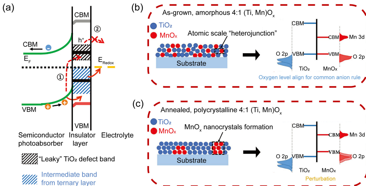
Fig. 23 (a) Schematic diagram comparing the carrier transfer mechanism through the defect states or intermediate bands of TiO 2 films. (b) Schematic diagram of the microstructure of the as-grown (Ti, Mn)O x film and the relative positions of energy levels in the atomic scale heterojunction. (c) Schematic diagram of the microstructure of the annealed (Ti, Mn)O x film and the relative positions of energy levels in the TiO 2 /MnO x nanocluster bulk heterojunction. Reproduced from ref. 193 with permission from John Wiley and Sons, copyright 2022.
