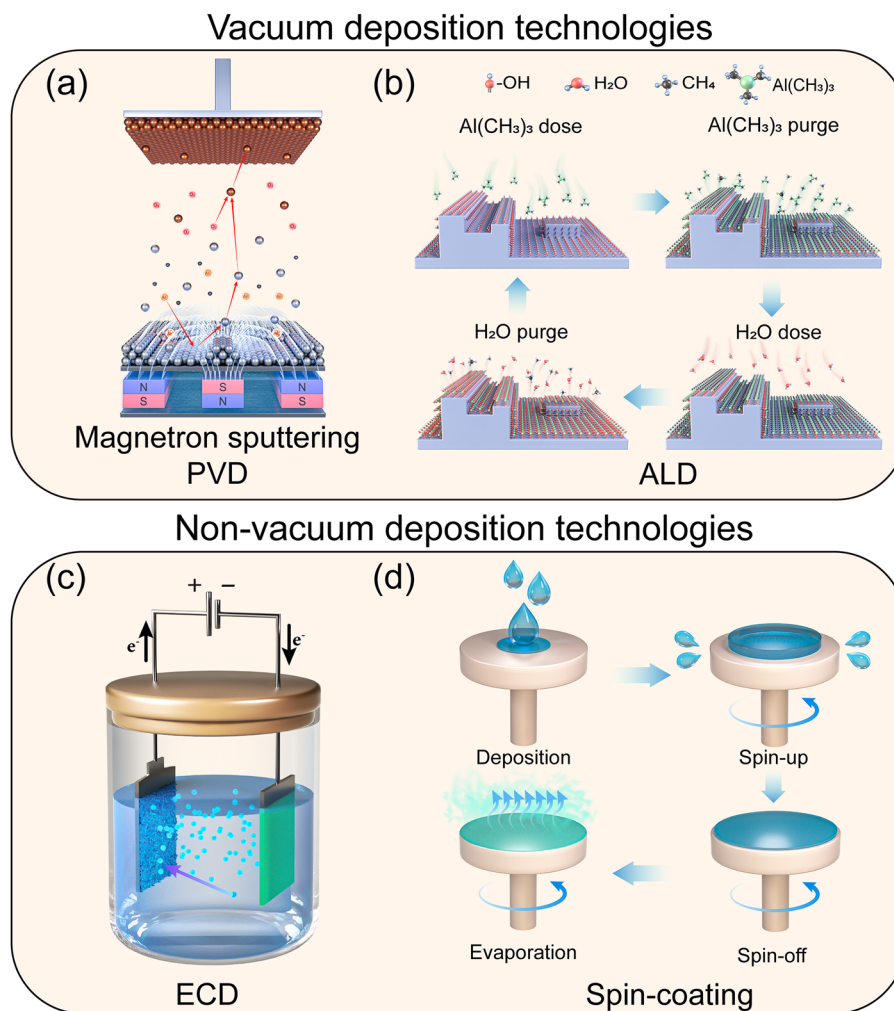
Fig. 7 Schematic diagram of the preparation of insulator layers based on vacuum deposition technologies and non-vacuum deposition technologies. (a) Deposition of \text{TiO}_2 films by reactive magnetron sputtering with oxygen. (b) Deposition of conformal \text{Al}_2\text{O}_3 films by the ALD technique on a nanostructured substrate. (c) Electric-field induced electrochemical deposition technique. (d) Spin-coating deposition technique.
