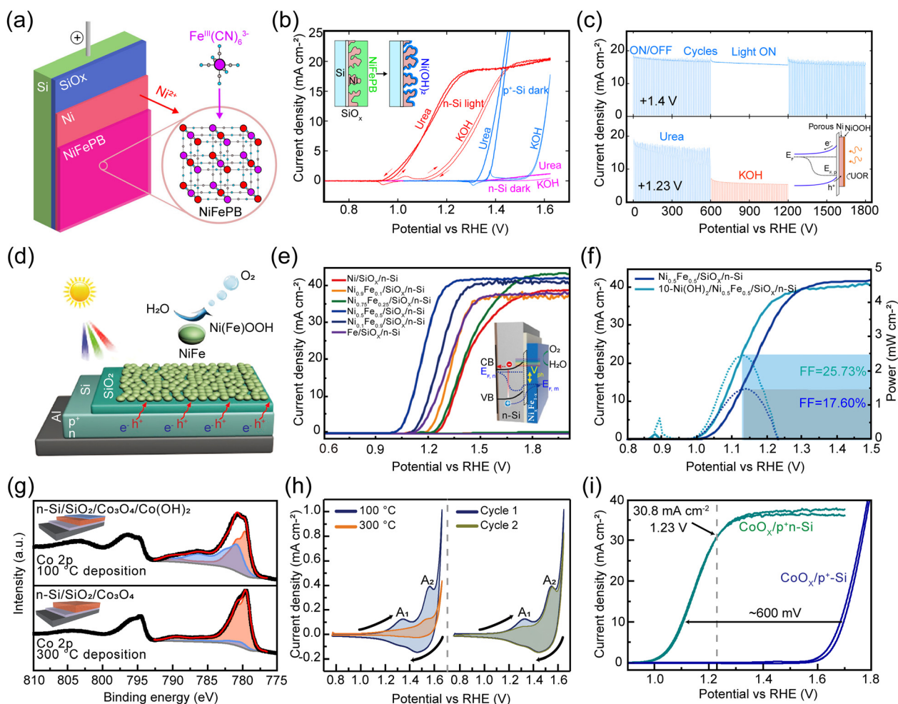
Fig. 13 Earth-abundant transition-metal-based cocatalysts in MIS-based photoanodes for the OER. (a) Schematic structure of the Si/SiO x /Ni/NiFePB MIS photoanode. The redox-active NiFePB was prepared by electrochemically oxidizing the Ni layer in a K 3 Fe(CN) 6 electrolyte; (b) CV curves of n-Si/SiO x /Ni/NiFePB (red) under illumination, p + -Si/SiO x /Ni/NiFePB (blue) in the dark, and n-Si/SiO x /Ni/NiFePB (pink) in the dark with the electrolyte of 1 M KOH and 0.33 M urea + 1 M KOH; (c) current density vs. time plots for UOR on Si/SiO x /Ni/NiFePB recorded at 1.40 V (top) and 1.23 V (down) while the electrolyte was replaced at 600 s by 1 M KOH. Reproduced from ref. 239 under the terms of the CC-BY 4.0 license, copyright 2019, the authors, published by Springer Nature. (d) Schematic structure of the np + -Si/SiO x /NiFe MIS photoanode. Reproduced from ref. 240 with permission from John Wiley and Sons, copyright 2017. (e) LSV curves of the n-Si/SiO x /Ni 0.5 Fe 1-x photoanodes; (f) LSV curves of the n-Si/SiO x /Ni 0.5 Fe 0.5 photoanodes with and without additional Ni(OH) 2 cocatalysts. Reproduced from ref. 243 with permission from Elsevier, copyright 2022. (g) XPS analysis of Co 2p for CoO x films deposited at 100 °C (top) and 300 °C (down); (h) CV curves of CoO x films deposited at 100 °C and 300 °C (left) and comparison of first and second CV curve of CoO x films deposited at 100 °C (right); (i) LSV plots of p + n-Si/SiO x /Co 3 O 4 /Co(OH) 2 under illumination and p + n-Si/SiO x /Co 3 O 4 /Co(OH) 2 in the dark. Reproduced from ref. 245 with permission from Springer Nature, copyright 2016.
