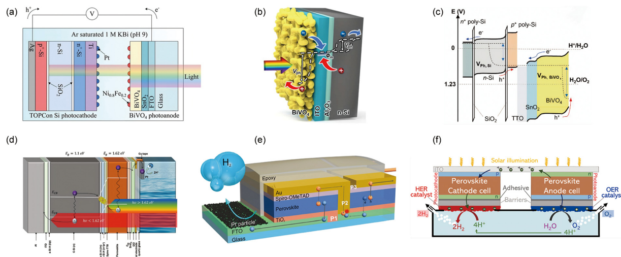
Fig. 27 Derivative configurations of tandem MIS photoelectrodes. (a) The wired tandem PEC cell was constructed using a \text{BiVO}_4 photoanode as the top cell and a TOPCon Si photocathode as the bottom cell. Reproduced from ref. 327 with permission from the Royal Society of Chemistry, copyright 2023. (b) Schematic illustration of the configuration of the \text{n-Si}/\text{Al}_2\text{O}_3/\text{ITO}/\text{BiVO}_4 integrated tandem photoanode. Reproduced from ref. 331 under the terms of the CC-BY 4.0 license, copyright 2023, the authors, published by the Royal Society of Chemistry. (c) Schematic illustration of band diagrams of the \text{BVO}/\text{SnO}_2/\text{TTO}/\text{TOPCon Si} integrated tandem photoanode. Reproduced from ref. 332 with permission from John Wiley and Sons, copyright 2020. (d) Schematic illustration of the configuration of the Pt/quartz glass/perovskite/silicon tandem photocathode for water splitting. Reproduced from ref. 340 with permission from John Wiley and Sons, copyright 2021. (e) Schematic illustration of the configuration of the optically parallel and electrically series-connected dual perovskite module photocathode. Reproduced from ref. 338 with permission from John Wiley and Sons, copyright 2023. (f) Schematic illustration of the configuration of a CAB-protected perovskite tandem photocathode and photoanode in co-planar series. Reproduced from ref. 339 under the terms of the CC-BY 4.0 license, copyright 2023, the authors, published by Springer Nature.
