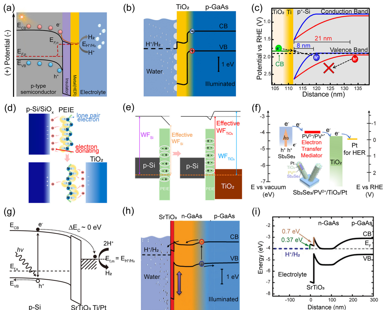
Fig. 20 (a) Schematic illustration of band diagrams showing the conduction band-based carrier transport mechanism of an MIS-based photocathode. (b) Energy band diagrams of a p-GaAs/TiO 2 /Pt photocathode under illumination. Reproduced from ref. 274 with permission from John Wiley and Sons, copyright 2020. (c) Energy band diagrams of an np + -Si/5 nm Ti/100 nm TiO 2 /Pt Film photoelectrode under illumination. Reproduced from ref. 146 with permission from the American Chemical Society, copyright 2015. (d) Schematic illustration of the dipole reorientation strategy mechanism; (e) energy level diagram of p-Si/PEIE (left) and p-Si/PEIE/TiO 2 (right). Reproduced from ref. 281 with permission from the American Chemical Society, copyright 2022. (f) Energy band diagrams of the Sb 2 Se 3 /PV 2+ /TiO 2 /Pt photocathode. The inset image is the schematic structure of the Sb 2 Se 3 /PV 2+ /TiO 2 /Pt photocathode. Reproduced from ref. 283 under the terms of the CC-BY 4.0 license, copyright 2022, the authors, published by Elsevier. (g) Energy band diagrams of a p-Si/SrTiO 3 /Ti/Pt photocathode. Reproduced from ref. 21 with permission from Springer Nature, copyright 2014. (h) Schematic structure of the np-GaAs/SrTiO 3 photocathode under illumination; (i) energy band diagrams of the np-GaAs/SrTiO 3 photocathode. Reproduced from ref. 284 under the terms of the CC-BY 3.0 license, copyright 2017, the authors, published by the Royal Society of Chemistry.
