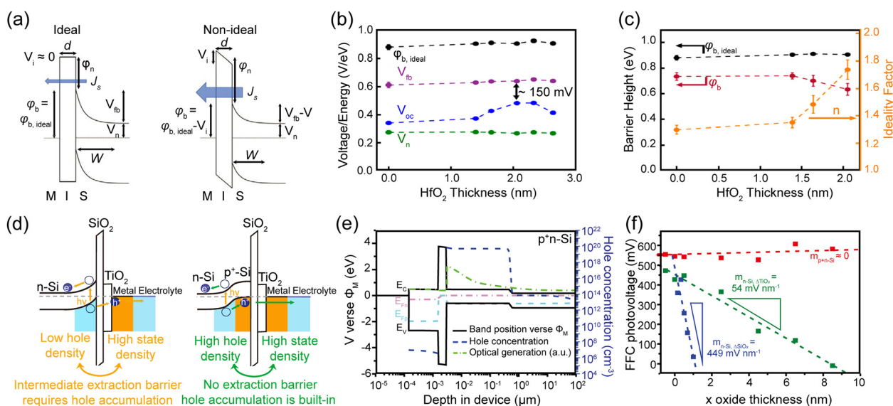
Fig. 18 (a) Energy band diagrams at equilibrium in the dark for an ideal MIS system ( n = 1 , left) and a nonideal MIS system ( n > 1 , right). Reproduced from ref. 265 with permission from John Wiley and Sons, copyright 2020. (b) \phi_{b,ideal} , V_{fb} , V_{oc} , and V_n for Ir/HfO 2 /n-Si photoelectrodes with varied HfO 2 thickness; (c) \phi_{b,ideal} , \phi_b , and n for Ir/HfO 2 /n-Si photoelectrodes with varied HfO 2 thickness. Reproduced from ref. 144 with permission from the American Chemical Society, copyright 2021. (d) Energy band diagrams of MIS-based photoanodes featuring n-Si (left) and p + n-Si (right) semiconductor layers, highlighting the extraction barrier imposed by the insulator layer. (e) Simulated band diagrams of MIS-based photoanodes with a p + n buried junction. (f) FFC photovoltages of the (x + 1.5) nm TiO 2 /~1.3 nm SiO 2 /p + nSi (red squares), (x + 1.5) nm TiO 2 /~1.3 nm SiO 2 /nSi (green squares), and 1.5 nm TiO 2 /(x + 1.3) nm SiO 2 /nSi (blue squares) samples plotted as a function of increasing oxide insulator thickness. Reproduced from ref. 170 with permission from Springer Nature, copyright 2015.
