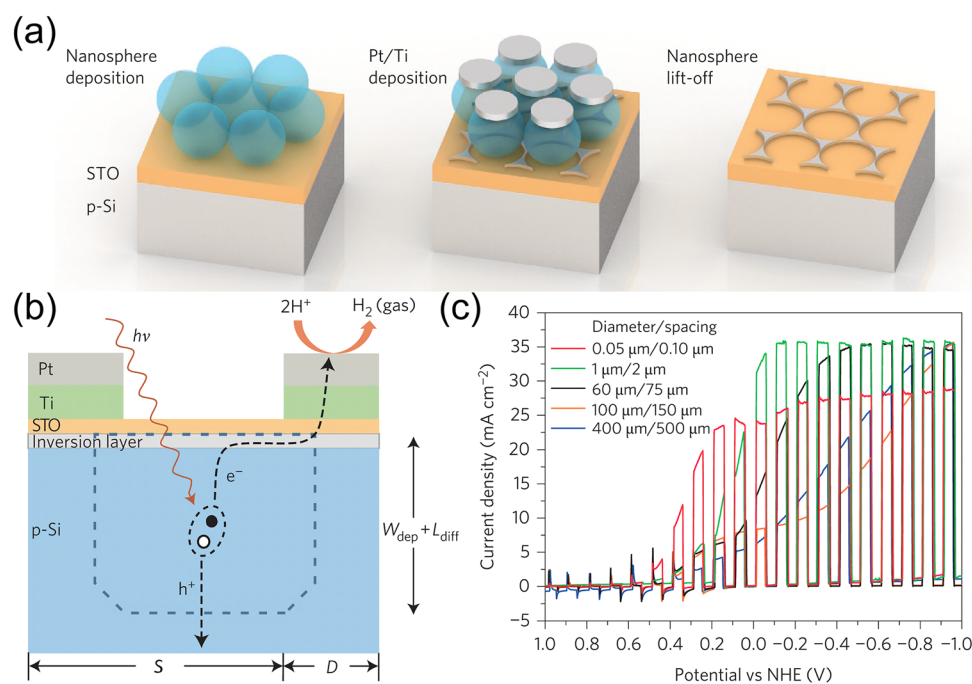
Fig. 10 Nanostructured noble metal cocatalysts in the MIS-based photocathode for the HER. (a) Schematic diagram of the nanosphere lithography process. The sequential steps of nanosphere deposition, Ti/Pt bilayer metal deposition, and nanosphere lift-off from left to right. (b) Schematic diagram of the working mechanism of the p-Si/SrTiO 3 /Ti/Pt photocathode. (c) LSV plots of p-Si/SrTiO 3 /Ti/Pt photocathodes with various cocatalyst feature sizes. Reproduced from ref. 21 with permission from Springer Nature, copyright 2014.
