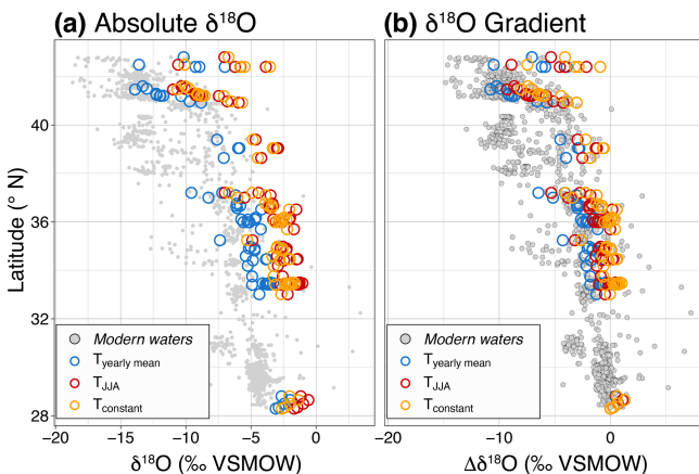
Figure 5. (a) Reconstructed \delta^{18}\text{O}_p plotted against latitude. Reconstructed \delta^{18}\text{O}_p is calculated assuming a spatially uniform temperature of 25 °C (yellow circles), annual mean temperatures (blue circles), or June–July–August (JJA) mean temperatures (red circles). Annual mean and JJA temperatures are taken from monthly long-term mean data retrieved from NARR (Mesinger et al., 2006). Gray circles are modern meteoric water \delta^{18}\text{O} , including groundwater and river or stream water, retrieved from Waterisotopes.org (Waterisotopes Database, 2019). (b) The same as (a) but the x axis sets the southernmost data ( \sim 28^\circ\text{N} ) to zero to emphasize the effect on the spatial gradient in \delta^{18}\text{O} .
