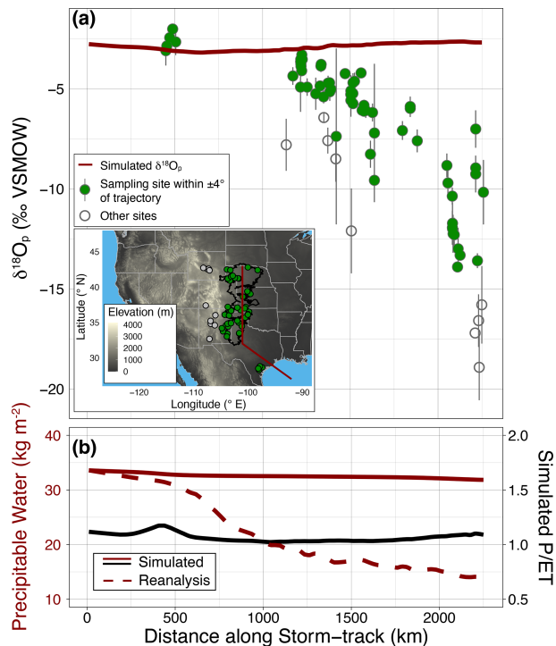
Figure 7. Vapor transport model simulation of \delta^{18}\text{O}_p along an idealized Great Plains low-level jet (GPLLJ) trajectory. (a) The red line is the modeled \delta^{18}\text{O}_p along the simulated storm track (exact location of the storm track is shown as a red line in the inset). Green points are reconstructed \delta^{18}\text{O}_p within \pm 4^\circ longitude of the trajectory. Gray circles are data greater than \pm 4^\circ longitude from the simulated trajectory. Vertical error bars are 1\sigma of the mean section reconstructed \delta^{18}\text{O}_p . (b) Simulated precipitable water (solid red) and P/ET (solid black) plotted along the simulated storm track. The dashed line shows the actual annual mean precipitable water along this storm track retrieved from NARR.
