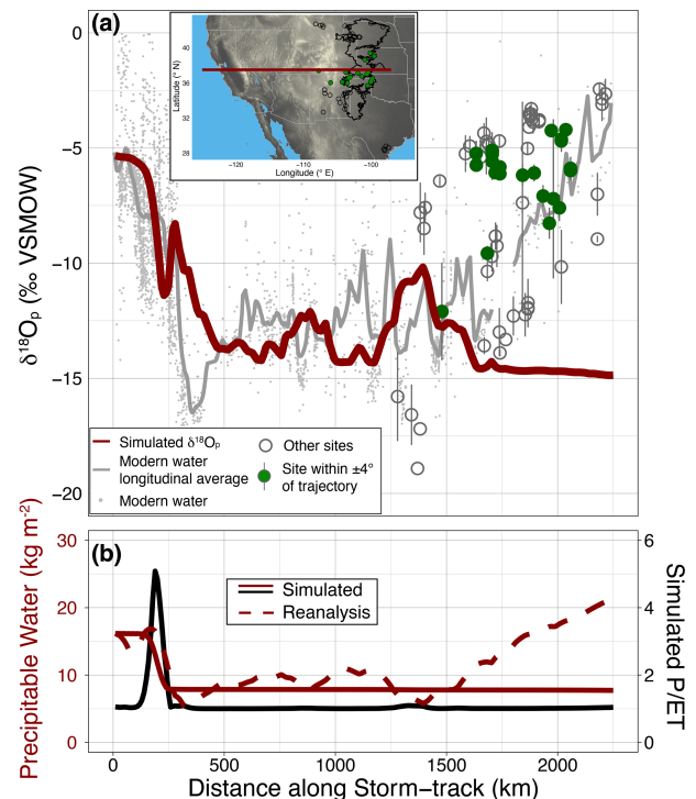
Figure 8. Vapor transport model simulation of \delta^{18}\text{O}_p along an idealized westerly trajectory. (a) The red line is the modeled \delta^{18}\text{O}_p along the simulated storm track (exact location of the storm track is shown as a red line in the inset). Green points are reconstructed \delta^{18}\text{O}_p data within \pm 4^\circ latitude from the storm track. Large, unfilled gray circles are data greater than \pm 4^\circ latitude from the simulated trajectory. Vertical error bars are 1\sigma of the mean section reconstructed \delta^{18}\text{O}_p . Small gray circles are modern meteoric water \delta^{18}\text{O} , including stream water, river water, and groundwater, retrieved from Waterisotopes.org (Waterisotopes Database, 2019). The gray line is a kernel-smoothed average of the meteoric water \delta^{18}\text{O} against distance along the storm track. (b) Simulated precipitable water (solid red) and P/ET (solid black) plotted along the simulated storm track. The dashed line shows the actual annual mean precipitable water along this storm track retrieved from NARR.
