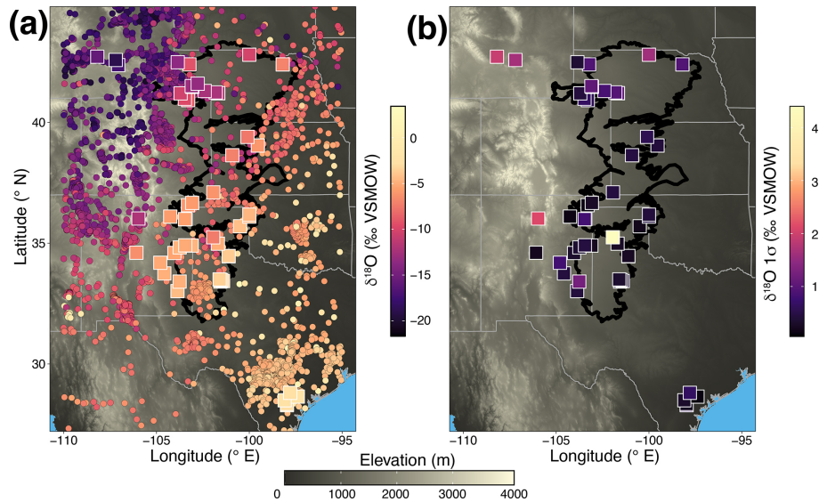
Figure 4. Spatial distribution of \delta^{18}\text{O} (a) and reconstructed \delta^{18}\text{O}_p 1 \sigma (b). (a) Comparison of reconstructed \delta^{18}\text{O}_p from \delta^{18}\text{O}_c (large squares) calculated using the yearly mean of monthly long-term temperature data retrieved from NARR for each site. Modern meteoric water \delta^{18}\text{O} (small circles) is derived from modern groundwater, river water, or stream water retrieved from Waterisotopes.org (Waterisotopes Database, 2019). Data points are colored by their \delta^{18}\text{O} values. (b) The 1 \sigma of the reconstructed \delta^{18}\text{O}_p derived from the variability in the \delta^{18}\text{O}_c values from each stratigraphic section. In both panels, the black polygon marks the extent of modern-day exposure of the Ogallala Formation.
