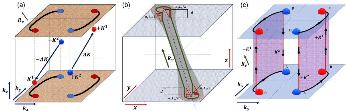
FIG. 1. Schematic picture. (a) k -space illustration of a minimal TWSM. Red (blue) spheres at \pm K^1 ( \pm K^2 ) denote right- (left-)handed WNs, red (blue) discs denote their projections onto the surface Brillouin zone, and black curves are FAs. (b) Real space illustration of the vortex (grey tube) and the semiclassical orbit (green curve). The classical bulk path parallels the tube axis, but quantum tunneling causes deviations near the surface. (c) Semiclassical orbits in mixed real ( z ) and momentum ( k_x, k_y ) space. Each orbit is a closed loop consisting of bulk chiral modes tied to a pair of WNs interspersed by FAs that connect their surface projections.
