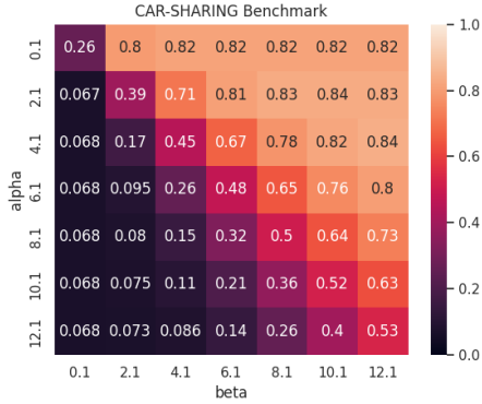
Figure 2: Matching Realization & Planning Distributions, CAR-SHARING Benchmark
