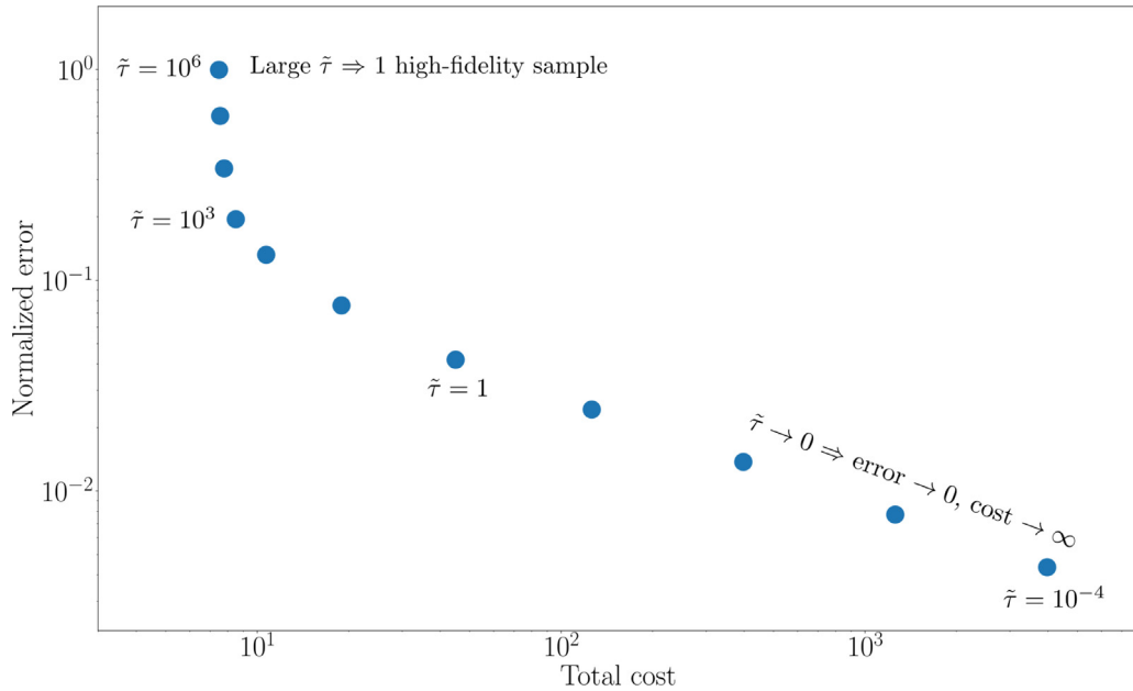
Fig. 6. Pareto-front optimization of MBLBLUE for Problem 2. Here \tilde{\tau} = \tau \|c\|_2 , where \tau is the Pareto parameter from (25) and c is the model cost vector. From right to left, the points in the figure correspond to \tilde{\tau} = 10^i for i = -4, \dots, 6 .
