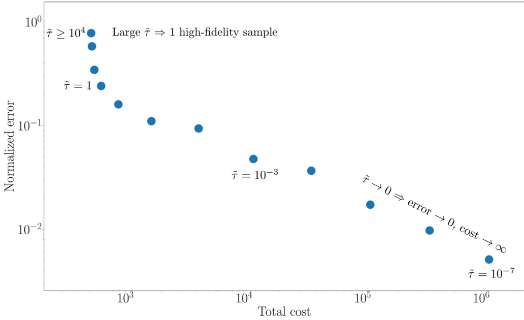
Fig. 4. Points on the Pareto frontier MBLBLUE for Problem 1. Here \tilde{\tau} = \tau \|c\|_2 , where \tau is the Pareto parameter from (25) and c is the model cost vector. From right to left, the points in the figure correspond to \tilde{\tau} = 10^i for i = -7, \dots, 4 .
