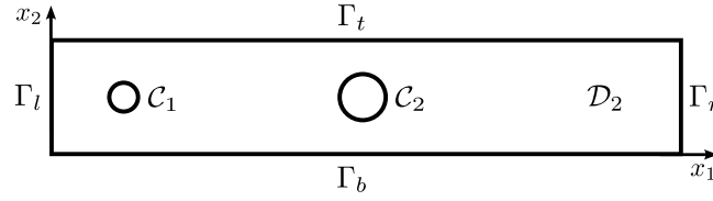
Fig. 1. The domain of Problem 1. The rectangle has length |\Gamma_b| = |\Gamma_t| = 2.2 and width |\Gamma_l| = |\Gamma_r| = 0.41 . The two obstacles C_1 and C_2 have centers at (0.2, 0.2) and (1.0, 0.2) and radii 0.05 and 0.08 respectively. \Gamma_l and \Gamma_r are the inflow and outflow boundaries respectively and the other boundaries are walls.
