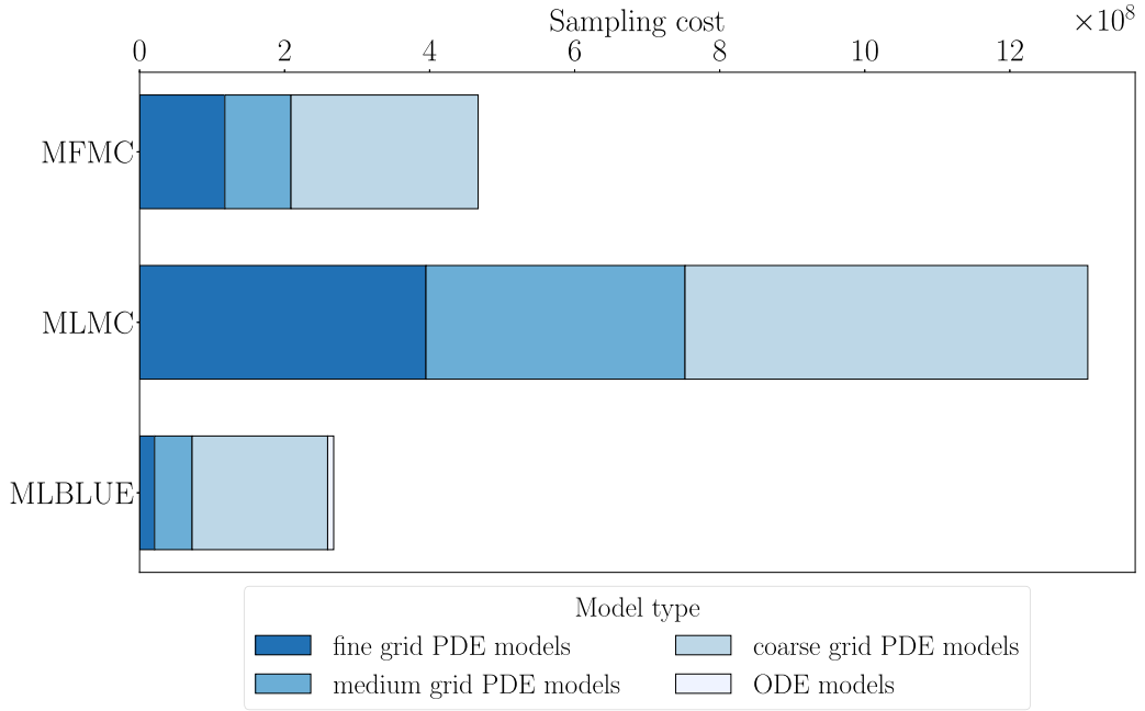
Fig. 5. Total cost of the MOSAP-optimal MLBLUE, MLMC, and MFMC methods for Problem 2. The three darkest colors correspond to the PDE models with darker tints indicating finer grids and timesteps. The lightest color corresponds to the total computational effort spent on all the ODE models. Here we do not distinguish the use of the Hodgkin–Huxley versus the FitzHugh–Nagumo models for the sake of clarity, but we present the detailed sample data in Table 2. (For interpretation of the references to color in this figure legend, the reader is referred to the web version of this article.)
