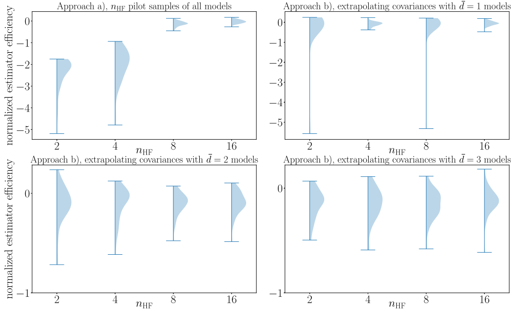
Fig. 7. Half-violin plots of the normalized estimator efficiency (39) for the approaches for Problem 3 described in Section 5.2.1 versus the number of restricted high-fidelity samples n_{\text{HF}} . The light-blue areas depict kernel-density estimates of the probability density function of (39) with respect to \theta . Values close to 0 indicate near-best efficiency. (For interpretation of the references to color in this figure legend, the reader is referred to the web version of this article.)
