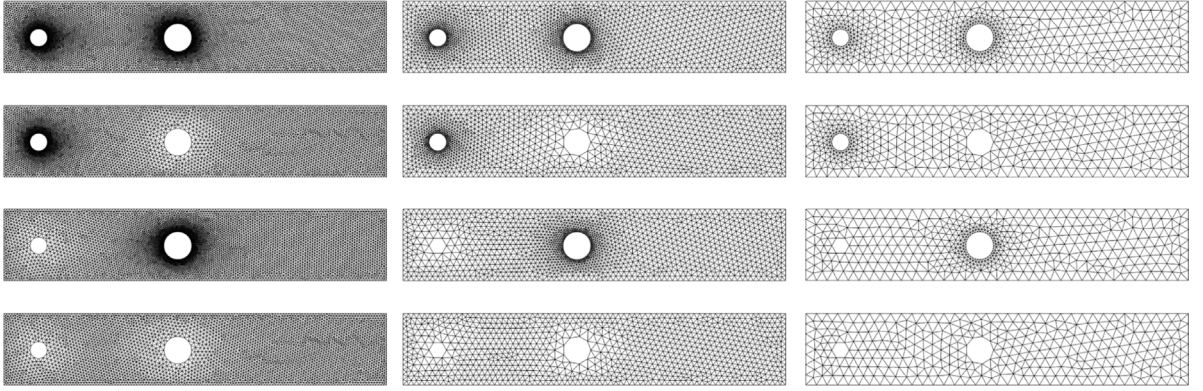
Fig. 2. The grids used to define the twelve models for Problem 1. Each column corresponds to a different “base” mesh: fine (left), medium (center), coarse (right). The actual “base” meshes are in the last row.
