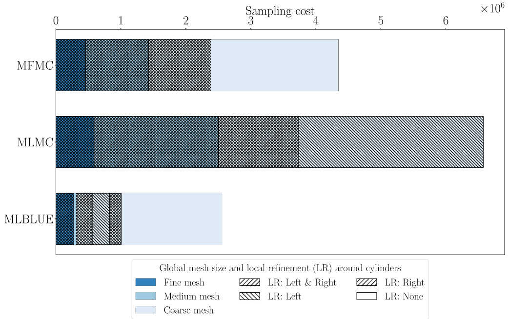
Fig. 3. Total cost of the MOSAP-optimal MLBLUE, MLMC, and MFMC methods for Problem 1. Colors denote the “base” meshes (darker = finer), while the patterns indicate the local refinements around obstacles. (For interpretation of the references to color in this figure legend, the reader is referred to the web version of this article.)
