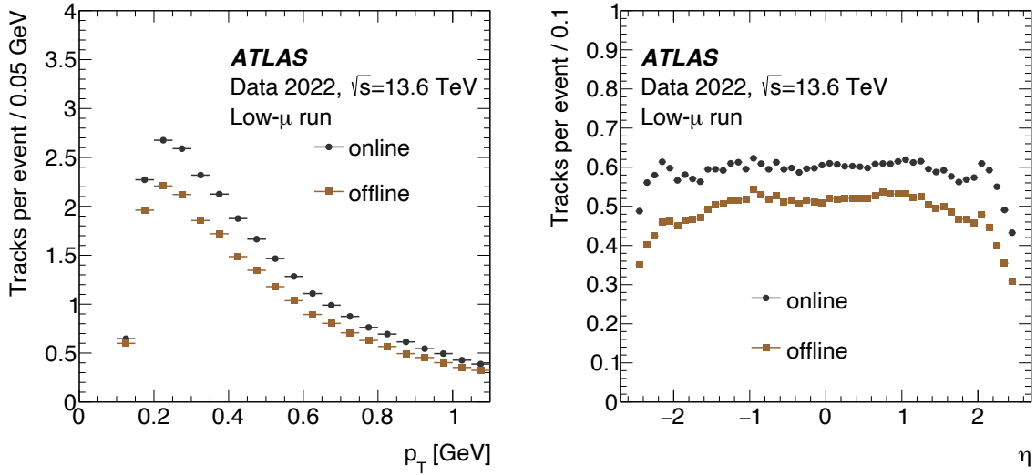
Figure 51. Comparison of (left) p_T spectra and (right) \eta of tracks reconstructed offline and passing minimum-bias quality selection and tracks reconstructed by the HLT online during low pile-up run in 2022.
