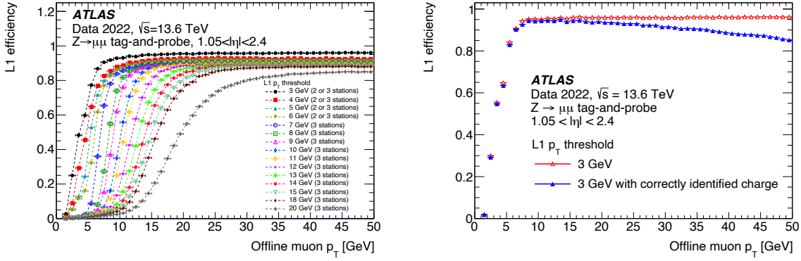
Figure 4. (Left) Efficiency of L1 muon triggers in the endcap region for various p_T thresholds. (Right) The efficiency of the charge identification for L1 muons with p_T > 3 GeV. Only statistical uncertainties are shown.
