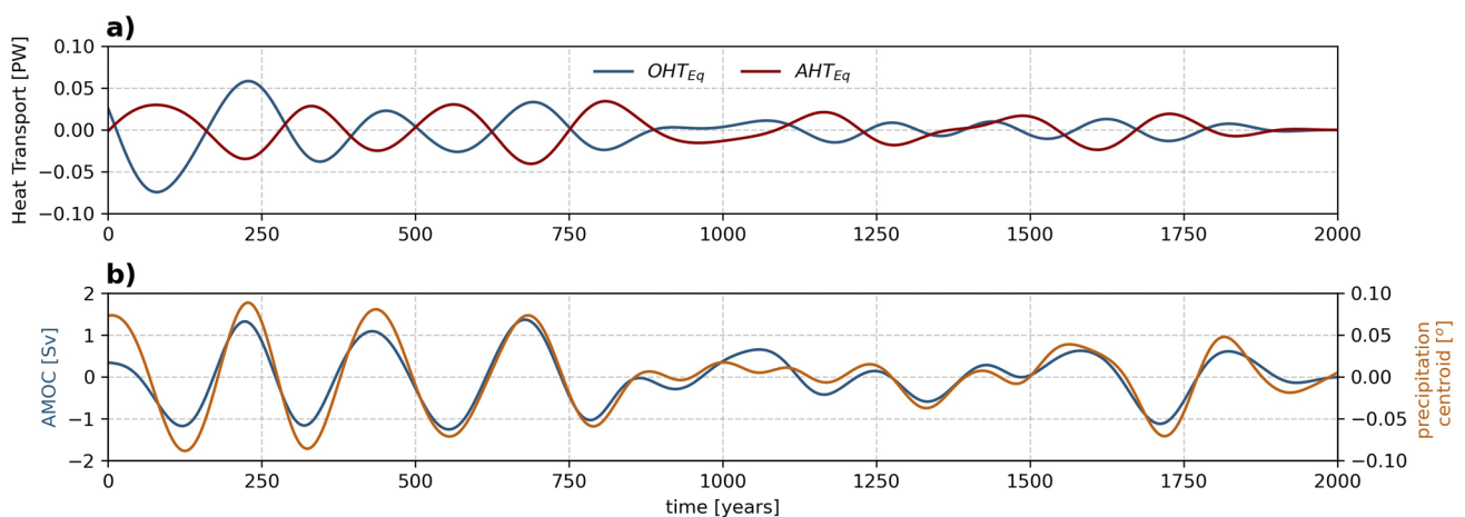
Fig. 7 a Centennial cross-equatorial oceanic and atmospheric heat transport anomalies. Annual mean values were computed before applying the centennial band-pass filter. b Centennial variations in the
