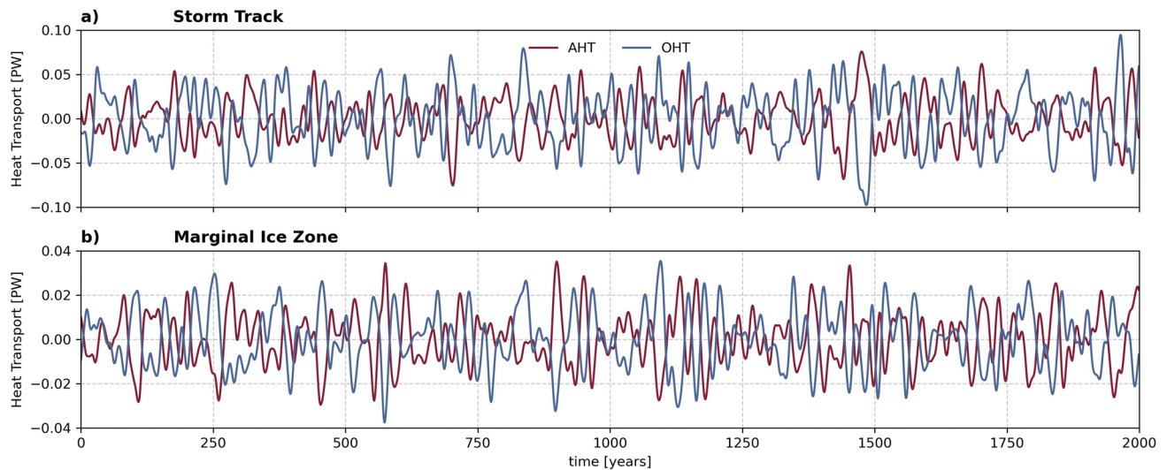
Fig. 3 Time series of ocean and atmosphere heat transport anomalies at the latitudes of the maximum decadal BJC: (a) the storm track region and (b) the marginal ice zone (MIZ). The decadal AMOC
