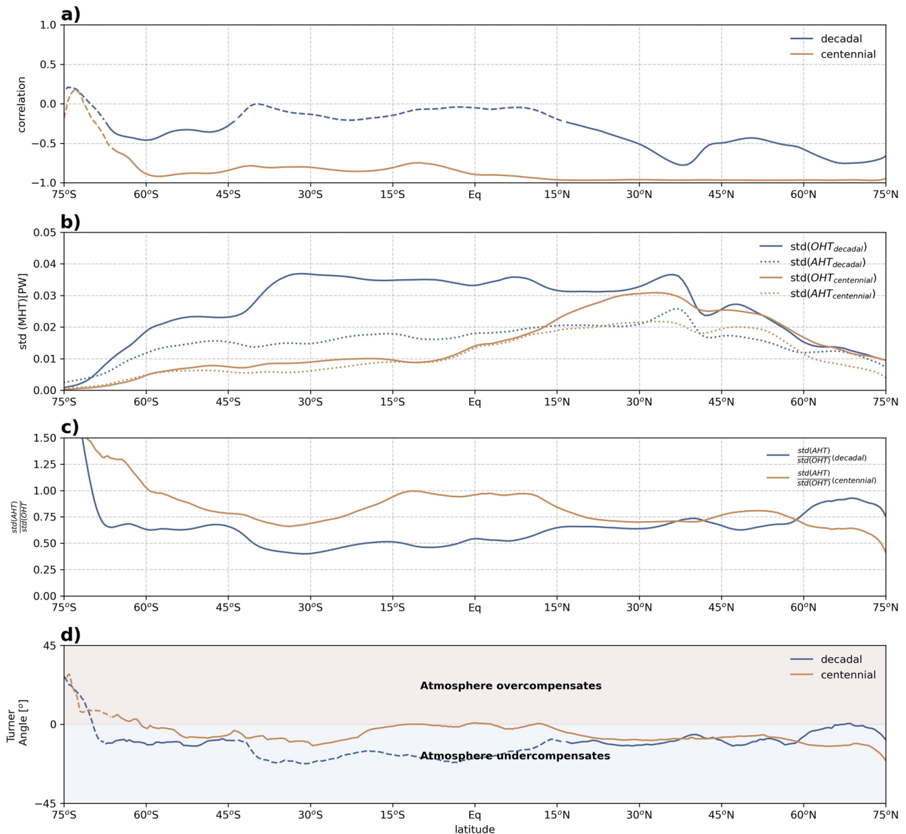
Fig. 2 a Correlations between oceanic and atmospheric heat transport anomalies as a function of latitude. The strongest decadal BJC is found around the storm track region (38°N) and the marginal ice zone, MIZ (67°N). To isolate decadal and centennial timescales a Butterworth bandpass-filter is used with time windows of [10–80] and [80–250] years, respectively. b Standard deviation of AHT (dotted lines) and OHT (solid lines) as a function of latitude. c Ratio of AHT standard deviation to OHT standard deviation. d The time-mean
