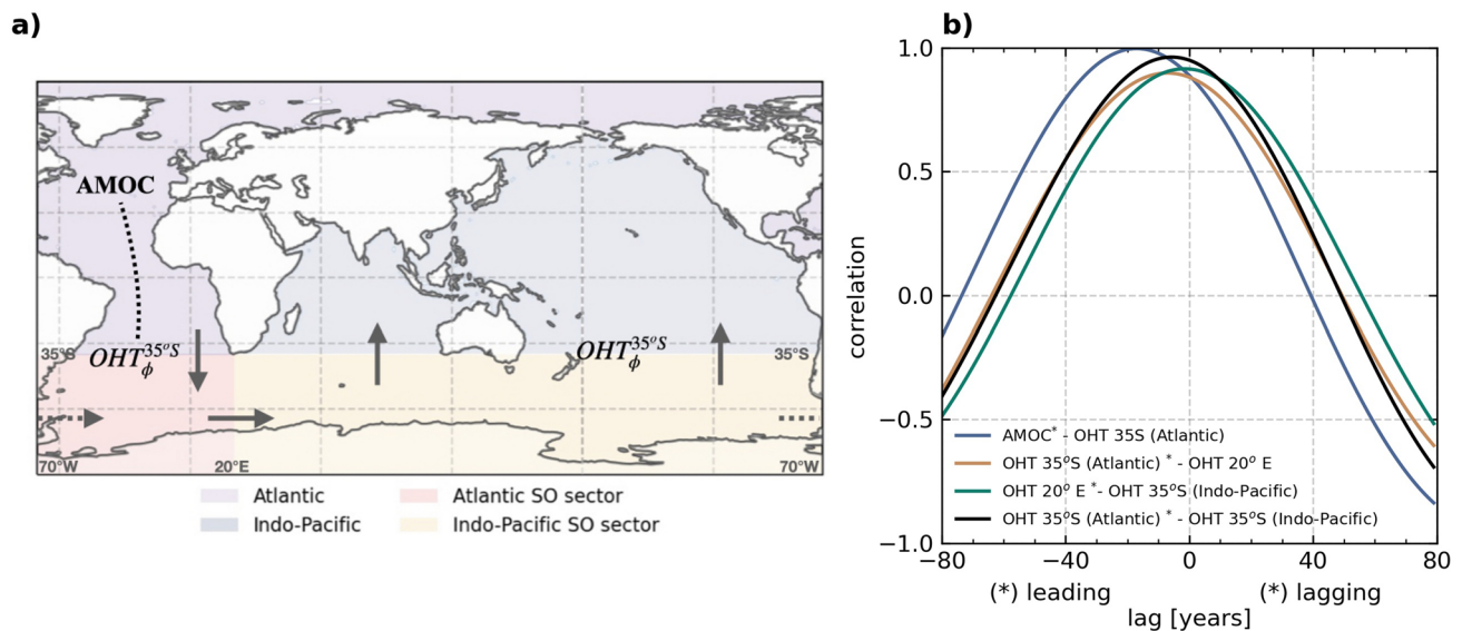
Fig. 10 a A schematics for the centennial Bjerknes-like interbasin compensation. Vertical and horizontal arrows represent anomalous meridional and zonal ocean heat transports between the four regions marked in the figure. b Lead-lag correlations between the correspond-
