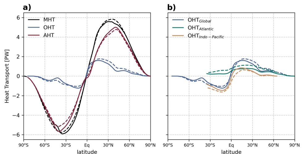
Fig. 1 a Time-mean meridional heat transport components in the IPSL-CM6A-LR model. Black, red and blue curves indicate planetary total, atmospheric and oceanic meridional heat transports (MHT, AHT and OHT, respectively). b Ocean heat transport and its Atlantic and Indo-Pacific components. Dashed lines show heat transport from observation-based data for the period 2000–2016 (Trenberth et al. 2019)
