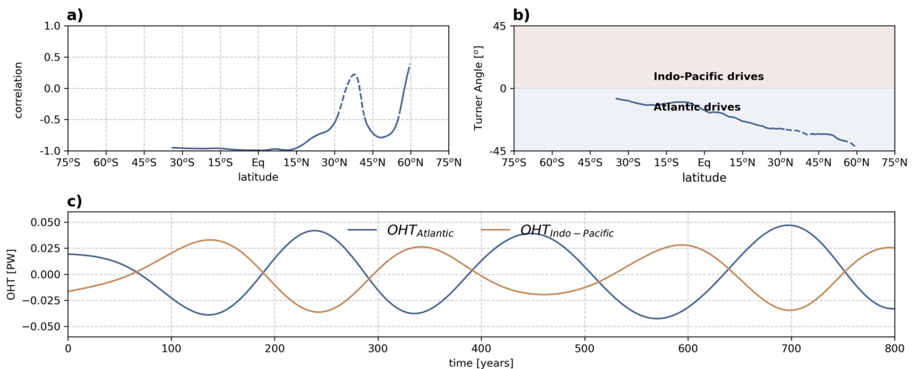
Fig. 8 A Bjerknes-like interbasin compensation (especially pronounced during the strong AMOC variability regime, i.e., years 1–800). a Correlation between Atlantic and Indo-Pacific heat transport anomalies as a function of latitude. b The Turner Angle for Atlantic and Indo-Pacific heat transport anomalies. Shading indicates
