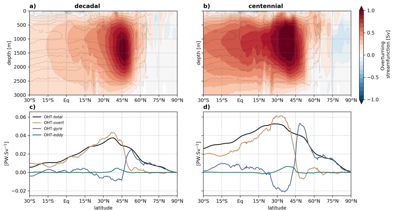
Fig. 4 a, b Regression of Atlantic overturning volume streamfunction onto the AMOC index for years 1–800 (shading, non-dimensional, i.e., Sv/Sv). Note that at centennial timescales AMOC anomalies extend much farther into the Southern Hemisphere. Grey contours
