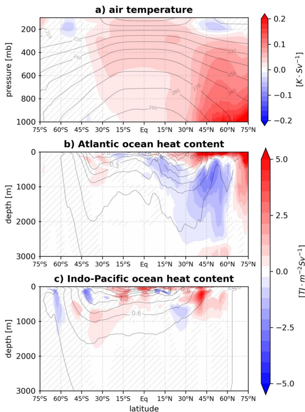
Fig. 5 Regression onto the AMOC index of decadal anomalies of zonally-averaged air temperature (a) and zonally-integrated ocean heat content for the Atlantic (b) and Indo-Pacific (c) for years 1–800 (ocean heat content was integrated from temperature in [°C]). Contours show the time means of the regressed fields (with 10 K contour intervals for the atmosphere, and 0.1 PJ/m 2 for the ocean). Hatched areas indicate significance levels lower than 95 percent according to Student's t -test
