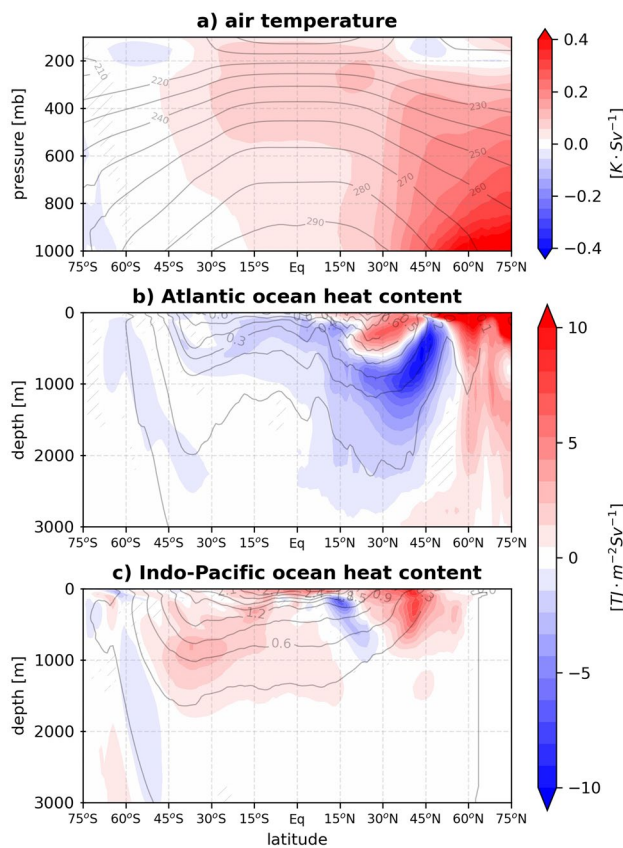
Fig. 6 As in Fig. 5 but for centennial anomalies
