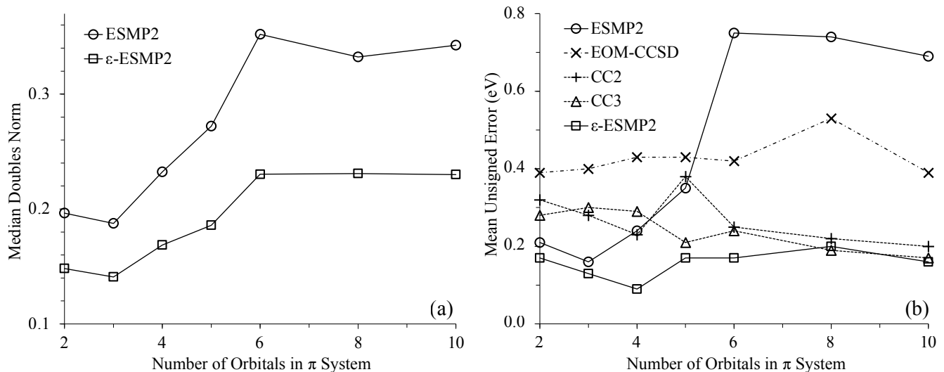
FIG. 1. (a) Median |T_2| doubles norms and (b) MUEs for excitation energies by \pi system size. States identified by ESMP2 to have strongly doubly excited character and states not found by ESMF (red and grey rows in Table I) are excluded.
