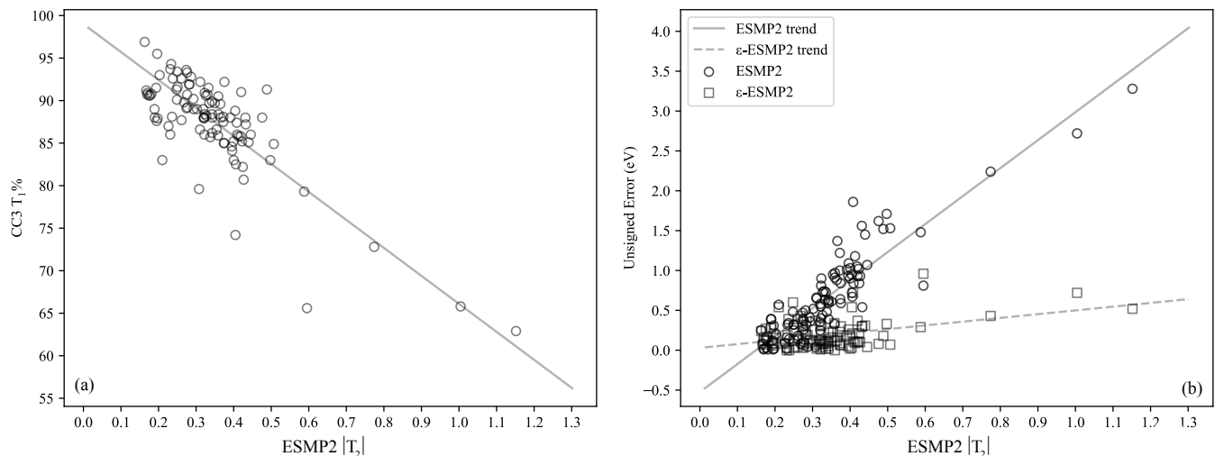
FIG. 2. (a) CC3 T_1 percentages and (b) ESMP2 and \epsilon -ESMP2 unsigned excitation energy errors plotted against the ESMP2 doubles norm |T_2| for all states. The lines are linear fits to the points.
