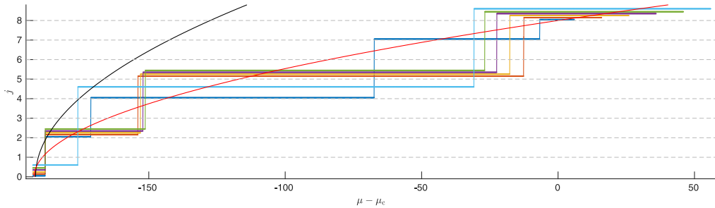
Figure 3. Simulations of (1.1) with initial condition A_*(x;j) , j = 8 and \varepsilon = 0.05 , with initial \mu -values \mu_{\text{in}} = \mu_c + \hat{\mu} , \hat{\mu} = 6, 16, \dots, 56 . Plotted are winding numbers of A as time progresses and \mu decreases, over the parameter value \mu at a given time instance. Trajectories crisscross the Eckhaus boundary in a staircase pattern that depends on the initial parameter value. The value \hat{\mu} = 0 corresponds to the onset of the Eckhaus instability at j = 8 . Initial conditions further away from the instability lead to later drops and higher drop numbers. Fractions of 1 are added to show all itineraries simultaneously, so that the actual current winding number is the largest integer below the plotted curve. Also shown are the boundary of instability (red) and the boundary of existence of equilibria (black) with a given j ; see Section 2 for details. Note that the figure is reflected along the diagonal when compared to Figure 1, using the traditional bifurcation-theoretic depiction of phase-space versus parameter also used in Figure 2.
