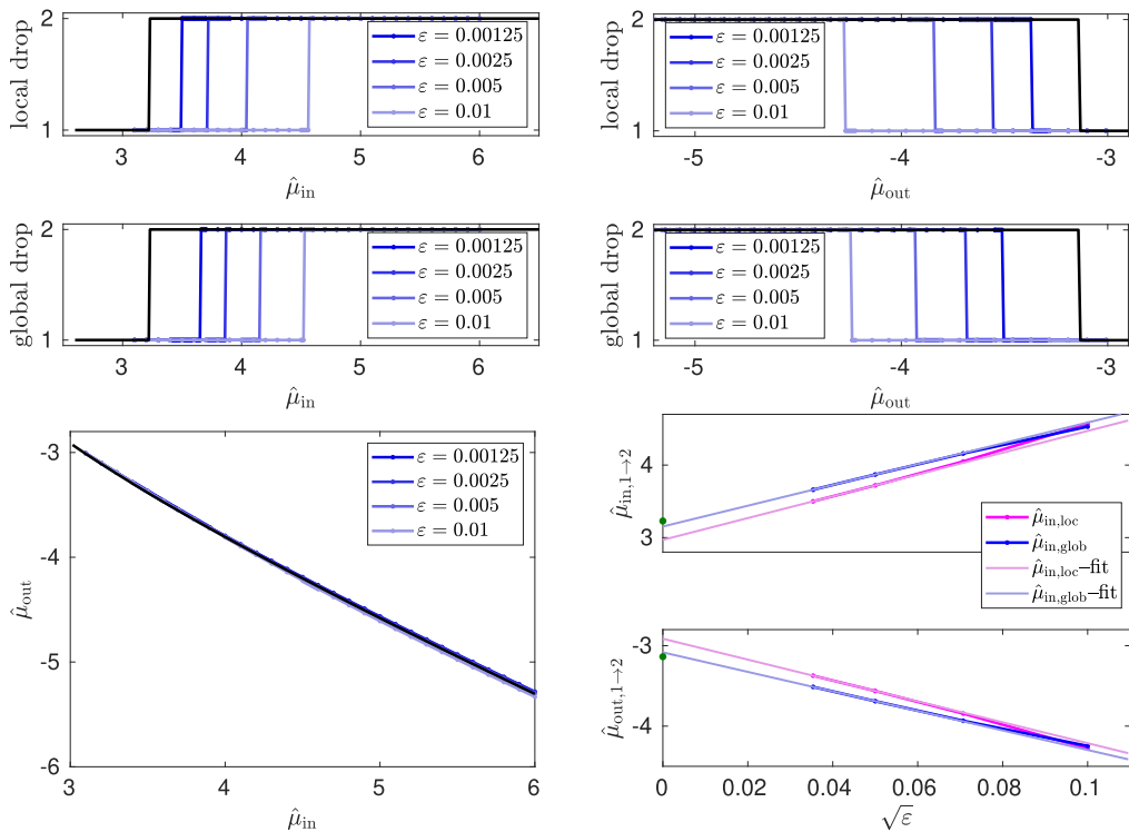
Figure 8. Numerical comparisons for the drop-by-1 to drop-by-2 transition. Top: local and global drop numbers depending on \mu_{\text{in}} (left) and \mu_{\text{out}} (right) for several values of \varepsilon ; predicted drop as solid black curve. Bottom: \mu_{\text{out}} versus \mu_{\text{in}} for several values of \varepsilon together with prediction for \varepsilon = 0 (solid black) (left); drop values \mu_{\text{in}} both local and global as observed in top row shown here as a function of \varepsilon , with linear fit and predicted values of drops as green dot. Extrapolated values at \varepsilon = 0 from linear fits fall within 10% of the predicted value for local drops and within 2% for global drops (right). Throughout, \mu = \mu_c + \hat{\mu} indicates values relative to criticality.
