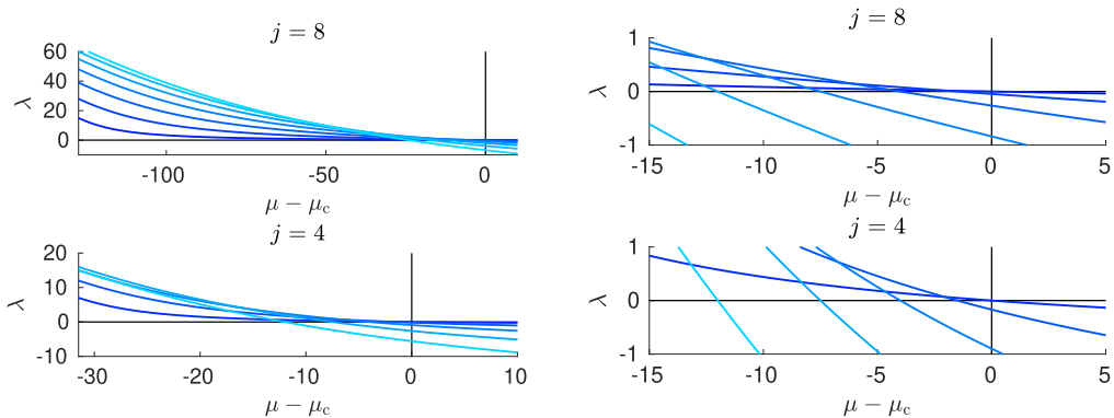
Figure 4. Eigenvalues of the linearisation at E_j with j = 8 (top) and j = 4 (bottom), for parameter values \mu = j^2 at onset to \mu_c + 10 . Enlargement near criticality (right) reveals the intricate crossovers that are explicit in the limit of large j . Eigenvalues are shown from \ell = 1 in dark blue to \ell = 7 (top) and \ell = 5 (bottom), respectively, in light blue.
