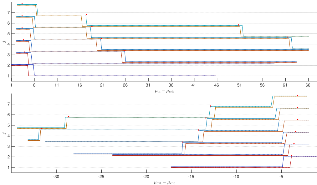
Figure 11. Drop-to numbers for initial patterns with j = 3, \dots, 8 varying \mu_{\text{in}} , plotted against \mu_{\text{in}} - \mu_{\text{c}} (top) and \mu_{\text{out}} - \mu_{\text{c}} (bottom). Shown are both local (blue) and global drops (yellow), which always yield an equal drop or a drop by one less than the local drop. The actual drop-to number is the integer part of the plotted value (which is slightly shifted to improve readability). Red markers indicate the theoretical prediction for drops.
