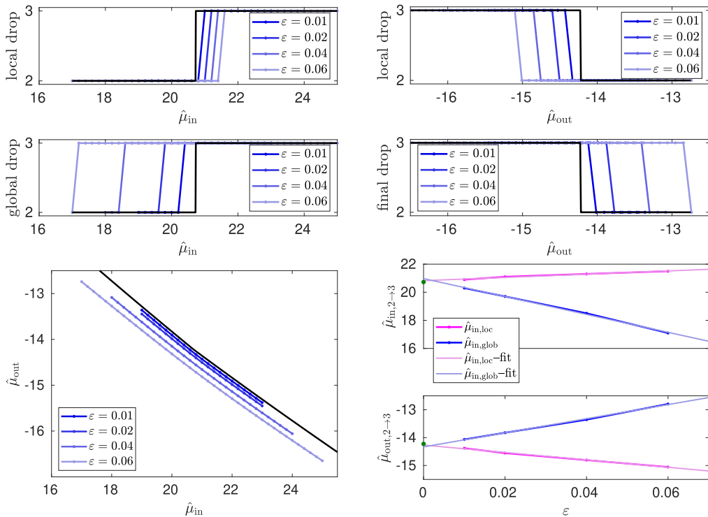
Figure 10. Numerical comparisons for the drop-by-2 to drop-by-3 transition. Top: local and global drop numbers depending on \mu_{\text{in}} (left) and \mu_{\text{out}} (right) for several values of \varepsilon ; predicted drop as solid black curve. Bottom: \mu_{\text{out}} versus \mu_{\text{in}} for several values of \varepsilon together with prediction for \varepsilon = 0 (solid black) (left); drop values \mu_{\text{in}} both local and global as observed in top row shown here as a function of \varepsilon , with linear fit and predicted values of drops as green dot. Extrapolated values at \varepsilon = 0 from linear fits fall within 1% of the predicted value (right). Throughout, \mu = \mu_c + \hat{\mu} indicates values relative to criticality.
