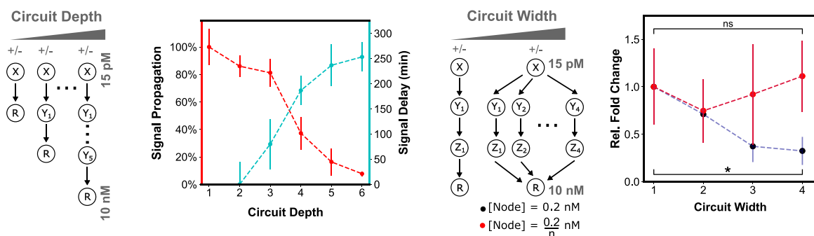
Fig. 3. Engineering deep and wide circuits with high-performing CRISPRa promoters. (A) Schematic of orthogonal CRISPRa/i nodes for use in cell-free circuits. Internal nodes contain an orthogonal scRNA target site and express orthogonal scRNAs. Output nodes contain orthogonal scRNA target sites and express RFP. All nodes contain the same UP element and minimal promoter (HP3). (B) High-throughput characterization of scRNA components in CFS. Left : Plasmids encoding each CRISPRa component are mixed using an acoustic liquid handling robot and expressed in CFS. Right : scRNA-dose-response curves for each node are generated by titrating the amount of scRNA plasmid from 0.5 pM to 5 nM. (C) Comparison of assembly strategies for building a four-layer CRISPRa cascade. Left : Internal node concentrations either decreased from 200 pM to 32 pM as depth increased, were held constant at 200 pM, or increased from 200 pM to 1.25 nM as depth increased. A fourth assembly method was tested in which internal node concentrations were 40, 200, and 170 pM, based on individual scRNA-dose response characteristics. A fifth cascade was included in which the high-performing promoter of the second internal node was replaced with the leaky J2 promoter. Input and output node concentrations were held constant across all strategies at 0 or 15 pM and 10 nM, respectively. Center : Cascade output RFP expression for each assembly strategy with scRNA input (red) and without (black), relative to RFP basal expression. Right : Change in time to maximum expression rate ( \Delta t_{max} ) for each assembly strategy (SI Appendix, Methods S3). (D) Rapid fold change optimization of a four-layer CRISPRa cascade. Left : The first and third internal nodes of the cascade were varied between 40 and 160 pM and 85 and 340 pM, respectively. The input node, second internal node, and output node were held constant at 0 or 15 pM, 0.2 nM, and 10 nM, respectively. Right : Fold change between with and without scRNA input for each CRISPRa cascade. (E) Signal propagation through deep CRISPRa/i circuits. Left : CRISPRa cascades with increasing depth. Input and output node concentrations were held constant across all cascades at 0 or 15 pM and 10 nM, respectively. All of the parallel cascade scRNA outputs are connected to the same RFP node. All node concentrations are tabulated in SI Appendix, Table S5. Right : Propagation efficiency and signal delay are shown as a function of circuit depth (SI Appendix, Methods S3). (F) Construction of wide CRISPRa/i circuits. Left : CRISPRa cascades with increasing width. Input and output node concentrations were held constant across all cascades at 0 or 15 pM and 10 nM, respectively. Right : The concentration of each internal node was held at 0.2 nM as circuit width increased (blue), or the internal node concentration was scaled down proportionally to the width of the circuit (red), such that each internal node concentration is 0.2/n nM, where n is the number of parallel cascades. Fold activation is given relative to a single CRISPRa cascade (SI Appendix, Methods S3). For all panels, values represent the mean \pm SD of three technical replicates.
