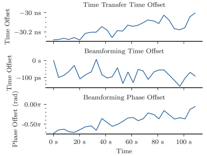
Fig. 3. (Top) Time offset measured between the two systems \Delta_{0n} after coarse synchronization using GNSS PPS. We estimate \Delta_{0n} using a TWTT exchange, and correct for it by delaying the samples at node 1 accordingly. (Middle) Time offset of the beamformed signals after delay correction using (2). (Bottom) Phase offset measured at the beamforming target after delay correction using (2). Although the system clocks skew by \sim 280 ps over the duration of the experiment, the beamforming signal only varies by at most 160 ps.
