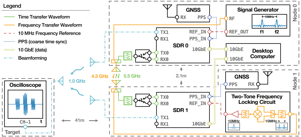
Fig. 1. System schematic showing target node (left), and distributed array nodes 0 and 1 (top and bottom, respectively). Node 0 held the coordination computer running GNU Radio which was connected via 10 GbE to each node for control. Node 0 also contained the signal generator for frequency reference which generated a 10 MHz two-tone waveform at 4.3 GHz to be transmitted to the two-tone frequency locking circuit on node 1 used to lock SDR 1, as well as generated the 10 MHz frequency reference for the SDR on node 0. Each node also contained a GNSS receiver for coarse initial time synchronization between platforms (only used once on initialization). Finally, channel 0 on each SDR was connected to a transmit-receive switch to be controlled via timing synchronization pulse direction which was connected to the 8-dBi log-periodic time-frequency transfer antennas, and channel 1 on each SDR was connected to a 10-dBi log-periodic beamforming antenna.
