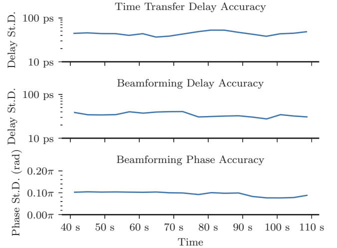
Fig. 4. Time standard deviation measured between the two systems (top) and time and phase standard deviation measured at the beamforming target (middle and bottom).
