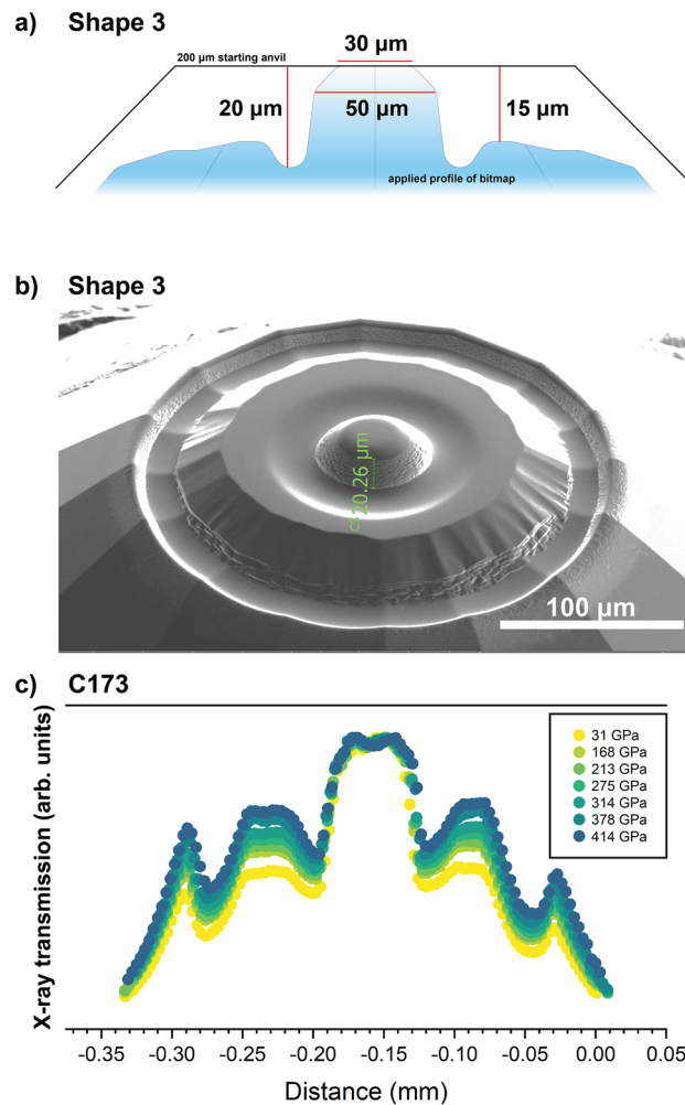
Figure 1. (a) General schematic of the toroidal Shape 3 tested in this study on sample C173. The profile of the starting 200 \mu\text{m} standard anvil is included. The idealized bitmap profile, shaded in blue was scaled to 250 \times 250 \mu\text{m} , such that the outer shoulder overlaps with the pavilion of the standard anvil. A sharp edge is produced at the boundary of the bitmap and is an artifact of the differing slopes between the bitmap and the diamond pavilion. (b) Example of the toroidal anvil Shape 3 milled with the focused ion beam showing the real profile that results from milling onto the pavilion and the sharp outer lip produced by the bitmap slope that is offset onto the pavilion. (c) Absorption scan of sample C173 with Shape 3 between 30 and 414 GPa measured at the center of the sample chamber based on the Pt scale 24 .
