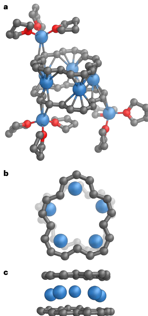
Fig. 3 | Single-crystal X-ray structure of 1^{4-}\text{Li}_4 . a , The asymmetric unit (interstitial solvent, hydrogen atoms and minor disorder components omitted for clarity) with C–Li distances in the range 2.175(4)–2.745(4) Å (internal ions) and 2.285(3)–2.591(4) Å (external ions) indicated by thin tubes. b , c , Two orthogonal views on the sandwich part: top view ( b ) and side view ( c ). Colour code: C, grey; O, red and Li, blue.
