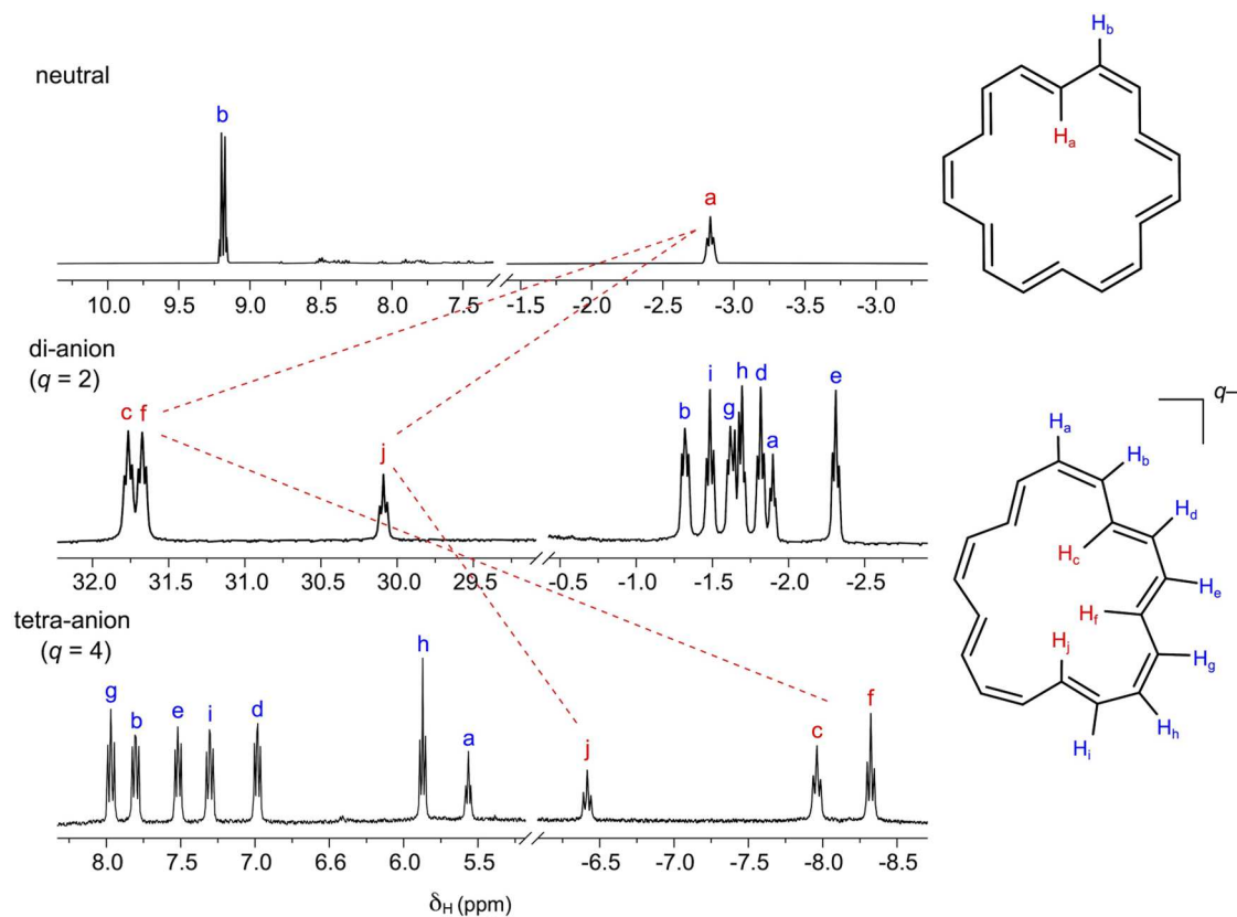
Extended Data Fig. 1 | Overview of ^1\text{H} NMR spectra. Comparison of the ^1\text{H} NMR spectra of neutral 1 (THF- d_8 , 500 MHz, -40^\circ\text{C} ), di-anion 1 · \text{Li}_2 (at -60^\circ\text{C} ) and tetra-anion 1 · \text{Li}_4 (at -40^\circ\text{C} ). All spectra in THF- d_8 , 500 MHz.
