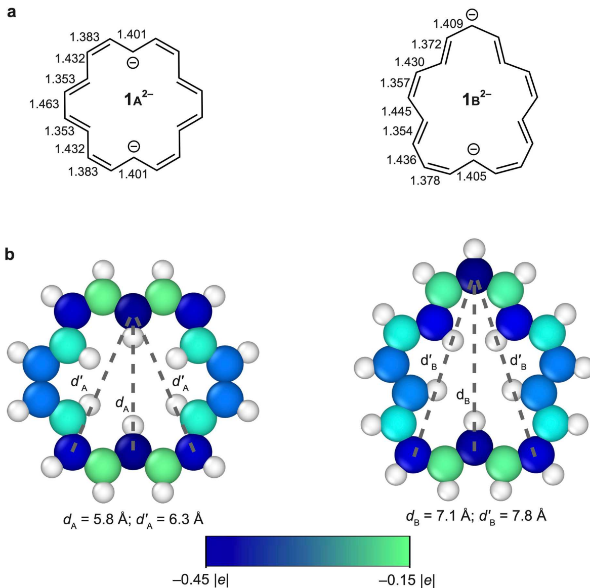
Extended Data Fig. 4 | Bond lengths, charge distributions and trans-annular distances in two geometries of the dianion. a Bond lengths and b NBO charges in 1A 2- (left) and 1B 2- (right) calculated at the BLYP45/def2-TZVP level. Dark blue corresponds to −0.45 |e|, light green to −0.15 |e|. Distances between atoms with the largest negative charge are highlighted.
