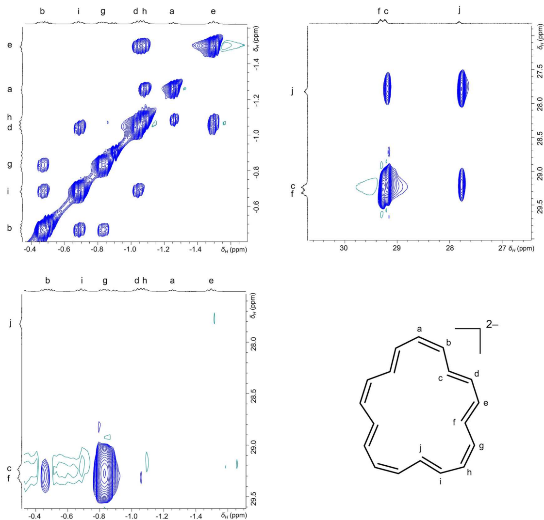
Extended Data Fig. 2 | Fragments of the ^1\text{H} - ^1\text{H} EXSY spectrum of in-situ generated di-anion 1 - \text{K}_2 . This spectrum characterizes the dynamic exchange processes in 1 - \text{K}_2 ( \text{THF}-d_8 , -70^\circ\text{C} , 500 MHz, mixing time 0.0 sec).
