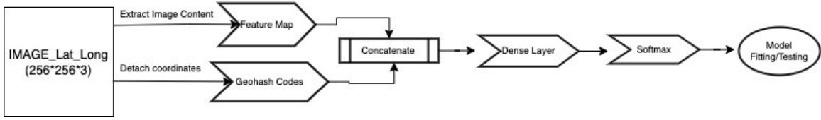
Figure 2: An illustration of the architecture obtained by integrating geohash codes into the CNN (including pretrained models) architecture.
