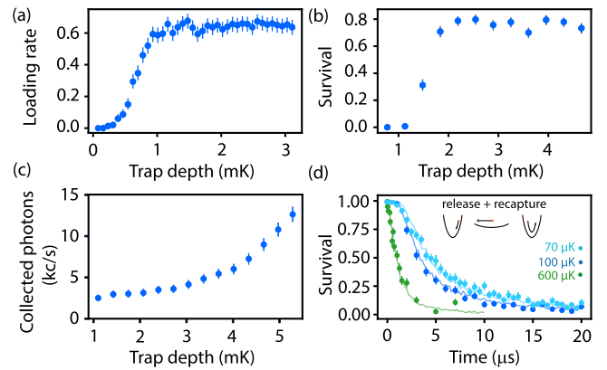
FIG. 3. Properties of ^6\text{Li} in a tweezer. (a) Atom loading vs trap depth (mK). For imaging, trap depth is ramped to a constant value of 3.4 mK. (b) Survival vs trap depth after 533 consecutive image cycles. (c) Photons collected vs trap depth during 15 ms image. In (b) and (c), \Lambda -GM parameters are not changed as a function of trap depth. (d) Release-and-recapture survival probability under different cooling scenarios. Light blue: optimized cooling for low temperature. Dark blue: optimized cooling for survival. Green: hold in tweezer for 1 s (no cooling light applied). Solid lines are Monte Carlo simulations used to extract a temperature.
