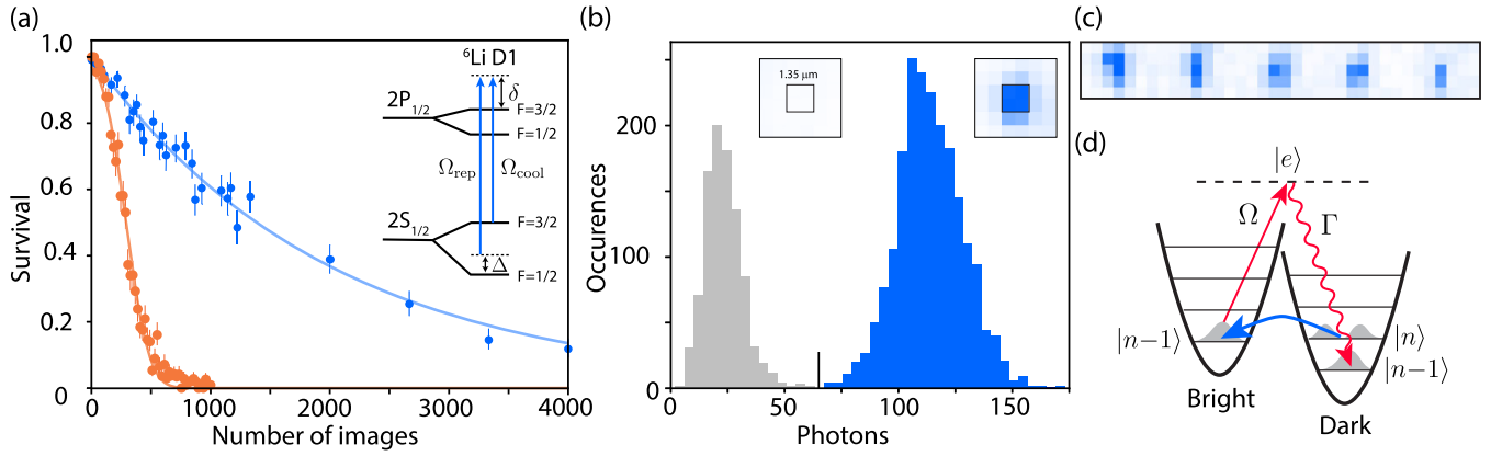
FIG. 1. Low-loss \Lambda -GM imaging of ^6\text{Li} . (a) Atom survival in an optical tweezer with (blue) and without (orange) active cooling light vs consecutive images. The data with continuous GM cooling have a 1/e decay time of 30.0(8) s, corresponding to 2000 images. The atom without active cooling light applied is heated due to off-resonant scattering of the tweezer light and has a 1/e time of 5.13(7) s. The inset is the D1 level structure with \Lambda -GM parameters labeled. (b) Histogram of fluorescence from a single ^6\text{Li} atom trapped in a 1064 nm optical tweezer. This histogram represents an averaged image (3000 shots) of a single region of interest with a signal threshold of 65 photon counts and a loading rate of 0.68(3). Fitting a Gaussian distribution to both peaks and integrating the 0 atom (1 atom) fraction above (below) the signal threshold gives an imaging fidelity of 0.999 7(2). The insets show the cropped region of interest of an image of 0 (left) or 1 (right) atom. (c) Single-shot image of five occupied adjacent tweezer sites. (d) Simplified picture of \Lambda -GM in a tweezer. A dark state |D, n\rangle couples to the bright state |B, n-1\rangle with one less motional quanta. Spontaneous emission then pumps the population to the dark state |D, n-1\rangle when in the Lamb-Dicke regime.
