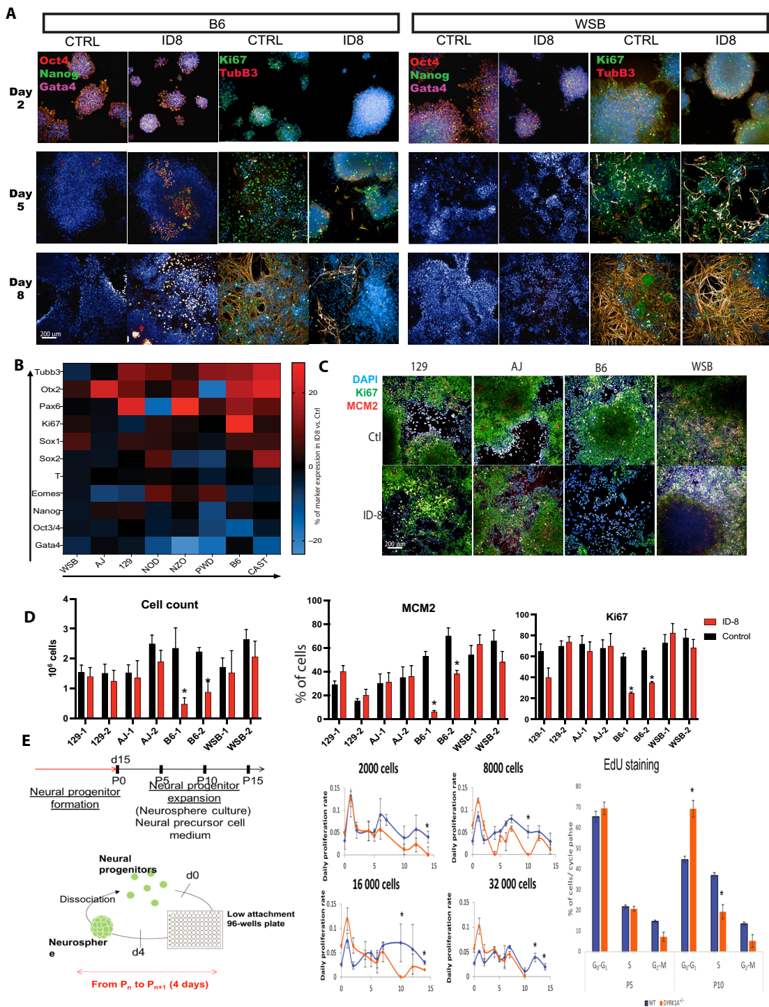
Fig. 5. DYRK1A inhibition differentially blocks neural progenitor proliferation in a strain-dependent fashion. (A) Representative images of the B6 and WSB mESC lines differentiated into NPC in the presence of the DYRK1A inhibitor ID-8 and analyzed at days 2, 5, and 8. (B) Comparison between the proportion of cells expressing the indicated markers as measured by HCS in control and ID-8–treated cells after 8 days of differentiation. Red indicates decreased percentage of cells expressing the associated marker in ID-8–treated cells compared to control, whereas green means an increase. Cell lines and markers are arranged according to the overall degree of change (arrows), and n = 4 biological replicates. (C and D) Images and plots representing the cell count of proliferating NPCs derived from six independent cell lines different from those used in (B). NPCs were cultured with or without ID-8 for five passages. B6 showed a decreased number of cells and proliferative markers (Ki67 and MCM2) compared to its control, whereas 129, AJ, and WSB were not affected. n = 4 . *Statistically different from its control, P < 0.05 . Kruskal-Wallis and Dunn’s test were conducted. (E) Long-term proliferation assay in hPSC-derived NPC. Left: Experimental design [cells were kept in proliferative conditions as neurospheres for 15 passages (2 months total)]. Middle: Cell numbers over time. Right: Percentage of cells in each cycle phase measured by EdU staining in WT and DYRK1A +/- . Experiment shows that DYRK1A +/- NPC undergo quiescence faster than control. Two-tailed t test, n = 4 , * P < 0.05 .
