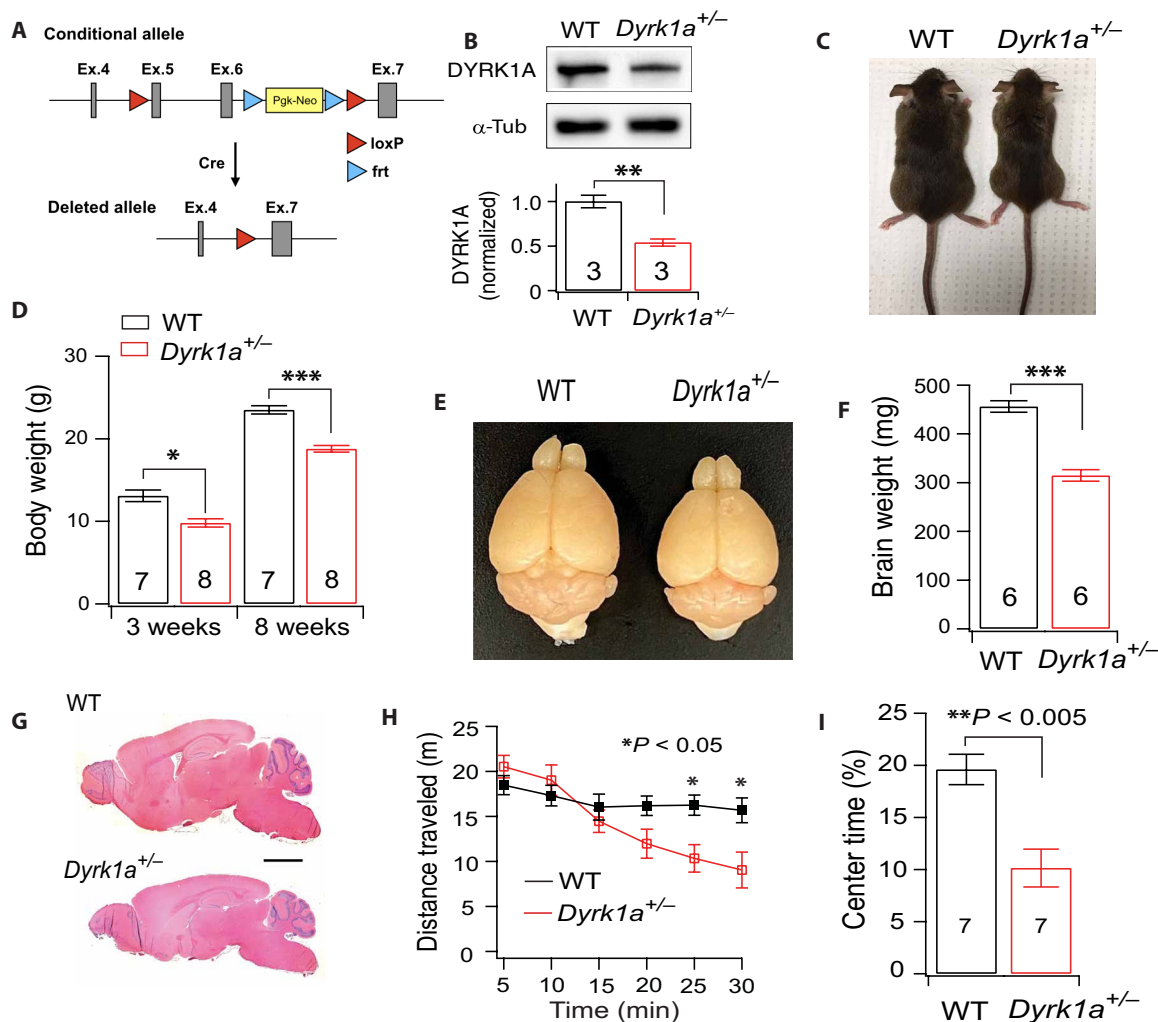
Fig. 10. Heterozygous deletion of Dyrk1 in mice confirms strain-dependent sensitivity observed in vitro. (A) Generation of the null allele of Dyrk1a using a conditional Dyrk1a allele and constitutively expressed Cre. Exons 5 and 6 of Dyrk1a , which encode part of the kinase domain, are flanked by loxP sites. The germline CMV Cre driver removes exons 5 and 6 and the Pkg-Neo selection cassette and causes a frameshift. (B to I) Phenotype of Dyrk1a heterozygotes in B6/129 background. (B) Western blot of cortical tissues from WT and Dyrk1a +/- mice. α-Tub, α-tubulin. (C) A Dyrk1a +/- mouse and a WT littermate at 12 weeks of age. (D) Body weight of male mutant and control mice at 3 and 12 weeks of age. (E) Brains of a control and mutant at 12 weeks of age. (F) Brain weights of mutant and control mice at 12 weeks of age. (G) Sagittal brain sections from a WT and Dyrk1a +/- mouse at 3 months of age. Scale bar, 2 mm. (H) Distance traveled by Dyrk1a +/- ( n = 7) and WT ( n = 7) mice per 5 min in an open field apparatus. (I) Percentage of time spent at the center of the arena. * P < 0.05, ** P < 0.01, and *** P < 0.001.
