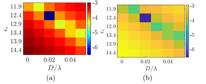
FIG. 8. Logarithm of mean value of the cost function comparing noisy data for D = 0.02\lambda_0 and \epsilon_r = 12.4 and noiseless data for (a) object translation and (b) phase scanning of the structured field. Cost function minimum was obtained at the correct value of separation and dielectric constant within a margin of \lambda_0/100 for separation and 0.5 for dielectric constant.
