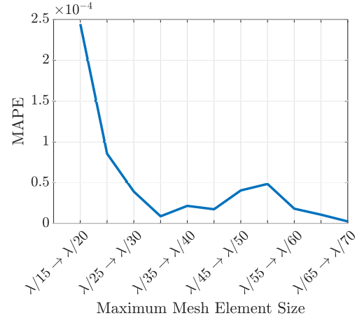
FIG. 12. Mean absolute percent error (MAPE) in g_p(\Delta\gamma_y; D) when decreasing the maximum mesh element size, calculated one speckle field (the same one used in Fig. 10(a)). Parameter values of D = 0.01\lambda_0 and \epsilon_r = 4 were used. Any decrease in the maximum mesh element size beyond \lambda/25 resulted in a MAPE less than 0.0001%, so our chosen maximum size of \lambda/40 is clearly sufficient for numerical convergence.
