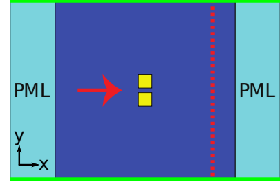
FIG. 9. Adaptation of the geometry shown in Fig. 2 for use with a speckle field, which is incident from the left. The left and right boundaries are still 2\lambda_0 -thick PMLs, but the top and bottom boundaries (green) have been replaced with continuous periodic boundary conditions.
