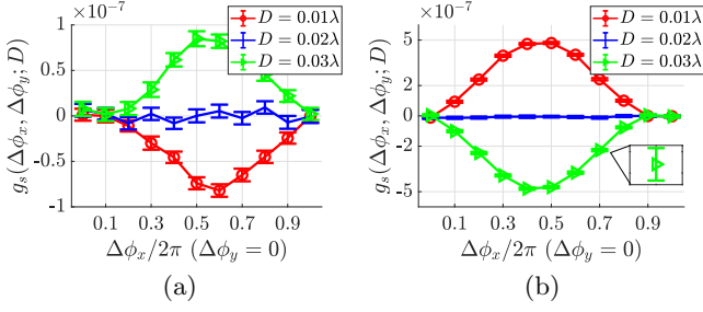
FIG. 3. Resolution performance for the arrangement in Fig. 2 with phase scanning of the structured field. The reference separation is D_0 = 0.02\lambda_0 . The object in (a) has \epsilon_r = 1.5 , and in (b) has \epsilon_r = 4 . The error bars are generated empirically using an SNR of 54.1 dB. Separation changes of 0.01\lambda_0 are easily distinguished with far-field data. When \epsilon_r is increased, this distinguishability increases as well.
