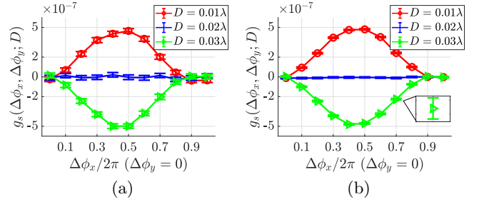
FIG. 5. Effect of detector noise for the arrangement in Fig. 2 with phase scanning of the field and \epsilon_r = 4 . The error bars were generated using an SNR of (a) 49.1 dB and (b) 54.1 dB. Other simulation parameters are similar to Fig. 3. The relationship between SNR and distinguishability is explored further in Sect. II E.
