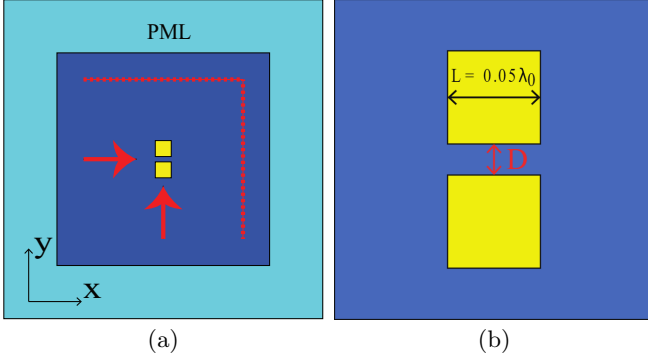
FIG. 2. (a) The free-space simulation domain is a square 6\lambda_0 on a side and bounded by a 2\lambda_0 -thick PML on all sides. Two dielectric scatterers are placed in the center, forming an object with separation D to be resolved. The red arrows indicate the direction of propagation of the incident plane waves. The dotted red lines represent the detector arrays, which measure the normal component of the time-average Poynting vector (intensity). (b) The central region is enlarged to show the scatterers of side L = 0.05\lambda_0 and separation D . These figures are not drawn to scale, in that the object size is larger than that used in the simulations, given the detector arrangement presented (with this size of the objects, the detectors would be located farther away than shown).
