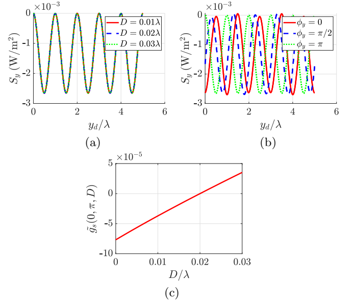
FIG. 13. Detailed information about the measurements underlying Sect. II. (a) Poynting vector incident upon the y detector at different positions, for varying D . The change in intensity is small compared to the background. y_d/\lambda represents the position on the y detector plane normalized in terms of wavelength. (b) Similar, but for a changing field position instead. The measurement is laterally translated. (c) Measured power difference for a fixed field position, but more separation values D , and having been divided by the background intensity according to (B1). This illustrates required detector sensitivity.
