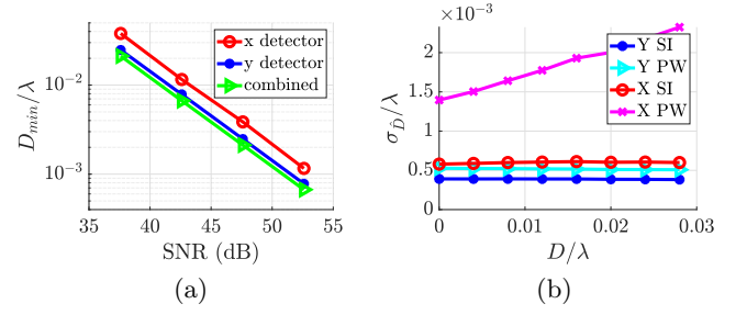
FIG. 7. Minimum scatterer separation distinguishable with 2\sigma certainty as a function of combined detector SNR, and comparison between Cramér-Rao bounds for estimating D with plane-wave illumination versus standing-wave illumination. Both sub-figures are scaled in terms of \lambda , and use \epsilon_r = 4 . (a) Minimum scatterer separation distinguishable from D = 0 with 2\sigma certainty as a function of SNR for three detector plane configurations with structured illumination. (b) Square root of the CRB variance of \hat{D} as a function of D for plane-wave illumination (in each direction, and over the corresponding detector plane) and structured illumination (over the each detector plane). 52.6-dB SNR. SI: structured illumination, PW: single-plane-wave illumination, y: y detector plane, x: x detector plane.
