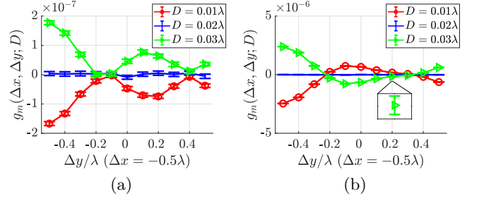
FIG. 4. Similar to Fig. 3, but a stationary field and moving object are used for comparison. \Delta y was varied in steps of 0.1\lambda_0 from -0.5\lambda_0 to 0.5\lambda_0 , while \Delta x was fixed at -0.5\lambda_0 . As in Fig. 3, the object in (a) has \epsilon_r = 1.5 , and in (b) has \epsilon_r = 4 . Despite the different shapes of the curves, it is still the case that the separation between the curves increases with \epsilon_r .
