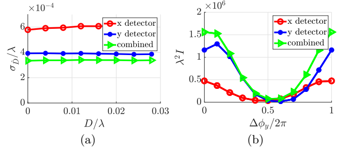
FIG. 6. Cramér-Rao bound and Fisher information for estimating D from power flow through the detector plane, scaled in terms of \lambda . \epsilon_r = 4 for both sub-figures. (a) Square root of the CRB variance of \hat{D} as a function of D for three detector plane configurations, using data corresponding to 11 values of \Delta\phi_y . (b) Fisher information as a function of \Delta\phi_y for three detector plane configurations at D = 0.02\lambda .
