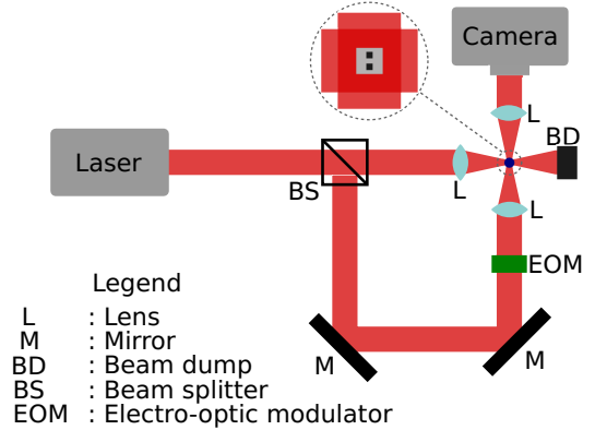
FIG. 14. Conceptual diagram for a possible experimental adaptation. A laser is focused onto a structured sample, and an electro-optic modulator translates the field along one direction by modulating its phase.
