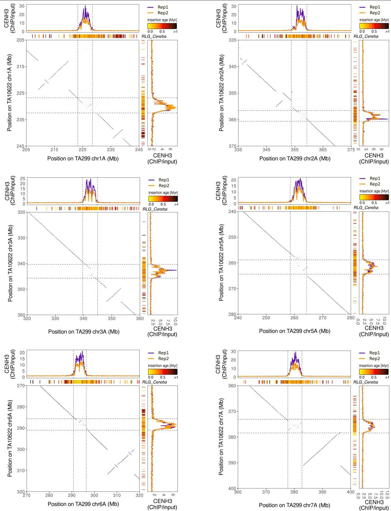
Extended Data Fig. 6 | Dot plot comparisons of centromeric and peri-centromeric regions of T. monococtum accessions TA299 (horizontal) and TA10622 (vertical). Aligned with the dot plots are plots of the average coverage
