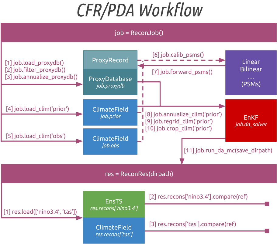
Figure 5. The cfr workflow for the last millennium reanalysis (LMR; Hakim et al., 2016; Tardif et al., 2019) paleoclimate data assimilation (PDA) framework. Here “nino3.4” and “tas” stand for two examples of the reconstructed variables for validation, referring to the El Niño–Southern Oscillation index series calculated as the spatial average of surface temperature within the tropical Pacific region (5° N–5° S, 170–120° W) and the surface temperature field, respectively. PSMs is for proxy system models, and EnKF is for ensemble Kalman filter.
