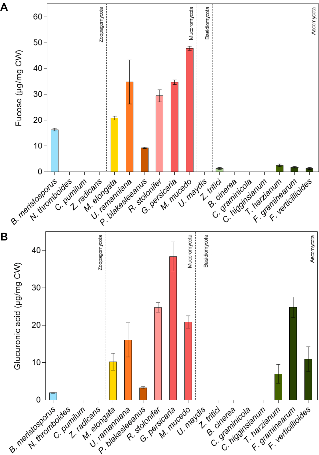
Fig. 6. Amount of fucose and glucuronic acid in the cell wall of selected fungal species. Data (µg/mg cell wall dry weight) represent mean ± S.D. of (A) fucose and (B) glucuronic acid from 4 independent measurements.
