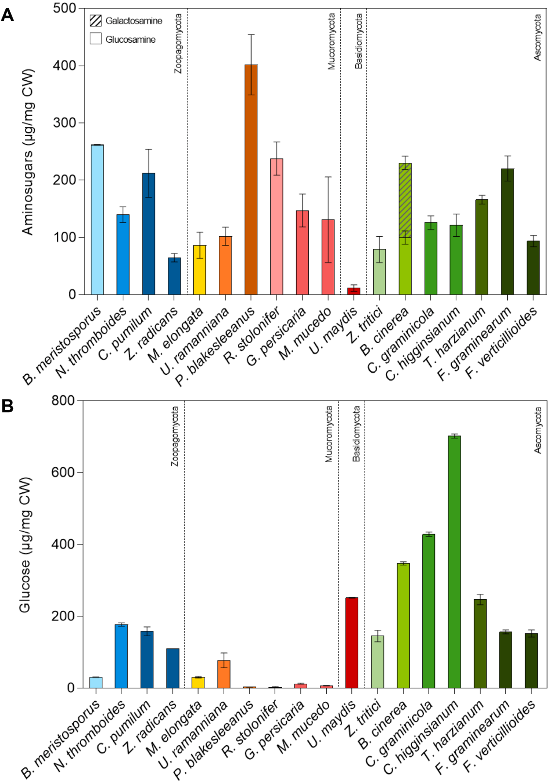
Fig. 4. Amount of glucosamine, galactosamine and glucose in the cell wall of selected fungal species. Data (µg/mg cell wall dry weight) represent mean ± S.D. of (A) glucosamine and galactosamine and (B) glucose from 4 independent measurements.
