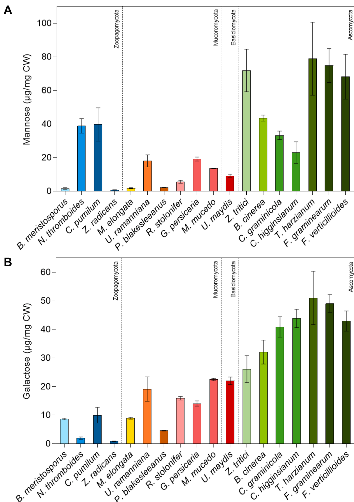
Fig. 5. Amount of mannose and galactose in the cell wall of selected fungal species. Data ( \mu\text{g/mg} cell wall dry weight) represent mean \pm S.D. of (A) mannose and (B) galactose from 4 independent measurements.
