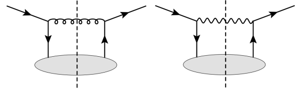
FIG. 1. Nonperturbative matrix elements that lead to a semihard quark annihilating off a resolved soft antiquark in the medium and producing an on-shell gluon (left) or photon (right).
