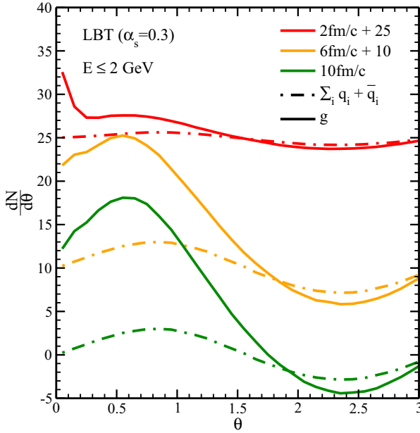
FIG. 9. Particle number distribution from LBT simulation starting from a E_{\text{in}} = 25 GeV gluon and evolving in a static medium at T = 0.25 GeV, as a function of the polar angle, for soft partons with energy E \leq 2 GeV. The gluon distribution is displayed in full lines, while the sum of quarks and antiquarks is displayed in dashed lines, at three evolution times of 2, 6, and 10 fm/c.
