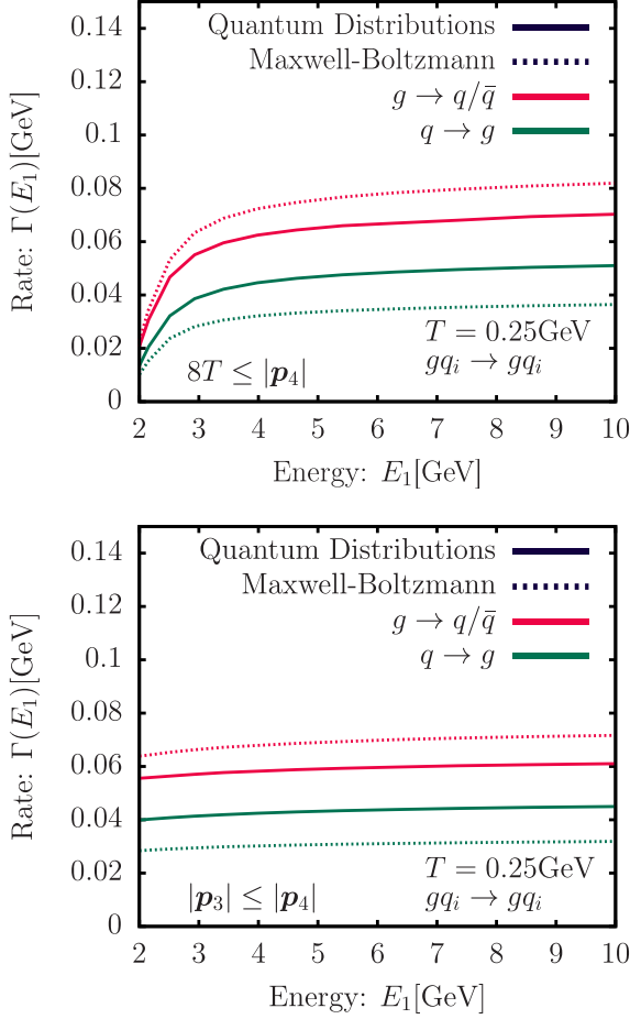
FIG. 6. QCD Compton scattering. The rate of gluon conversion into quark (or antiquark), Eq. (11), is represented in red lines, while the reverse process from Eq. (10) is displayed in green lines. Kinematic selections are employed for the momentum p_4 of the semihard parton with opposing flavor, in the top panel 8T \leq |p_4| or |p_3| \leq |p_4| in the bottom panel. While the dashed lines represents the rate where the equilibrium distributions are taken to be the classical Maxwell-Boltzmann distribution, the rates computed using the equilibrium distribution from quantum statistics are shown in the full lines.
