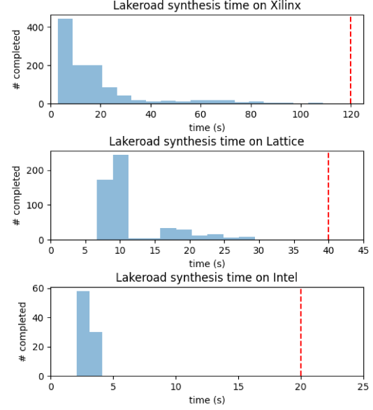
Figure 7. Histograms of Lakeroad program synthesis run-time for all terminating (success or UNSAT) Lakeroad experiments described in Section 5.1, with timeout thresholds indicated with a vertical dotted red line.
