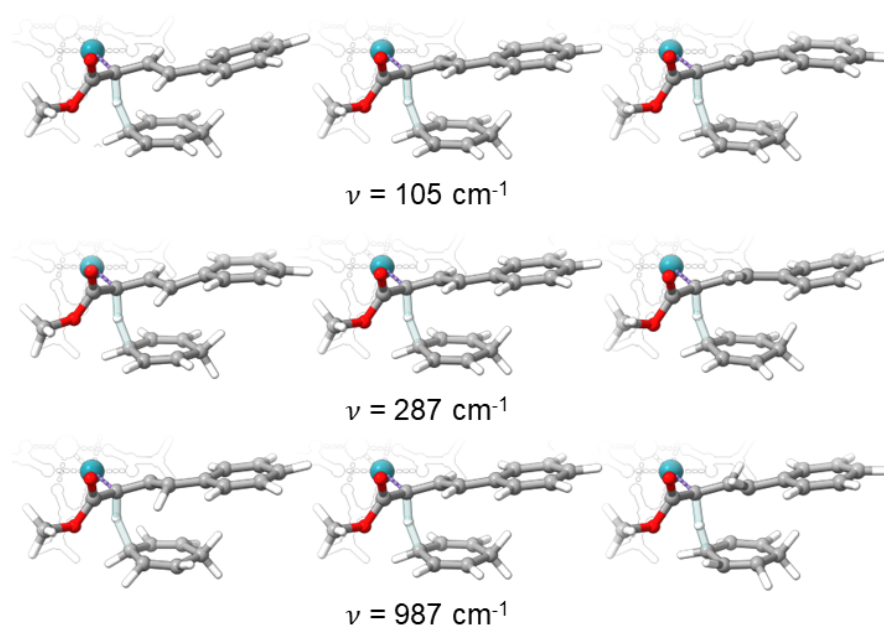
Figure 6. 3D static images showing the key vibrational modes in s-trans TS1 that contribute to Cope C-C bond motion.
