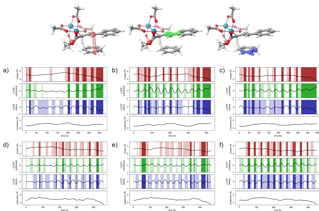
Figure 7. Plots of key coordinates for the Cope and insertion reaction for two different MD simulations starting from s-trans TS1 . a-c plot of key coordinates for a trajectory that resulted in the Cope product. d-f plot of key coordinates for a trajectory resulting in the insertion product. Red regions highlight when the Cope C-C bond length is decreasing. Green areas highlight when the carbonoid carbon for the Cope product is bending away from the diene. Conversely, blue areas highlight when the Cope carbon on the diene is bending away from the carbonoid. Darker regions are when all three of these happen simultaneously.
