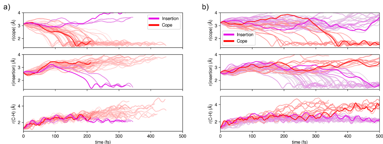
Figure 5. a) Plot of key distances (in Å) versus time (in fs) for forward progress during trajectories starting at s-cis TS1. b) Plot of key distances (in Å) versus time (in fs) for forward progress during trajectories starting at s-trans TS1. R(\text{cope}) and r(\text{insertion}) are the C-C distances for the atoms involved in forming the corresponding product. R(\text{C-H}) is the breaking C-H bond length.
