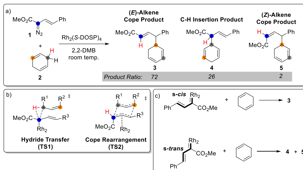
Scheme 1. a) Outline of Rh-catalyzed combined allylic C-H activation/Cope rearrangement reaction between styryldiazoacetate 1 and 1,4-cyclohexadiene 2 reported by Davies. 34 b) Depiction of the hydride transfer transition state TS1 and Cope rearrangement transition state TS2 . c) Comparison of s-cis and s-trans conformations of the reactive rhodium carbenoid and the proposed reaction products.
