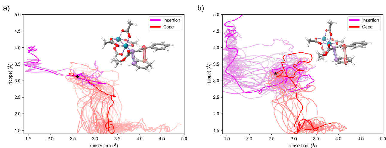
Figure 4. Left: Plot of 41 trajectories proceeding in the forward direction beginning at s-cis TS1 . Right: Plot of 43 trajectories proceeding in the forward direction beginning at s-trans TS1 . The star represents the transition-state structure position. R(\text{cope}) and r(\text{insertion}) are the corresponding C-C distances that lead to each of these products. Purple colored lines represent trajectories that ended in a C-H insertion product and red colored lines represent trajectories that ended a Cope product.
