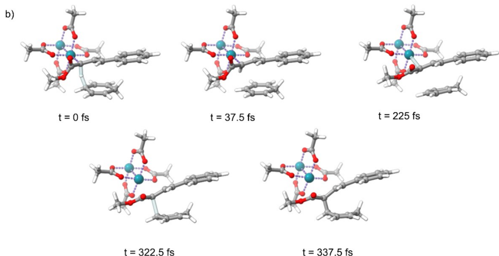
Figure 3. a) Snapshots from a dynamic reaction coordinate analysis starting from s-cis TS1 and proceeding in the forward direction. b) Snapshots from a dynamic reaction coordinate analysis starting from s-trans TS1 and proceeding in the forward direction.
