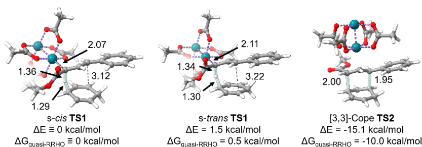
Figure 2. M06/def2-SVP optimized transition-state structures for C-H cleavage ( s-cis TS1 and s-trans TS1 ) and Cope rearrangement ( TS2 ). Distances in Å. Quasi-RRHO free energies are calculated at 298.15 K with 100 cm -1 as the damping parameter. 40 Energies are reported at the M06/def2-TZVP//M06/def2-SVP level of theory.
