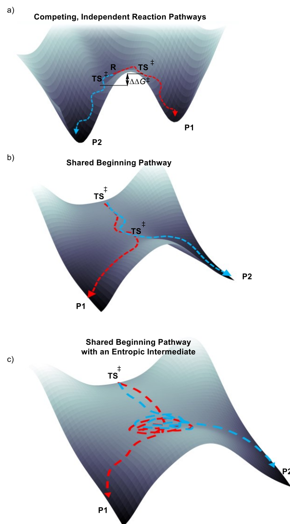
Figure 1. a) Illustration of a reaction where there are two independent reaction pathways leading from an intermediate (I) to products P1 and P2 . In this scenario the energy difference between the two transition states ( TS ) can be used to statistically model and understand the P1 versus P2 selectivity. b) Illustration of a potential-energy surface with two consecutive transition states, which is often referred to a post-transition state bifurcation because the surface divides between the two transition states. c) Illustration of a potential-energy surface with two consecutive transition states and a roaming, entropic intermediate that occurs en route to forming either P1 or P2 .
