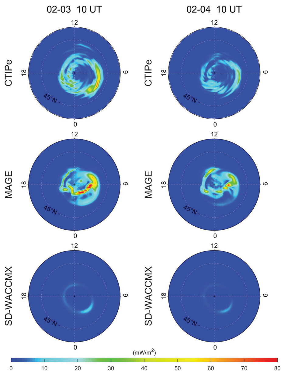
Figure 12. The height-integrated Joule heating in Northern Hemisphere simulated by the Coupled Thermosphere Ionosphere Plasmasphere Electrodynamics Model, Multiscale Atmosphere-Geospace Environment, and SD-WACCMX at 10:00 universal time on 03 February (the left panels) and on 04 February (the right panels). The patterns are plotted in latitude versus local time coordinates. The white dashed line represents the 45° latitude boundary in Northern Hemisphere.
