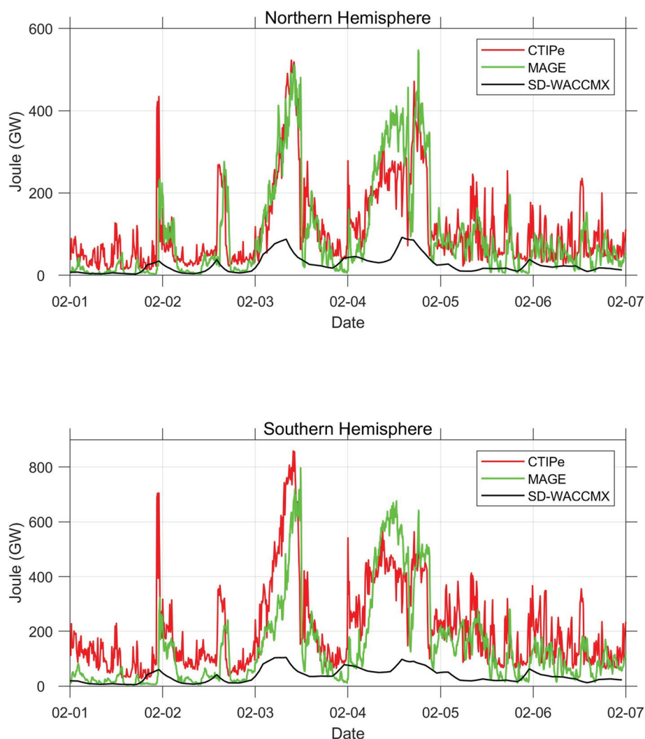
Figure 11. The integrated high latitude Joule heating rate poleward of 45^\circ in both the northern hemisphere (the top panel) and southern hemisphere (the bottom panel) simulated by the Coupled Thermosphere Ionosphere Plasmasphere Electrodynamics Model (red), Multiscale Atmosphere-Geospace Environment (green), and SD-WACCMX (dark).
