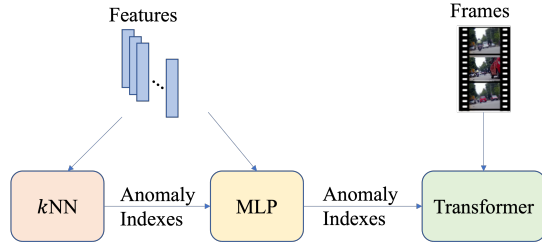
Figure 3. Self-supervised structure of REWARD.
