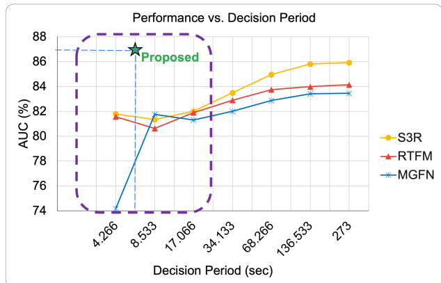
Figure 1. Performance drop in state-of-the-art methods with decreasing decision period. The proposed method (shown with star) significantly improves timely detection performance with 86.94% AUC and 6.4 sec decision period.
