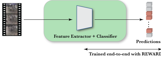
Figure 2. Proposed approach simplifies and outperforms the popular wVAD approaches which only train the feature encoder and classifier networks in an ad hoc manner. End-to-end training of feature extractor in our approach provides compactness and superior real-time performance.
