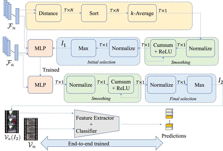
Figure 5. Proposed REWARD network for self-supervised end-to-end training of large video models in wVAD problems.
