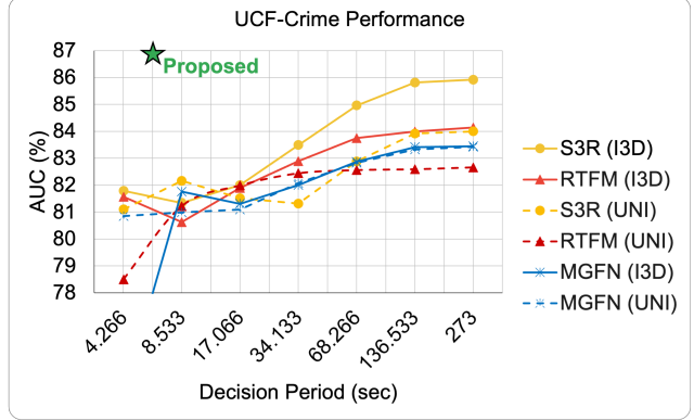
Figure 7. Performance drop of state-of-the-art methods with decreasing decision period on UCF-Crime. Proposed method (REWARD) provides a significantly improved real-time detection performance.
