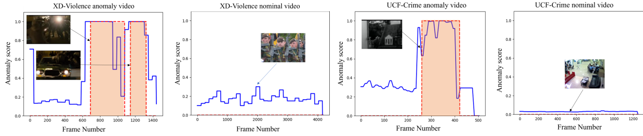
Figure 10. Anomaly score values of end-to-end trained REWARD based on Uniformer-32 on UCF-Crime and XD-Violence test videos. Light orange areas indicate the ground truth anomalous frames.
