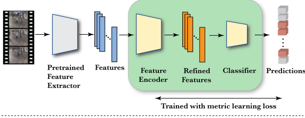
Proposed wVAD pipeline
