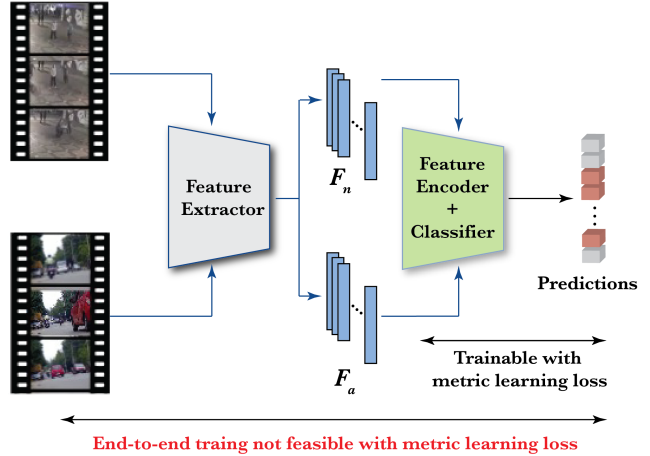
Figure 4. To train the feature encoder and classifier using a metric learning loss, F_n and F_a are processed together to promote the separability between normal and anomalous segments. Nevertheless, training a feature extractor end-to-end using a metric learning loss is not feasible due to two reasons: processing together large number of video clips in a single GPU entails huge memory requirements and feature extractor has orders of magnitude more parameters than feature encoder.
