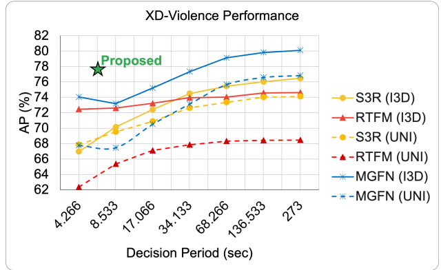
Figure 8. Performance drop of state-of-the-art methods with decreasing decision period on XD-Violence. Proposed method (REWARD) provides a significantly improved real-time detection performance.
