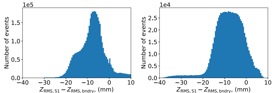
Fig. 10 Distribution of differences between position of ^{83\text{m}}\text{Kr} events as assigned using the linear correlation between \text{RMS}^2 as a function of z from S1 ( z_{\text{RMS,S1}} ) and as assigned purely referencing the cut-
