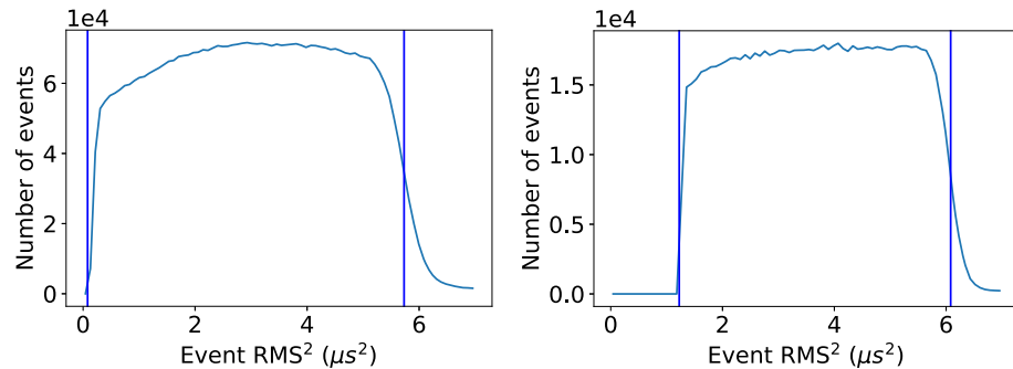
Fig. 9 Distribution of mean squared ( \text{RMS}^2 ) widths of ^{83\text{m}}\text{Kr} events, with boundary lines indicating corresponding minimum and maximum z values of the detector as determined from the distributions as described in the text. Left: NEXT-White data. Right: NEXT-100 simulation
