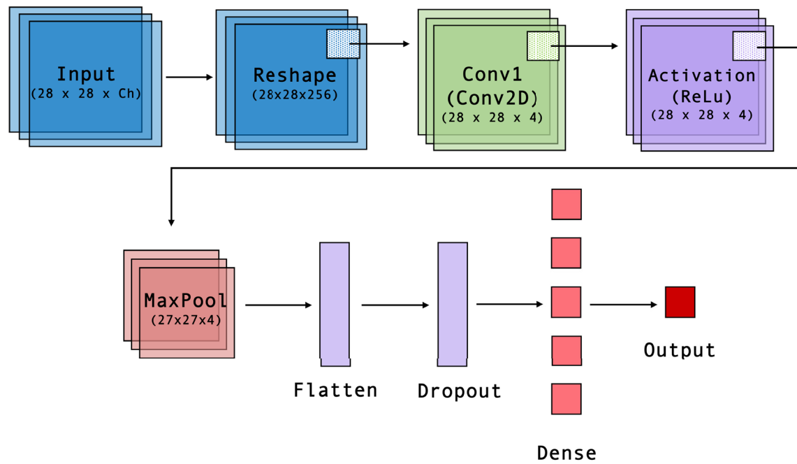
Fig. 11 Network architecture for XY plane configuration. For all three planes, XY , YZ , and XZ a sequential model is constructed. A permute layer is added to models YZ and XZ for dimensional order. Key features
