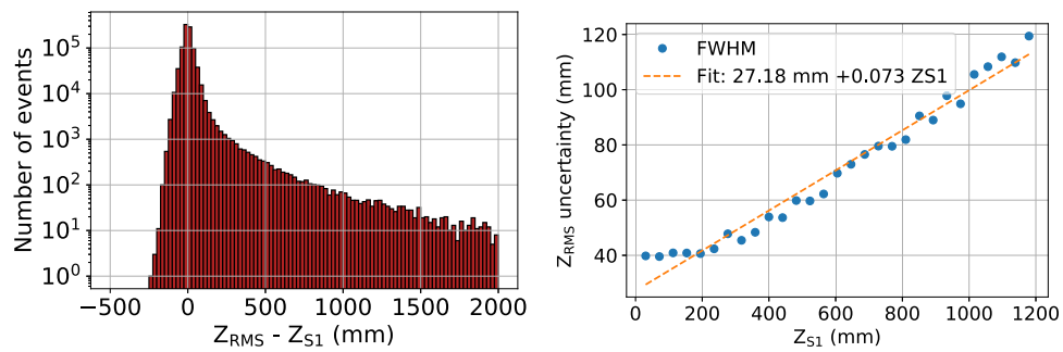
Fig. 8 NEXT-100 simulation. Left: Differences between z position determined by RMS ( z_{\text{RMS}} ) and determined from S1 ( z_{\text{S1}} ) for ^{83\text{m}}\text{Kr} events shown in log scale. Right: FWHM of z_{\text{RMS}} as a function of z_{\text{S1}} with a linear fit, understood as the increase in uncertainty of the z_{\text{RMS}} with z_{\text{S1}}
