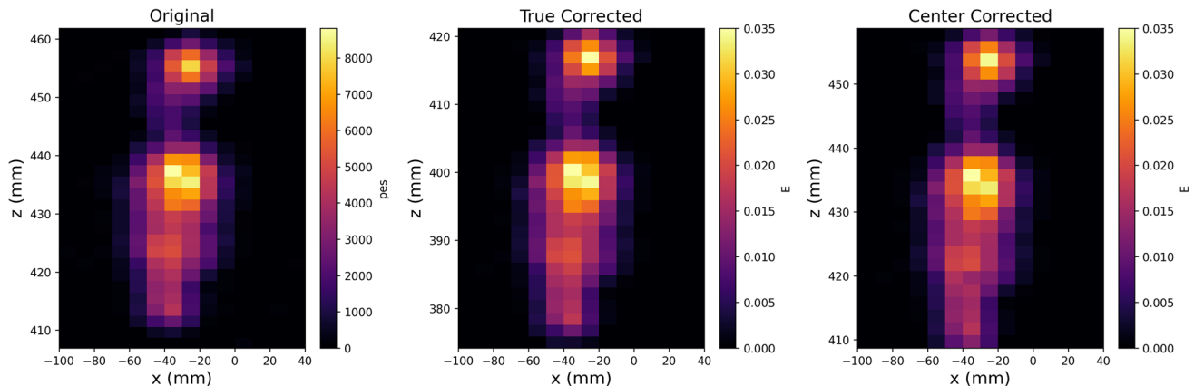
Fig. 12 Representation of the original uncalibrated event (left), the event after S1 calibration (middle), and the event post-diffusion calibration (right), projected onto the x - z plane. The effects of these corrections are notably rather small
