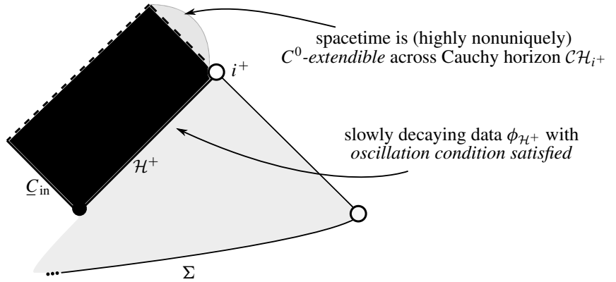
Figure 2. Theorem I(i) : if the strong qualitative oscillation condition is satisfied, then the spacetime is C^0 -extendible across the Cauchy horizon \mathcal{CH}_{i+} .
